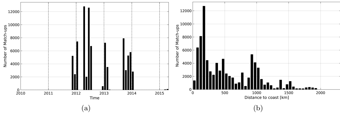
Figure 1: Number of match-ups between TSG-SAMOS and AQUARIUS-L2-JPL-V4 SSS as a function of time (a) and as function of the distance to coast (b) over the Tropical Atlantic Ocean Pi-MEP region and for the full satellite product period.
