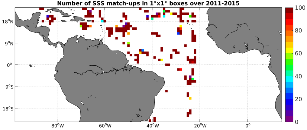
Figure 4: Number of SSS match-ups between TSG-SAMOS SSS and the AQUARIUS-L2-JPL-V4 SSS product for the Tropical Atlantic Ocean Pi-MEP region over 1^\circ \times 1^\circ boxes and for the full satellite product period.
