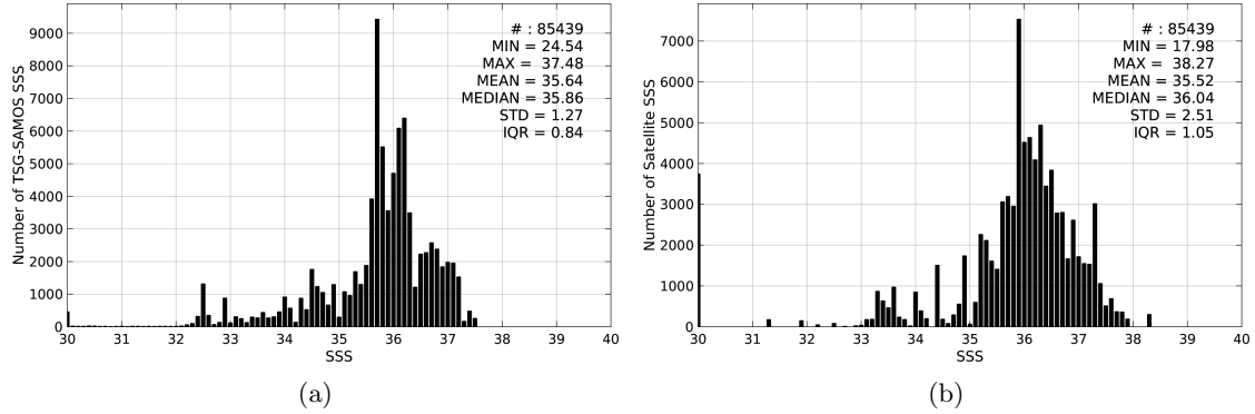
Figure 2: Histograms of SSS from TSG-SAMOS (a) and AQUARIUS-L2-JPL-V4 (b) considering all match-up pairs per bins of 0.1 over the Tropical Atlantic Ocean Pi-MEP region and for the full satellite product period.
