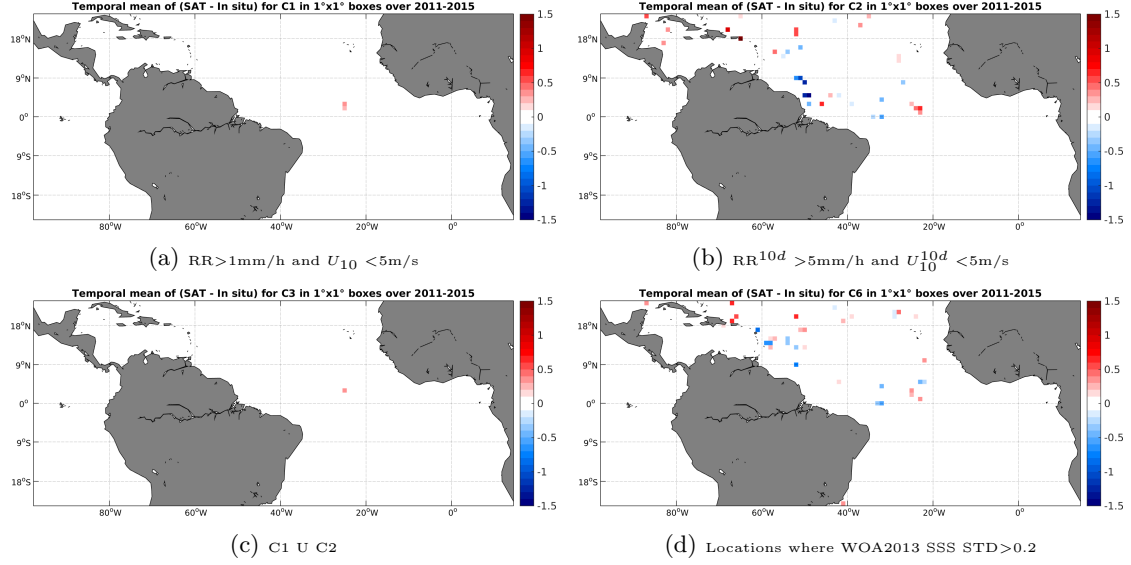
Figure 12: Temporal mean gridded over spatial boxes of size 1^\circ \times 1^\circ of \Delta SSS (AQUARIUS-L2-JPL-V4 - TSG-SAMOS) for 4 different subdatasets corresponding to: RR > 1mm/h and U_{10} < 5 m/s (a), RR^{10d} > 5 mm/h and U_{10}^{10d} < 5 m/s (b), C1 U C2 (c), Locations where WOA2013 SSS STD > 0.2 (d).
