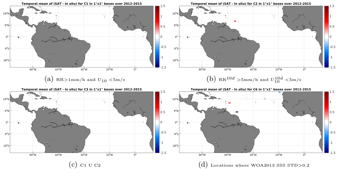
Figure 12: Temporal mean gridded over spatial boxes of size 1^\circ \times 1^\circ of \Delta SSS (AQUARIUS-L2-JPL-V4 - TSG-GOSUD-Sailing-ship) for 4 different subdatasets corresponding to:RR>1mm/h and U_{10} < 5\text{m/s} (a), RR^{10d} > 5\text{mm/h} and U_{10}^{10d} < 5\text{m/s} (b), C1 U C2 (c),Locations where WOA2013 SSS STD>0.2 (d).
