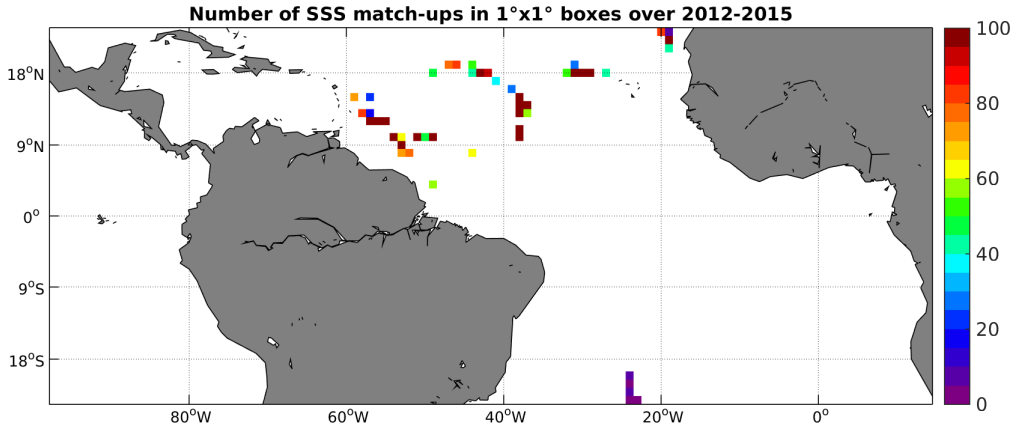
Figure 4: Number of SSS match-ups between TSG-GOSUD-Sailing-ship SSS and the AQUARIUS-L2-JPL-V4 SSS product for the Tropical Atlantic Ocean Pi-MEP region over 1^\circ \times 1^\circ boxes and for the full satellite product period.
