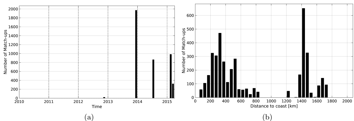
Figure 1: Number of match-ups between TSG-GOSUD-Sailing-ship and AQUARIUS-L2-JPL-V4 SSS as a function of time (a) and as function of the distance to coast (b) over the Tropical Atlantic Ocean Pi-MEP region and for the full satellite product period.
