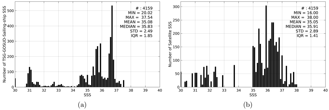
Figure 2: Histograms of SSS from TSG-GOSUD-Sailing-ship (a) and AQUARIUS-L2-JPL-V4 (b) considering all match-up pairs per bins of 0.1 over the Tropical Atlantic Ocean Pi-MEP region and for the full satellite product period.
