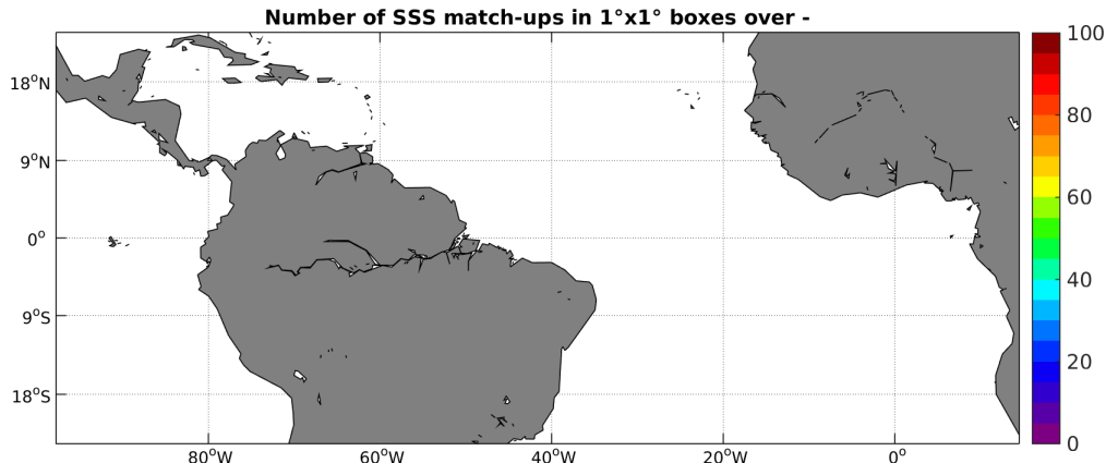
Figure 4: Number of SSS match-ups between Sea mammals SSS and the AQUARIUS-L2-JPL-V4 SSS product for the Tropical Atlantic Ocean Pi-MEP region over 1^\circ \times 1^\circ boxes and for the full satellite product period.
