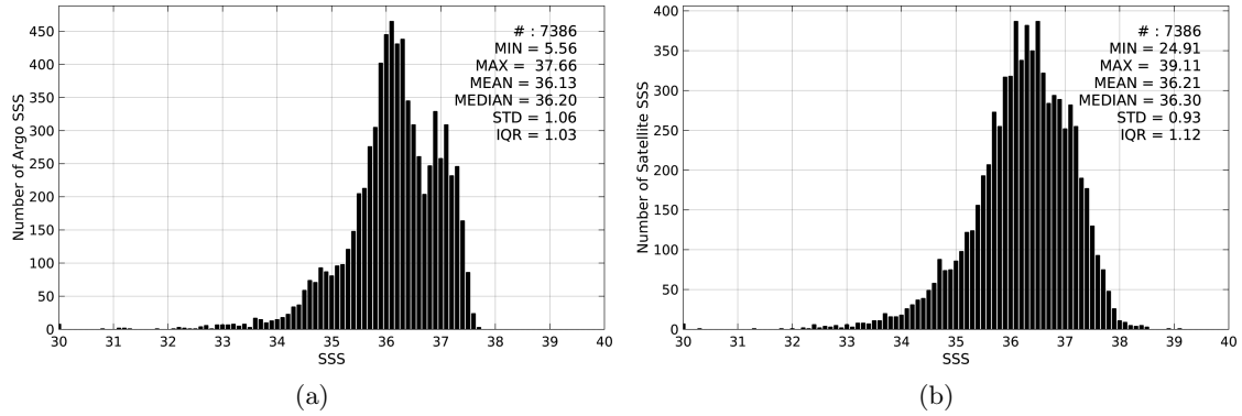
Figure 2: Histograms of SSS from Argo (a) and AQUARIUS-L2-JPL-V4 (b) considering all match-up pairs per bins of 0.1 over the Tropical Atlantic Ocean Pi-MEP region and for the full satellite product period.
