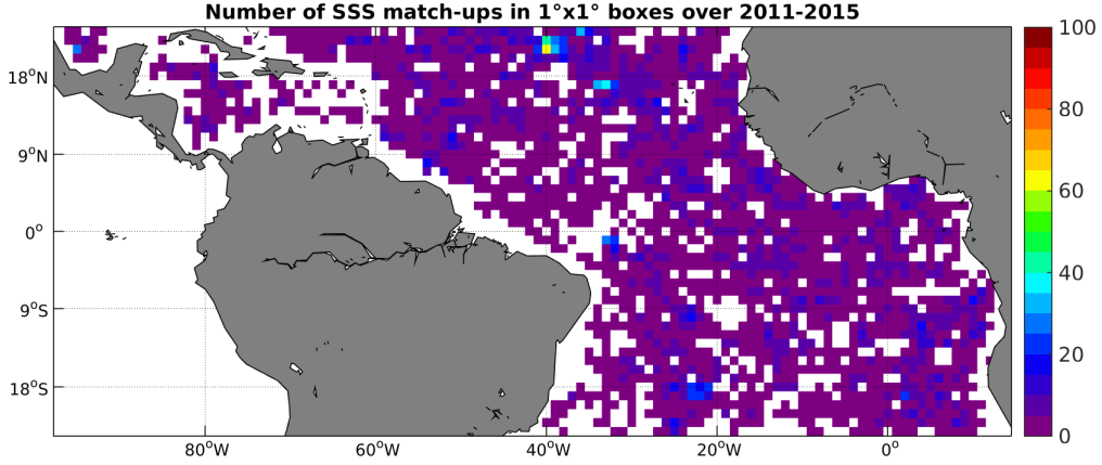
Figure 4: Number of SSS match-ups between Argo SSS and the AQUARIUS-L2-JPL-V4 SSS product for the Tropical Atlantic Ocean Pi-MEP region over 1^\circ \times 1^\circ boxes and for the full satellite product period.
