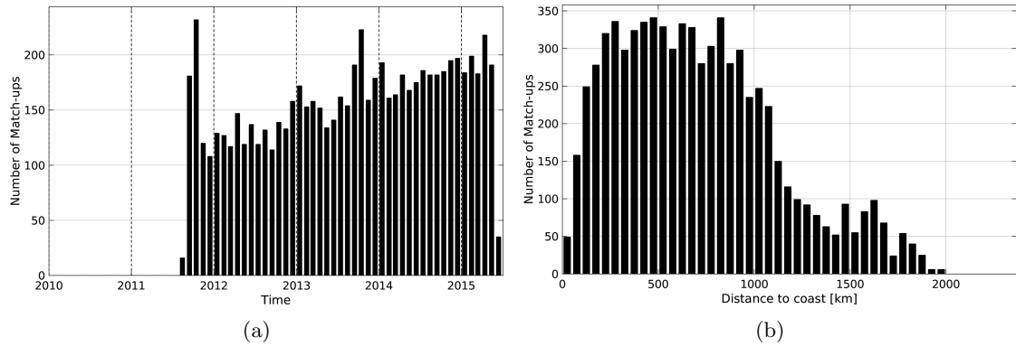
Figure 1: Number of match-ups between Argo and AQUARIUS-L2-JPL-V4 SSS as a function of time (a) and as function of the distance to coast (b) over the Tropical Atlantic Ocean Pi-MEP region and for the full satellite product period.
