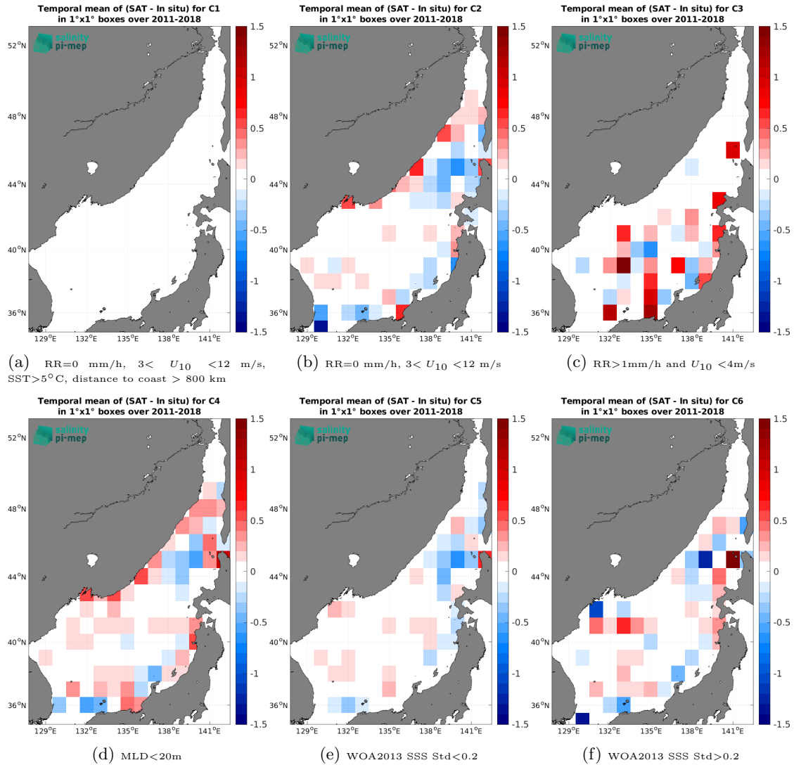
Figure 12: Temporal mean gridded over spatial boxes of size 1^\circ \times 1^\circ of \Delta SSS (SMOS and SMAP SSS L4 OI v1 - 7 Days (LOPS) - Argo) for 6 different subdatasets corresponding to: RR=0 mm/h, 3 < U_{10} < 12 m/s, SST > 5°C, distance to coast > 800 km (a), RR=0 mm/h, 3 < U_{10} < 12 m/s (b), RR > 1mm/h and U_{10} < 4 m/s (c), MLD < 20m (d), WOA2013 SSS Std < 0.2 (e), WOA2013 SSS Std > 0.2 (f).
