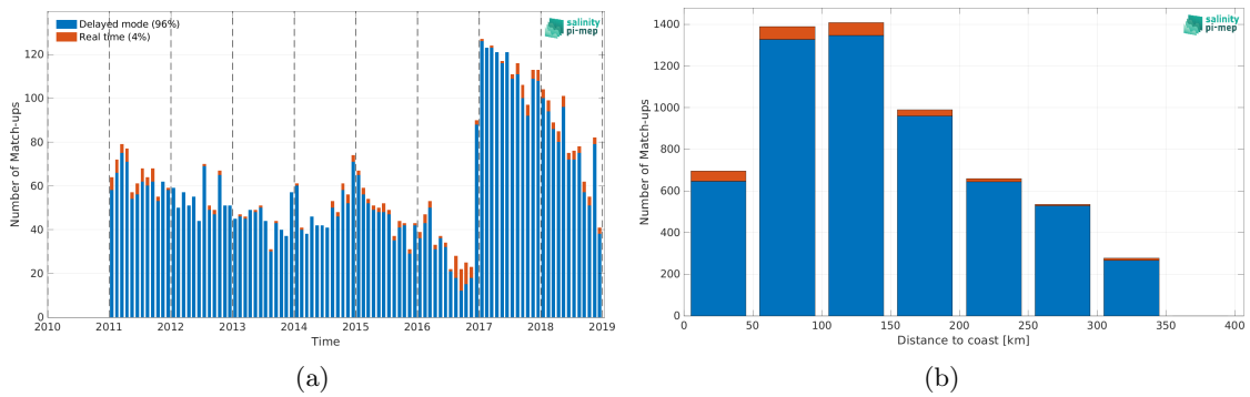
Figure 1: Number of match-ups between Argo and SMOS and SMAP SSS L4 OI v1 - 7 Days (LOPS) SSS as a function of time (a) and as function of the distance to coast (b) over the Sea of Japan Pi-MEP region and for the full satellite product period.
