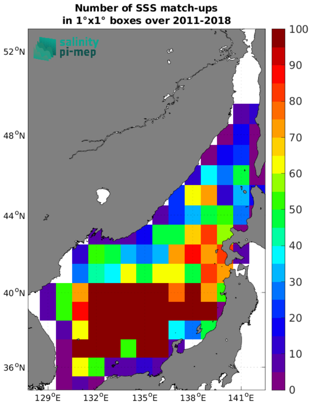
Figure 4: Number of SSS match-ups between Argo SSS and the SMOS and SMAP SSS L4 OI v1 - 7 Days (LOPS) SSS product for the Sea of Japan Pi-MEP region over 1°x1° boxes and for the full satellite product period.
