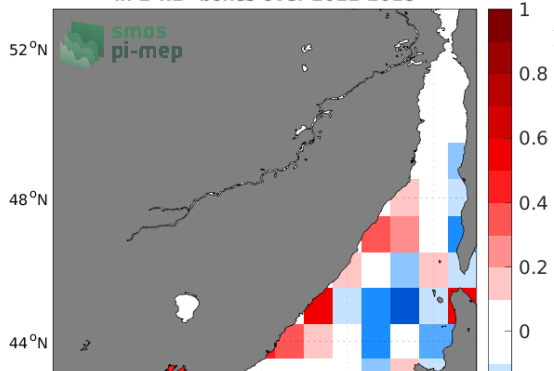
Temporal mean of (Sat - Argo) in 1°x1° boxes over 2011-2018
