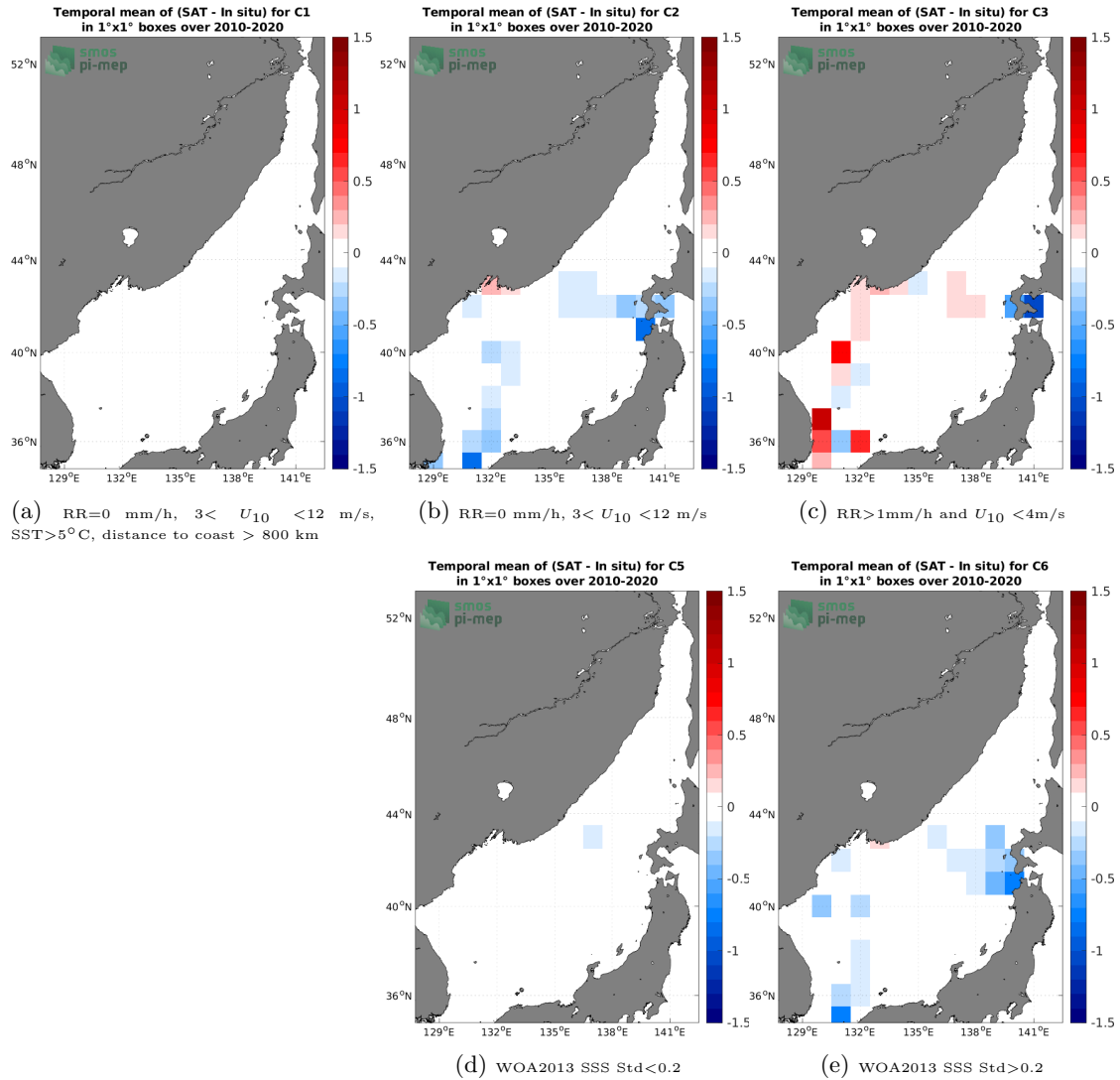
Figure 12: Temporal mean gridded over spatial boxes of size 1^\circ \times 1^\circ of \Delta SSS (SMOS SSS L4 v1 - Weekly (CMEMS-CNR) - TSG (LEGOS-DM)) for 5 different subdatasets corresponding to:RR=0 mm/h, 3 < U_{10} < 12 m/s, SST>5°C, distance to coast > 800 km (a), RR=0 mm/h, 3 < U_{10} < 12 m/s (b), RR>1mm/h and U_{10} < 4 m/s (c), WOA2013 SSS Std<0.2 (d), WOA2013 SSS Std>0.2 (e).
