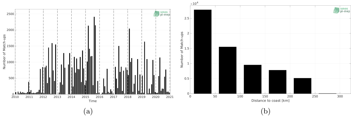
Figure 1: Number of match-ups between TSG (LEGOS-DM) and SMOS SSS L4 v1 - Weekly (CMEMS-CNR) SSS as a function of time (a) and as function of the distance to coast (b) over the Sea of Japan Pi-MEP region and for the full satellite product period.
