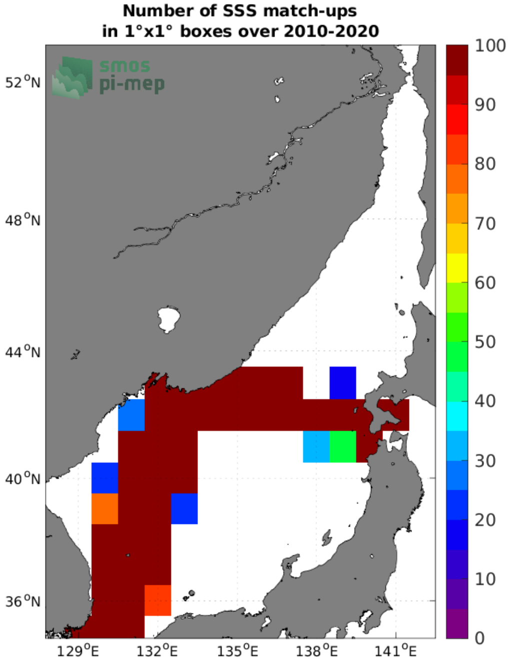
Figure 4: Number of SSS match-ups between TSG (LEGOS-DM) SSS and the SMOS SSS L4 v1 - Weekly (CMEMS-CNR) SSS product for the Sea of Japan Pi-MEP region over 1°x1° boxes and for the full satellite product period.
