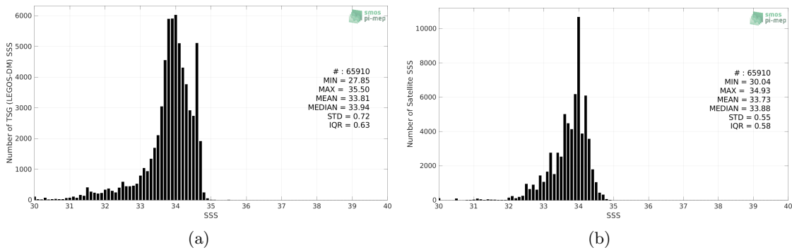
Figure 2: Histograms of SSS from TSG (LEGOS-DM) (a) and SMOS SSS L4 v1 - Weekly (CMEMS-CNR) (b) considering all match-up pairs per bins of 0.1 over the Sea of Japan Pi-MEP region and for the full satellite product period.
