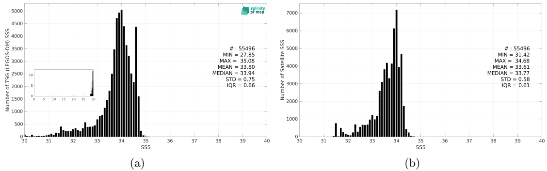
Figure 3: Histograms of SSS from TSG (LEGOS-DM) (a) and SMOS SSS L4 v1 - Monthly (CMEMS-CNR) (b) considering all match-up pairs per bins of 0.1 over the Sea of Japan Pi-MEP region and for the full satellite product period.
