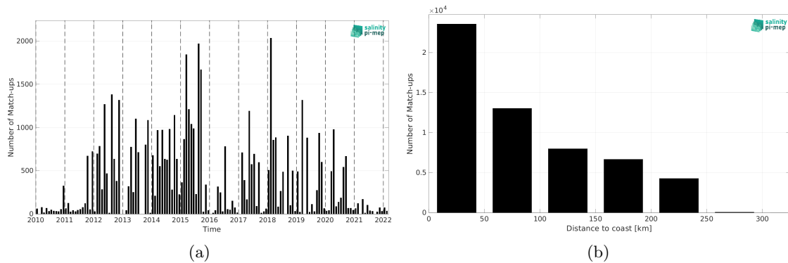
Figure 2: Number of match-ups between TSG (LEGOS-DM) and SMOS SSS L4 v1 - Monthly (CMEMS-CNR) SSS as a function of time (a) and as function of the distance to coast (b) over the Sea of Japan Pi-MEP region and for the full satellite product period.
