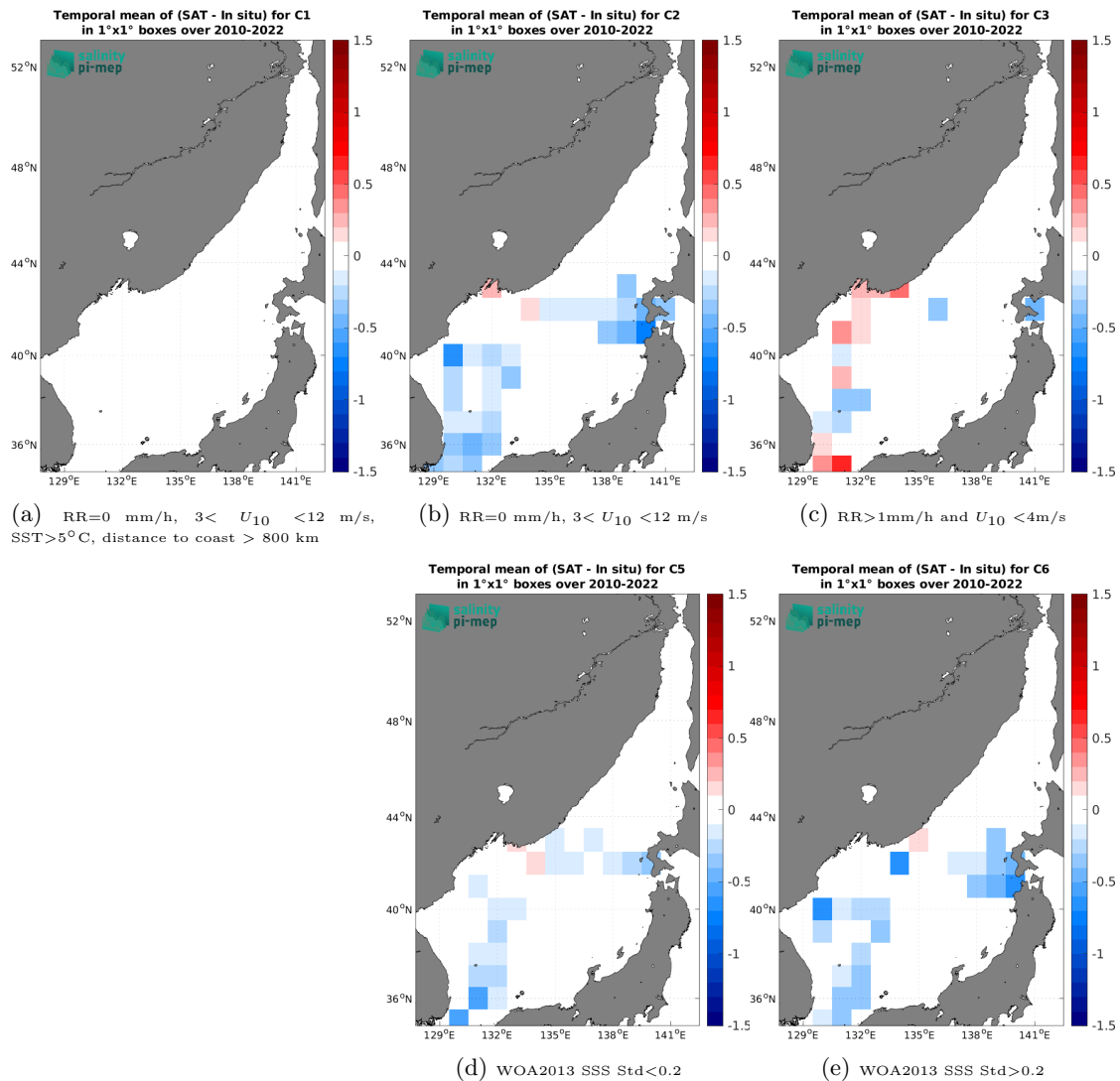
Figure 14: Temporal mean gridded over spatial boxes of size 1^\circ \times 1^\circ of \Delta SSS (SMOS SSS L4 v1 - Monthly (CMEMS-CNR) - TSG (LEGOS-DM)) for 5 different subdatasets corresponding to: RR=0 mm/h, 3 < U_{10} < 12 m/s, SST>5°C, distance to coast > 800 km (a), RR=0 mm/h, 3 < U_{10} < 12 m/s (b), RR>1mm/h and U_{10} < 4 m/s (c), WOA2013 SSS Std<0.2 (d), WOA2013 SSS Std>0.2 (e).
