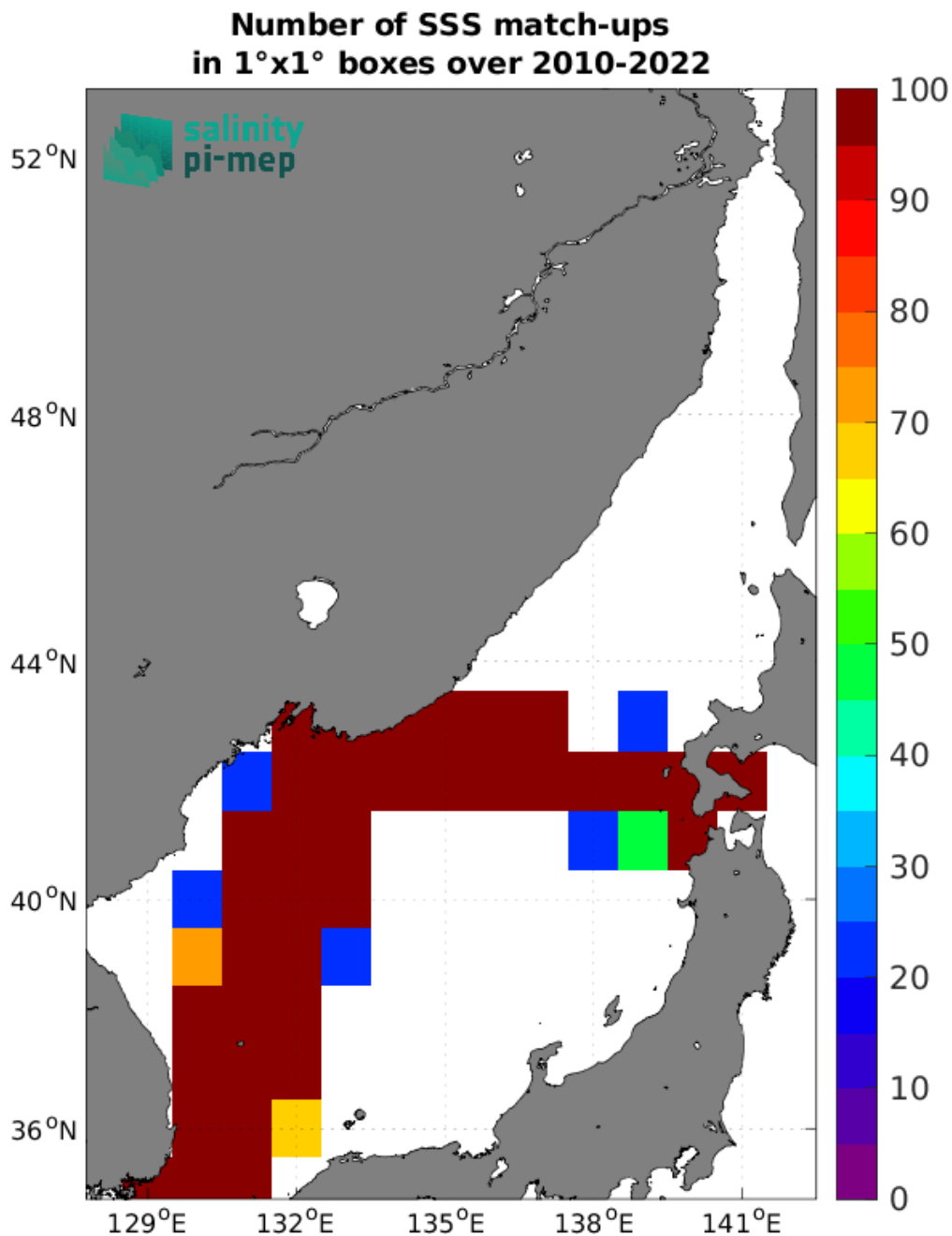
Figure 5: Number of SSS match-ups between TSG (LEGOS-DM) SSS and the SMOS SSS L4 v1 - Monthly (CMEMS-CNR) SSS product for the Sea of Japan Pi-MEP region over 1°x1° boxes and for the full satellite product period.
