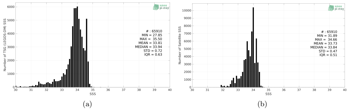
Figure 2: Histograms of SSS from TSG (LEGOS-DM) (a) and SMOS SSS L4 v1 - Monthly (CMEMS-CNR) (b) considering all match-up pairs per bins of 0.1 over the Sea of Japan Pi-MEP region and for the full satellite product period.
