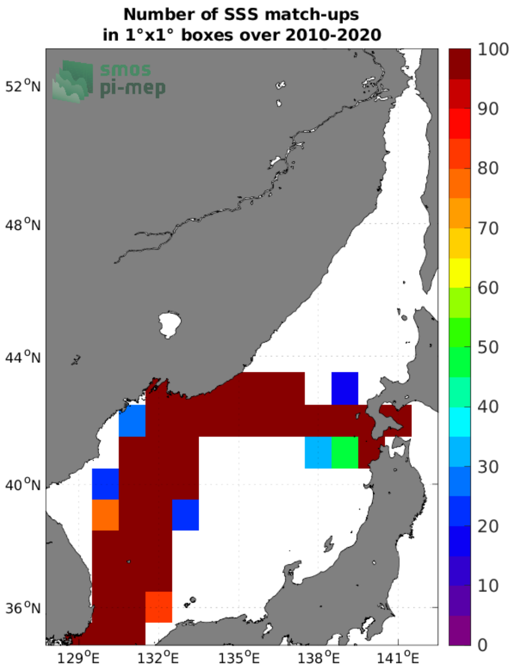
Figure 4: Number of SSS match-ups between TSG (LEGOS-DM) SSS and the SMOS SSS L4 v1 - Monthly (CMEMS-CNR) SSS product for the Sea of Japan Pi-MEP region over 1°x1° boxes and for the full satellite product period.
