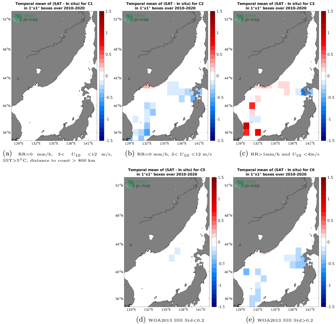
Figure 12: Temporal mean gridded over spatial boxes of size 1^\circ \times 1^\circ of \Delta SSS (SMOS SSS L4 v1 - Monthly (CMEMS-CNR) - TSG (LEGOS-DM)) for 5 different subdatasets corresponding to:RR=0 mm/h, 3 < U_{10} < 12 m/s, SST>5°C, distance to coast > 800 km (a), RR=0 mm/h, 3 < U_{10} < 12 m/s (b), RR>1mm/h and U_{10} < 4 m/s (c), WOA2013 SSS Std<0.2 (d), WOA2013 SSS Std>0.2 (e).
