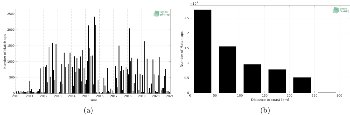
Figure 1: Number of match-ups between TSG (LEGOS-DM) and SMOS SSS L4 v1 - Monthly (CMEMS-CNR) SSS as a function of time (a) and as function of the distance to coast (b) over the Sea of Japan Pi-MEP region and for the full satellite product period.
