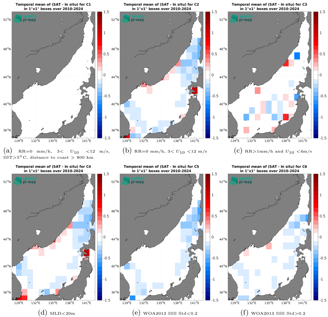
Figure 14: Temporal mean gridded over spatial boxes of size 1^\circ \times 1^\circ of \Delta\text{SSS} (SMOS SSS L4 v1 - Monthly (CMEMS-CNR) - Argo) for 6 different subdatasets corresponding to: RR=0 mm/h, 3 < U_{10} < 12 m/s, SST > 5^\circ\text{C} , distance to coast > 800 km (a), RR=0 mm/h, 3 < U_{10} < 12 m/s (b), RR > 1 mm/h and U_{10} < 4 m/s (c), MLD < 20 m (d), WOA2013 SSS Std < 0.2 (e), WOA2013 SSS Std > 0.2 (f).
