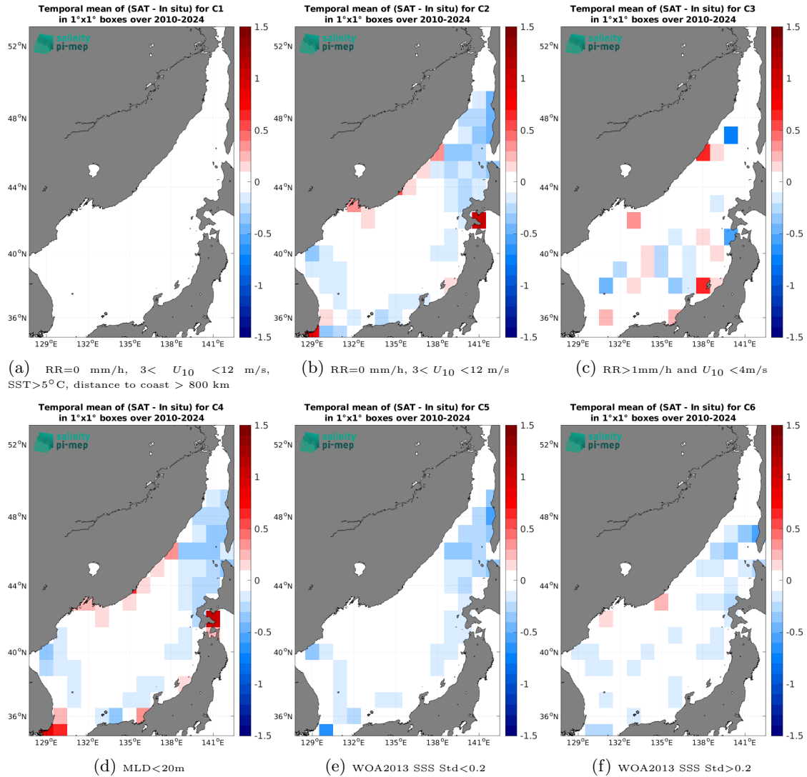
Figure 14: Temporal mean gridded over spatial boxes of size 1^\circ \times 1^\circ of \Delta SSS (SMOS SSS L4 v1 - Monthly (CMEMS-CNR) - Argo) for 6 different subdatasets corresponding to:RR=0 mm/h, 3 < U_{10} < 12 m/s, SST>5°C, distance to coast > 800 km (a), RR=0 mm/h, 3 < U_{10} < 12 m/s (b), RR>1mm/h and U_{10} < 4 m/s (c),MLD<20m (d),WOA2013 SSS Std<0.2 (e),WOA2013 SSS Std>0.2 (f).
