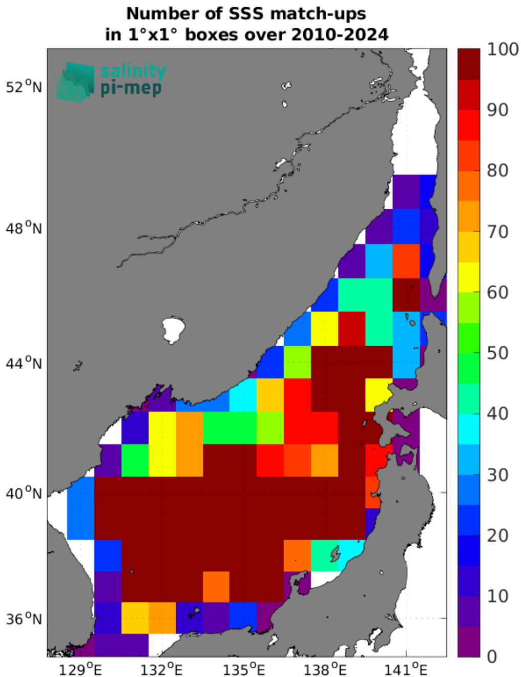
Figure 5: Number of SSS match-ups between Argo SSS and the SMOS SSS L4 v1 - Monthly (CMEMS-CNR) SSS product for the Sea of Japan Pi-MEP region over 1°x1° boxes and for the full satellite product period.
