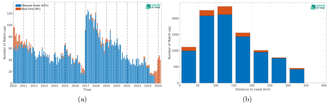
Figure 2: Number of match-ups between Argo and SMOS SSS L4 v1 - Monthly (CMEMS-CNR) SSS as a function of time (a) and as function of the distance to coast (b) over the Sea of Japan Pi-MEP region and for the full satellite product period.
