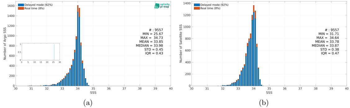
Figure 3: Histograms of SSS from Argo (a) and SMOS SSS L4 v1 - Monthly (CMEMS-CNR) (b) considering all match-up pairs per bins of 0.1 over the Sea of Japan Pi-MEP region and for the full satellite product period.
