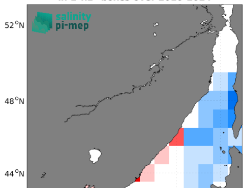
(c) MEAN(Argo SSS)
