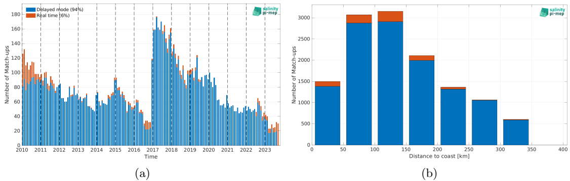
Figure 1: Number of match-ups between Argo and SMOS SSS L4 v1 - Monthly (CMEMS-CNR) SSS as a function of time (a) and as function of the distance to coast (b) over the Sea of Japan Pi-MEP region and for the full satellite product period.
