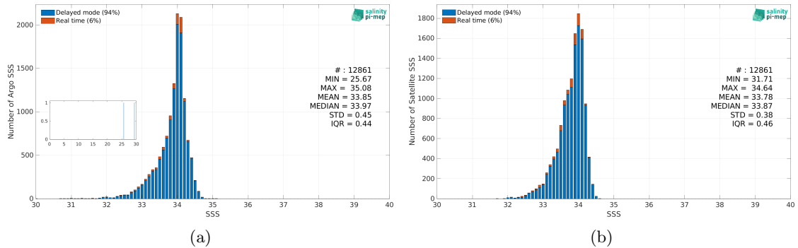
Figure 2: Histograms of SSS from Argo (a) and SMOS SSS L4 v1 - Monthly (CMEMS-CNR) (b) considering all match-up pairs per bins of 0.1 over the Sea of Japan Pi-MEP region and for the full satellite product period.
