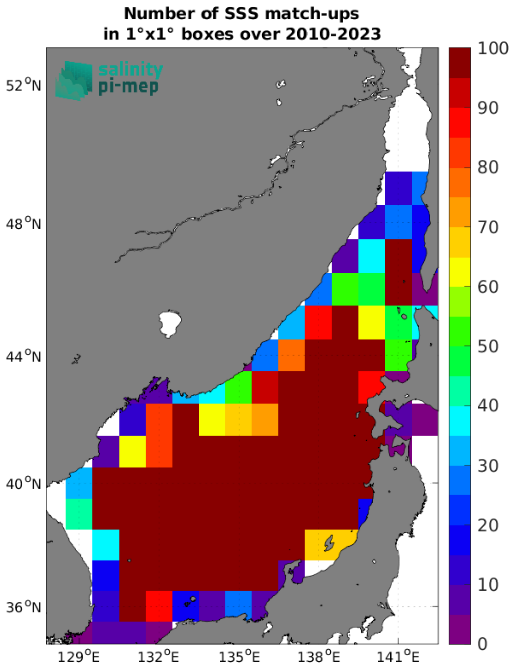
Figure 4: Number of SSS match-ups between Argo SSS and the SMOS SSS L4 v1 - Monthly (CMEMS-CNR) SSS product for the Sea of Japan Pi-MEP region over 1°x1° boxes and for the full satellite product period.
