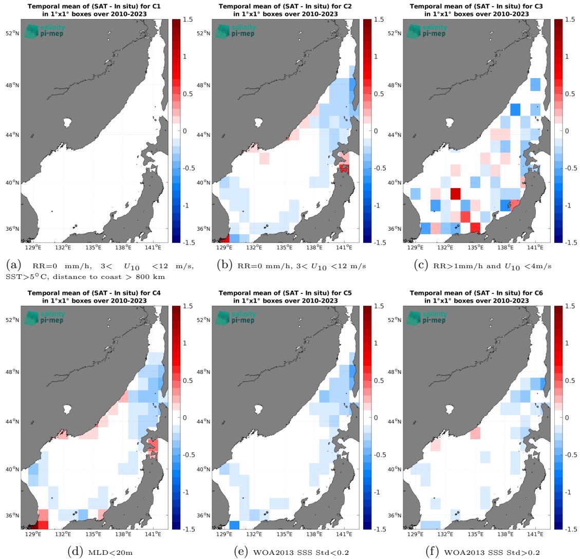
Figure 12: Temporal mean gridded over spatial boxes of size 1^\circ \times 1^\circ of \Delta SSS (SMOS SSS L4 v1 - Monthly (CMEMS-CNR) - Argo) for 6 different subdatasets corresponding to:RR=0 mm/h, 3 < U_{10} < 12 m/s, SST>5°C, distance to coast > 800 km (a), RR=0 mm/h, 3 < U_{10} < 12 m/s (b), RR>1mm/h and U_{10} < 4 m/s (c),MLD<20m (d),WOA2013 SSS Std<0.2 (e),WOA2013 SSS Std>0.2 (f).
