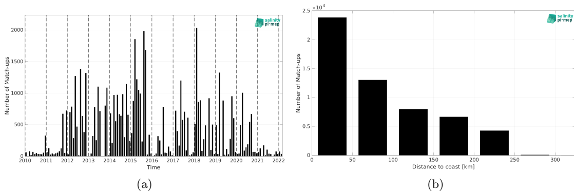
Figure 2: Number of match-ups between TSG (LEGOS-DM) and SMOS SSS L4 v1 - Daily (CMEMS-CNR) SSS as a function of time (a) and as function of the distance to coast (b) over the Sea of Japan Pi-MEP region and for the full satellite product period.
