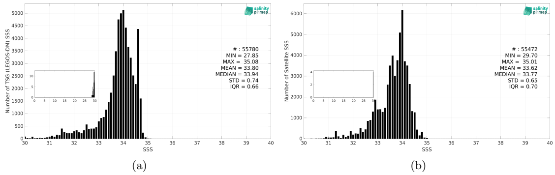
Figure 3: Histograms of SSS from TSG (LEGOS-DM) (a) and SMOS SSS L4 v1 - Daily (CMEMS-CNR) (b) considering all match-up pairs per bins of 0.1 over the Sea of Japan Pi-MEP region and for the full satellite product period.
