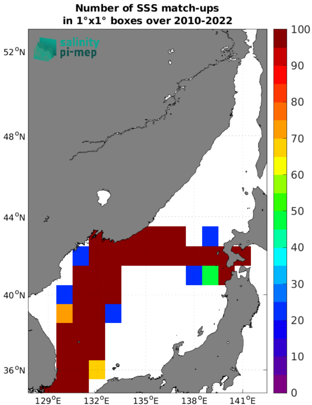
Figure 5: Number of SSS match-ups between TSG (LEGOS-DM) SSS and the SMOS SSS L4 v1 - Daily (CMEMS-CNR) SSS product for the Sea of Japan Pi-MEP region over 1°x1° boxes and for the full satellite product period.
