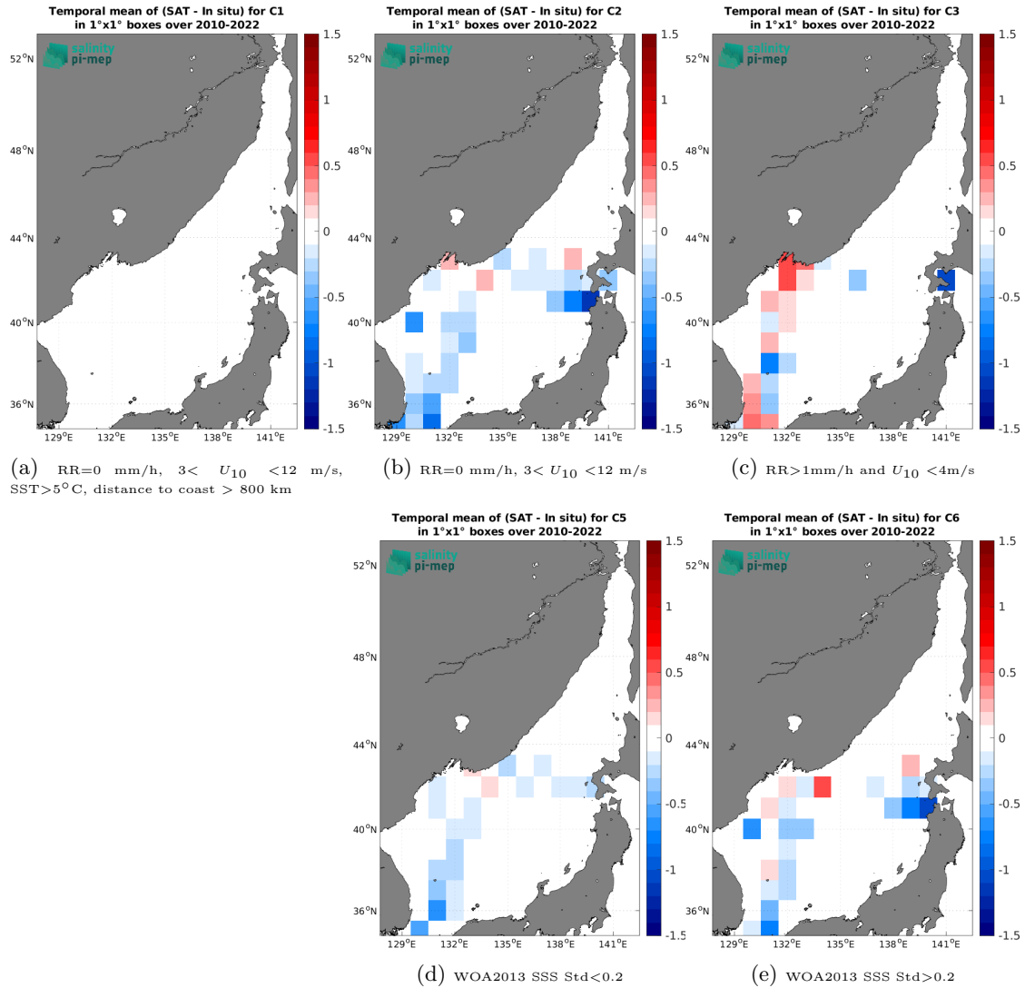
Figure 14: Temporal mean gridded over spatial boxes of size 1^\circ \times 1^\circ of \Delta SSS (SMOS SSS L4 v1 - Daily (CMEMS-CNR) - TSG (LEGOS-DM)) for 5 different subdatasets corresponding to:RR=0 mm/h, 3 < U_{10} < 12 m/s, SST>5°C, distance to coast > 800 km (a), RR=0 mm/h, 3 < U_{10} < 12 m/s (b), RR>1mm/h and U_{10} < 4 m/s (c), WOA2013 SSS Std<0.2 (d), WOA2013 SSS Std>0.2 (e).
