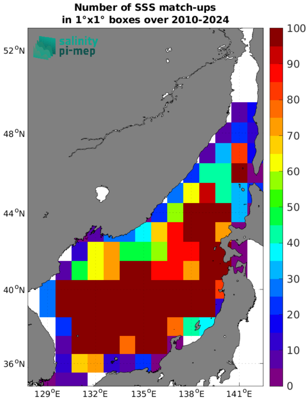
Figure 5: Number of SSS match-ups between Argo SSS and the SMOS SSS L4 v1 - Daily (CMEMS-CNR) SSS product for the Sea of Japan Pi-MEP region over 1°x1° boxes and for the full satellite product period.
