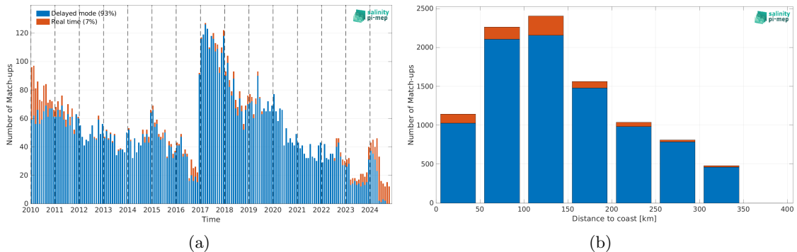
Figure 2: Number of match-ups between Argo and SMOS SSS L4 v1 - Daily (CMEMS-CNR) SSS as a function of time (a) and as function of the distance to coast (b) over the Sea of Japan Pi-MEP region and for the full satellite product period.
