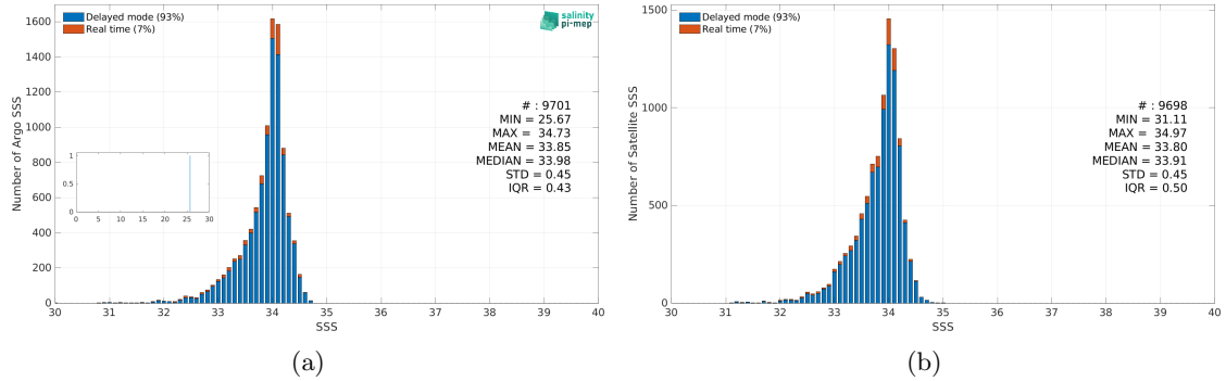
Figure 3: Histograms of SSS from Argo (a) and SMOS SSS L4 v1 - Daily (CMEMS-CNR) (b) considering all match-up pairs per bins of 0.1 over the Sea of Japan Pi-MEP region and for the full satellite product period.
