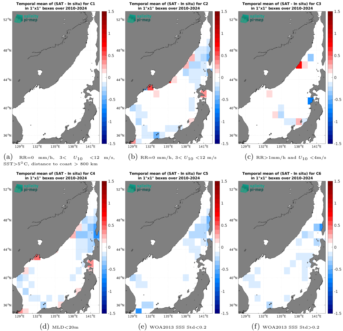
Figure 14: Temporal mean gridded over spatial boxes of size 1^\circ \times 1^\circ of \Delta SSS (SMOS SSS L4 v1 - Daily (CMEMS-CNR) - Argo) for 6 different subdatasets corresponding to: RR=0 mm/h, 3 < U_{10} < 12 m/s, SST > 5°C, distance to coast > 800 km (a), RR=0 mm/h, 3 < U_{10} < 12 m/s (b), RR > 1mm/h and U_{10} < 4 m/s (c), MLD < 20m (d), WOA2013 SSS Std < 0.2 (e), WOA2013 SSS Std > 0.2 (f).
