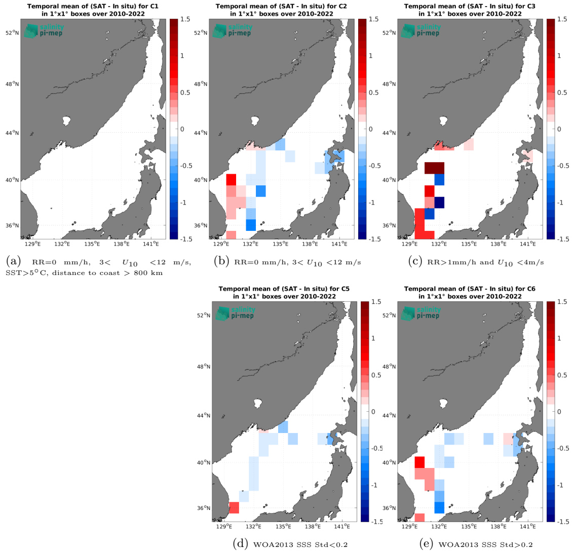
Figure 14: Temporal mean gridded over spatial boxes of size 1^\circ \times 1^\circ of \Delta SSS (SMOS SSS L4 OI v346 - Weekly (CMEMS-CATDS-LOPS) - TSG (LEGOS-DM)) for 5 different subdatasets corresponding to: RR=0 mm/h, 3 < U_{10} < 12 m/s, SST>5°C, distance to coast > 800 km (a), RR=0 mm/h, 3 < U_{10} < 12 m/s (b), RR>1mm/h and U_{10} < 4 m/s (c), WOA2013 SSS Std<0.2 (d), WOA2013 SSS Std>0.2 (e).
