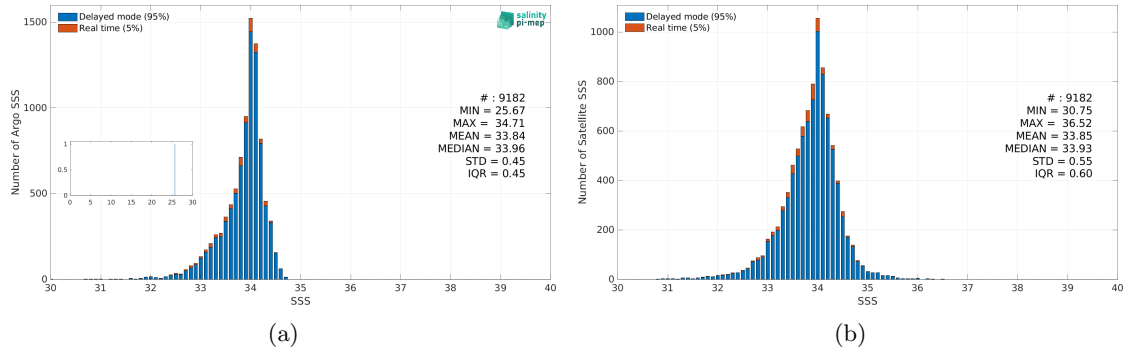
Figure 3: Histograms of SSS from Argo (a) and SMOS SSS L4 OI v346 - Weekly (CMEMS-CATDS-LOPS) (b) considering all match-up pairs per bins of 0.1 over the Sea of Japan Pi-MEP region and for the full satellite product period.
