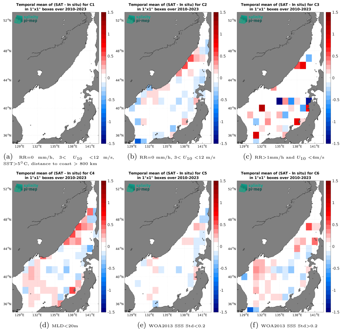
Figure 14: Temporal mean gridded over spatial boxes of size 1^\circ \times 1^\circ of \Delta SSS (SMOS SSS L4 OI v346 - Weekly (CMEMS-CATDS-LOPS) - Argo) for 6 different subdatasets corresponding to: RR=0 mm/h, 3 < U_{10} < 12 m/s, SST > 5°C, distance to coast > 800 km (a), RR=0 mm/h, 3 < U_{10} < 12 m/s (b), RR > 1mm/h and U_{10} < 4 m/s (c), MLD < 20m (d), WOA2013 SSS Std < 0.2 (e), WOA2013 SSS Std > 0.2 (f).
