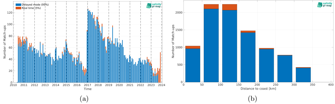
Figure 2: Number of match-ups between Argo and SMOS SSS L4 OI v346 - Weekly (CMEMS-CATDS-LOPS) SSS as a function of time (a) and as function of the distance to coast (b) over the Sea of Japan Pi-MEP region and for the full satellite product period.
