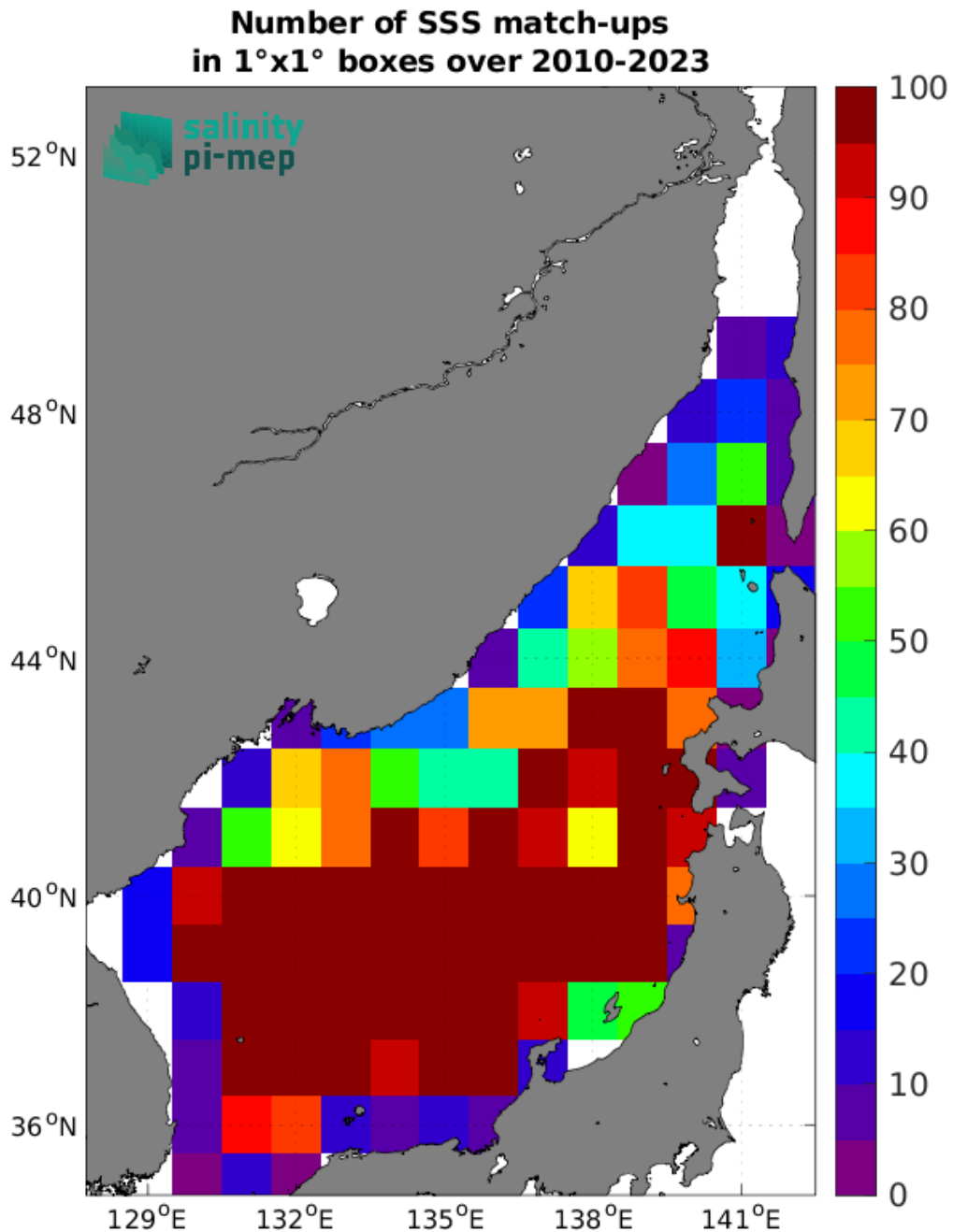
Figure 5: Number of SSS match-ups between Argo SSS and the SMOS SSS L4 OI v346 - Weekly (CMEMS-CATDS-LOPS) SSS product for the Sea of Japan Pi-MEP region over 1°x1° boxes and for the full satellite product period.
