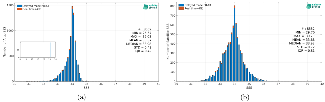
Figure 2: Histograms of SSS from Argo (a) and SMOS SSS L4 OI v342 - Weekly (CMEMS-CATDS-LOPS) (b) considering all match-up pairs per bins of 0.1 over the Sea of Japan Pi-MEP region and for the full satellite product period.
