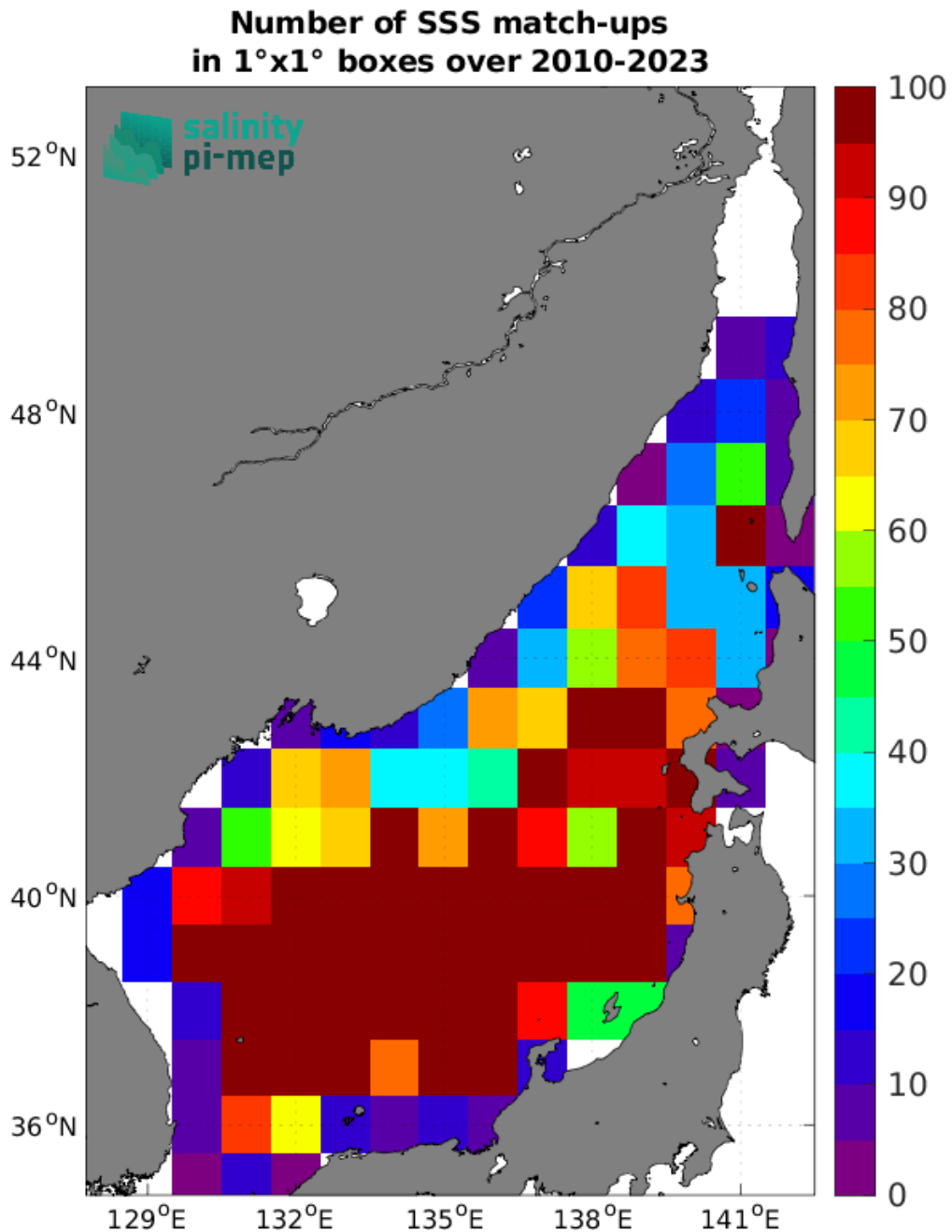
Figure 4: Number of SSS match-ups between Argo SSS and the SMOS SSS L4 OI v342 - Weekly (CMEMS-CATDS-LOPS) SSS product for the Sea of Japan Pi-MEP region over 1°x1° boxes and for the full satellite product period.
