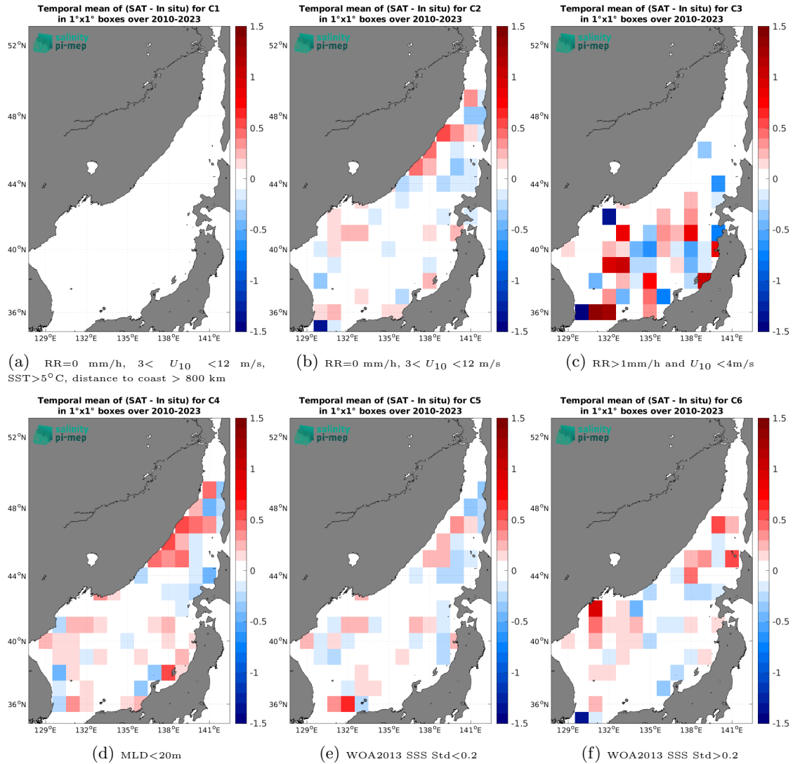
Figure 12: Temporal mean gridded over spatial boxes of size 1^\circ \times 1^\circ of \Delta SSS (SMOS SSS L4 OI v342 - Weekly (CMEMS-CATDS-LOPS) - Argo) for 6 different subdatasets corresponding to: RR=0 mm/h, 3 < U_{10} < 12 m/s, SST > 5°C, distance to coast > 800 km (a), RR=0 mm/h, 3 < U_{10} < 12 m/s (b), RR > 1mm/h and U_{10} < 4 m/s (c), MLD < 20m (d), WOA2013 SSS Std < 0.2 (e), WOA2013 SSS Std > 0.2 (f).
