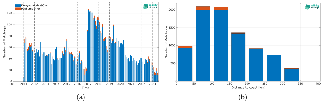
Figure 1: Number of match-ups between Argo and SMOS SSS L4 OI v342 - Weekly (CMEMS-CATDS-LOPS) SSS as a function of time (a) and as function of the distance to coast (b) over the Sea of Japan Pi-MEP region and for the full satellite product period.
