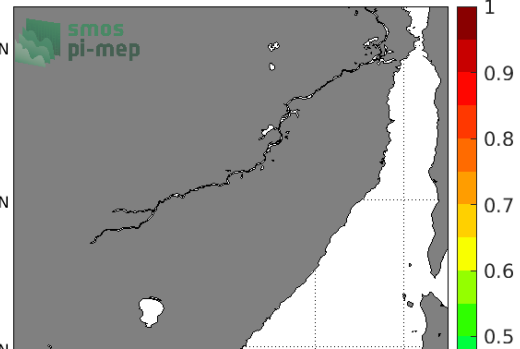
Temporal STD of (Sat - TSG (LEGOS-DM)) in 1°x1° boxes over 2015-2017
