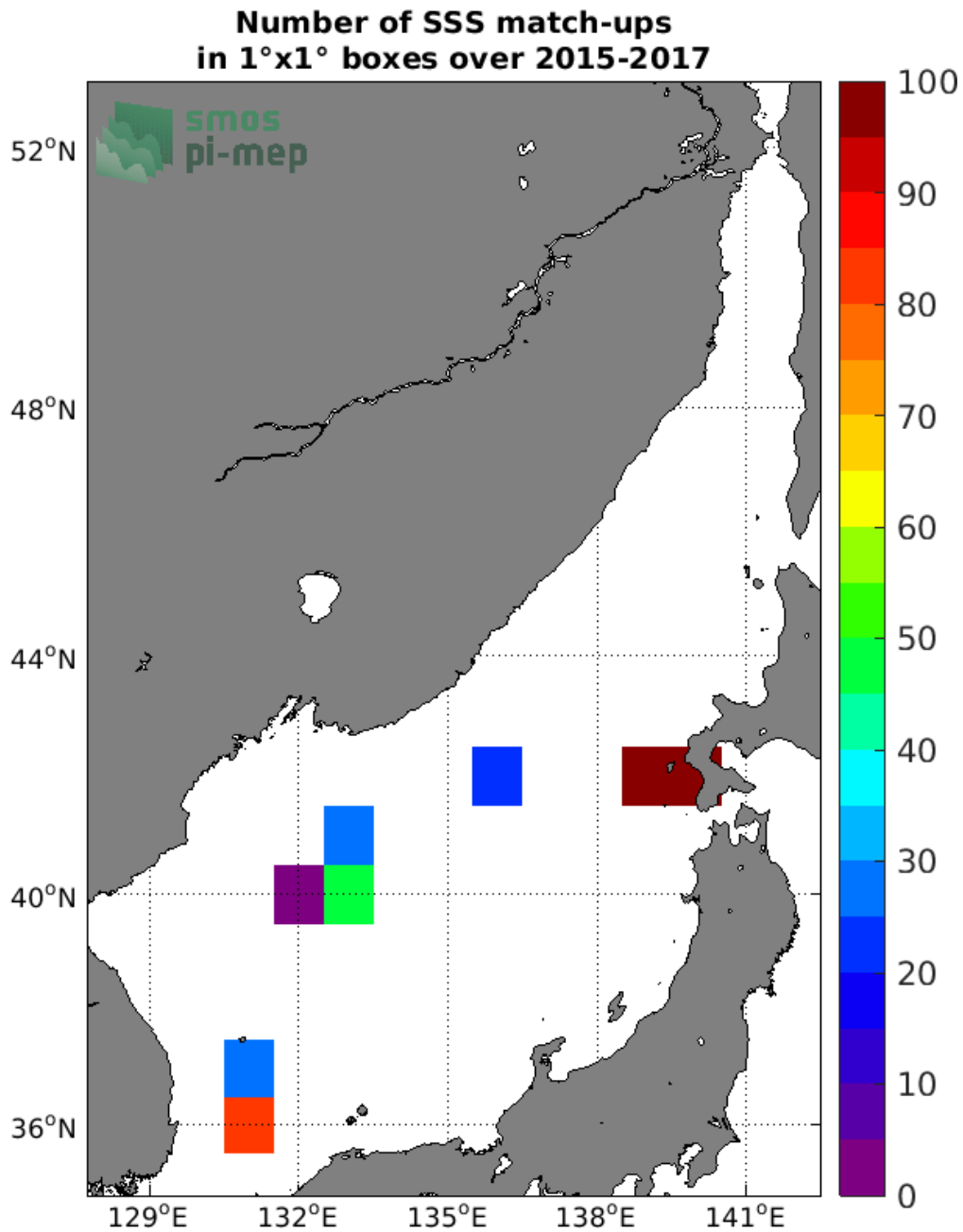
Figure 4: Number of SSS match-ups between TSG (LEGOS-DM) SSS and the SMOS L4 v2 Weekly (CATDS-CECOS-IFREMER) SSS product for the Sea of Japan Pi-MEP region over 1°x1° boxes and for the full satellite product period.
