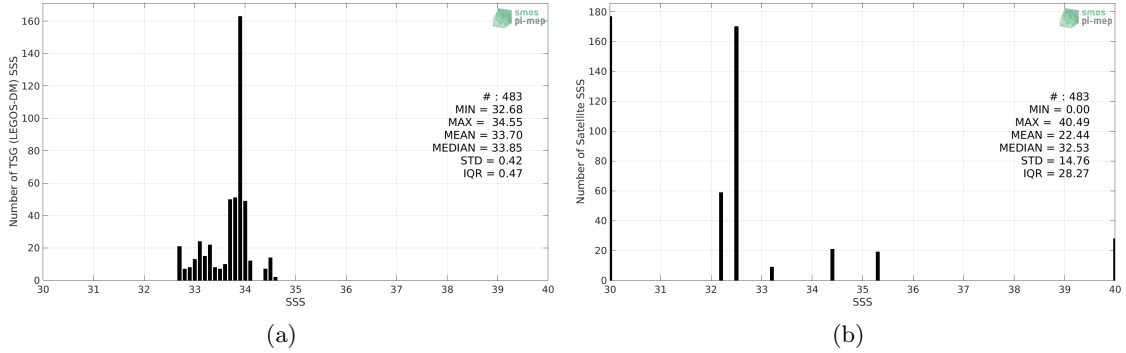
Figure 2: Histograms of SSS from TSG (LEGOS-DM) (a) and SMOS L4 v2 Weekly (CATDS-CECOS-IFREMER) (b) considering all match-up pairs per bins of 0.1 over the Sea of Japan Pi-MEP region and for the full satellite product period.
