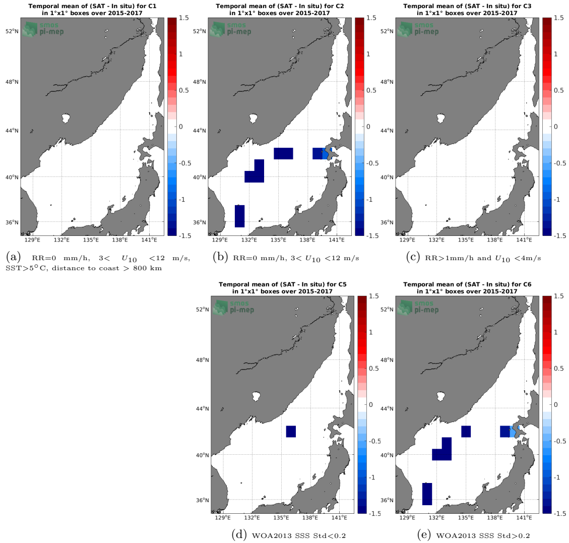
Figure 12: Temporal mean gridded over spatial boxes of size 1°x1° of \Delta SSS (SMOS L4 v2 Weekly (CATDS-CECOS-IFREMER) - TSG (LEGOS-DM)) for 5 different subdatasets corresponding to:RR=0 mm/h, 3 < U_{10} < 12 m/s, SST>5°C, distance to coast > 800 km (a), RR=0 mm/h, 3 < U_{10} < 12 m/s (b), RR>1mm/h and U_{10} < 4 m/s (c), WOA2013 SSS Std<0.2 (d), WOA2013 SSS Std>0.2 (e).
