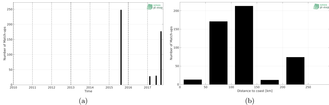
Figure 1: Number of match-ups between TSG (LEGOS-DM) and SMOS L4 v2 Weekly (CATDS-CECOS-IFREMER) SSS as a function of time (a) and as function of the distance to coast (b) over the Sea of Japan Pi-MEP region and for the full satellite product period.
