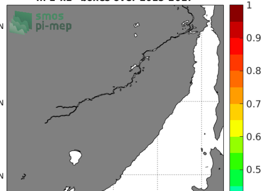
Temporal STD of (Sat - TSG-LEGOS-DM) in 1°x1° boxes over 2015-2017
