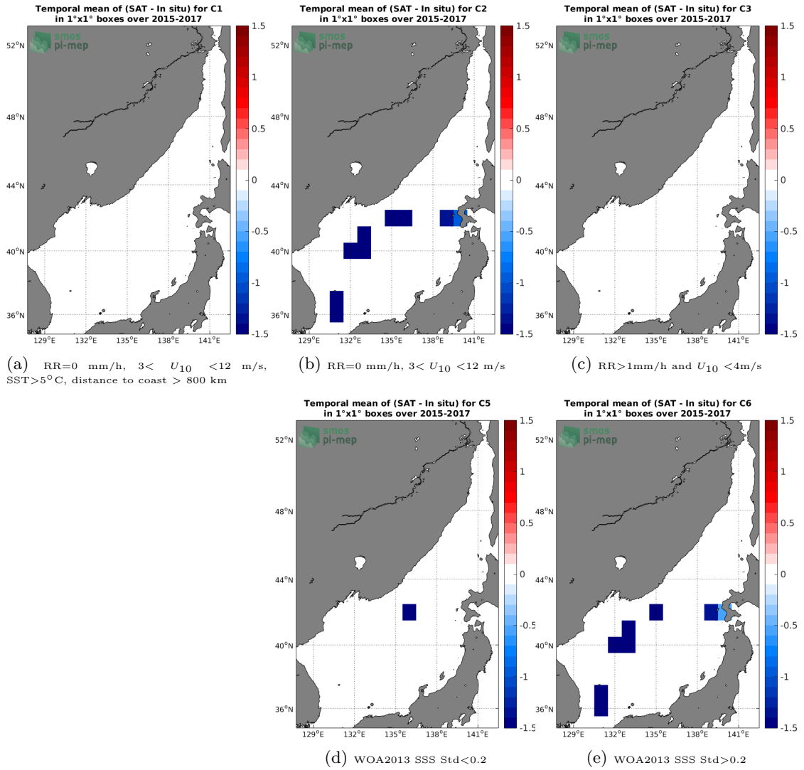
Figure 12: Temporal mean gridded over spatial boxes of size 1°x1° of \Delta\text{SSS} (SMOS-L4-CATDS-CECOS-IFREMER-V2-WEEKLY-0.5DEG - TSG-LEGOS-DM) for 5 different subdatasets corresponding to: RR=0 mm/h, 3 < U_{10} < 12 m/s, SST > 5^\circ\text{C} , distance to coast > 800 km (a), RR=0 mm/h, 3 < U_{10} < 12 m/s (b), RR > 1 mm/h and U_{10} < 4 m/s (c), WOA2013 SSS Std < 0.2 (d), WOA2013 SSS Std > 0.2 (e).
