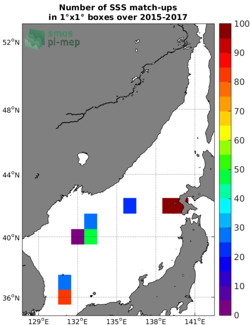
Figure 4: Number of SSS match-ups between TSG-LEGOS-DM SSS and the SMOS-L4-CATDS-CECOS-IFREMER-V2-WEEKLY-0.5DEG SSS product for the Sea of Japan Pi-MEP region over 1°x1° boxes and for the full satellite product period.
