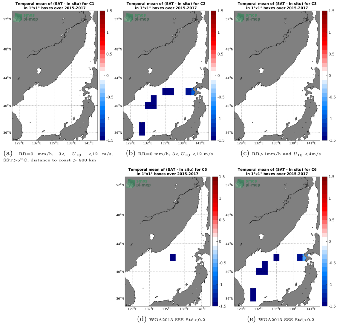
Figure 12: Temporal mean gridded over spatial boxes of size 1°x1° of \Delta SSS (SMOS-L4-CATDS-CECOS-IFREMER-V2-WEEKLY-0.5DEG - TSG-LEGOS-DM) for 5 different subdatasets corresponding to:RR=0 mm/h, 3 < U_{10} < 12 m/s, SST>5°C, distance to coast > 800 km (a), RR=0 mm/h, 3 < U_{10} < 12 m/s (b), RR>1mm/h and U_{10} < 4 m/s (c), WOA2013 SSS Std<0.2 (d), WOA2013 SSS Std>0.2 (e).
