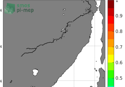
Temporal STD of (Sat - TSG-LEGOS-DM) in 1°x1° boxes over 2015-2017
