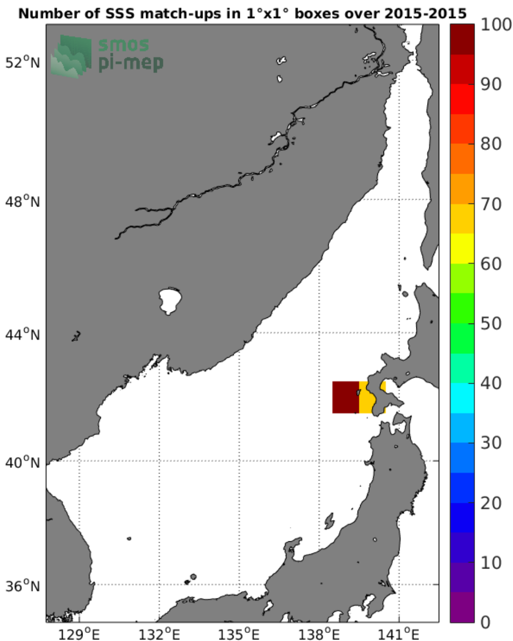
Figure 4: Number of SSS match-ups between TSG-LEGOS-DM SSS and the SMOS-L4-CATDS-CECOS-IFREMER-V2-WEEKLY-0.5DEG SSS product for the Sea of Japan Pi-MEP region over 1°x1° boxes and for the full satellite product period.
