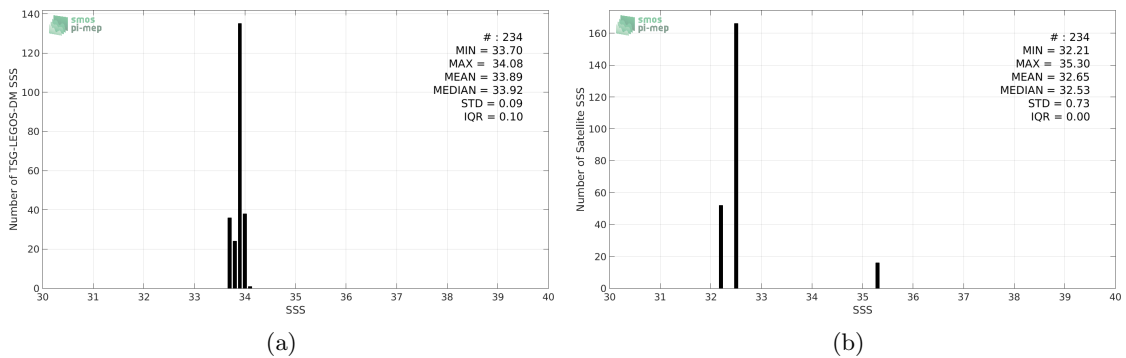
Figure 2: Histograms of SSS from TSG-LEGOS-DM (a) and SMOS-L4-CATDS-CECOS-IFREMER-V2-WEEKLY-0.5DEG (b) considering all match-up pairs per bins of 0.1 over the Sea of Japan Pi-MEP region and for the full satellite product period.
