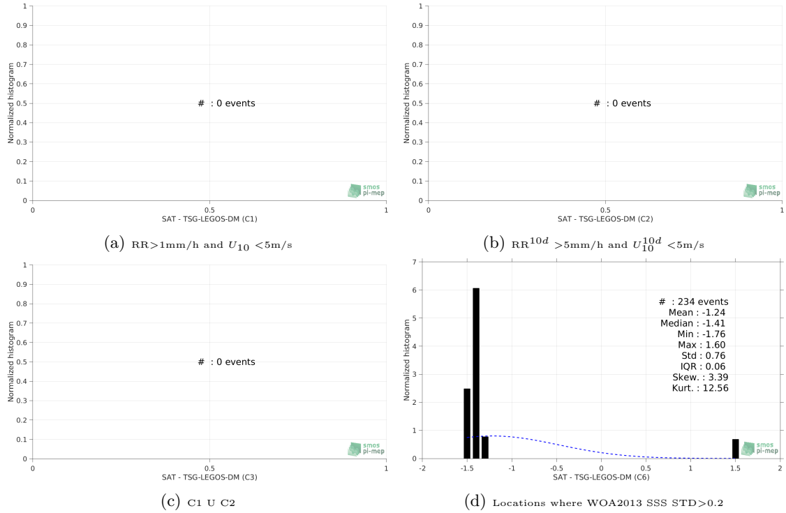
Figure 13: Normalized histogram of \Delta\text{SSS} (SMOS-L4-CATDS-CECOS-IFREMER-V2-WEEKLY-0.5DEG - TSG-LEGOS-DM) for 6 different subdatasets corresponding to: RR > 1\text{mm/h} and U_{10} < 5\text{m/s} (a), RR^{10d} > 5\text{mm/h} and U_{10}^{10d} < 5\text{m/s} (b), C1 U C2 (c), Locations where WOA2013 SSS STD > 0.2 (d).
