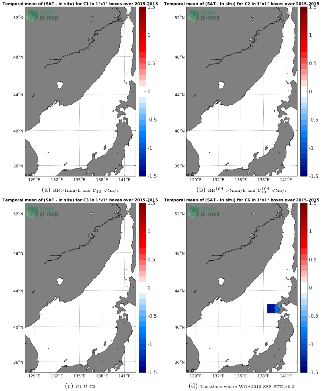
Figure 12: Temporal mean gridded over spatial boxes of size 1°x1° of \Delta\text{SSS} (SMOS-L4-CATDS-CECOS-IFREMER-V2-WEEKLY-0.5DEG - TSG-LEGOS-DM) for 4 different subdatasets corresponding to: RR > 1\text{mm/h} and U_{10} < 5\text{m/s} (a), RR^{10d} > 5\text{mm/h} and U_{10}^{10d} < 5\text{m/s} (b), C1 U C2 (c), Locations where WOA2013 SSS STD > 0.2 (d).
