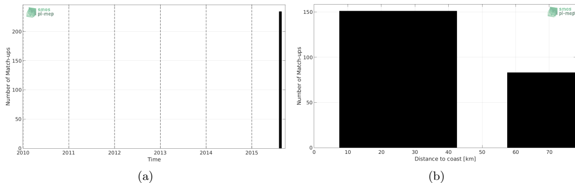
Figure 1: Number of match-ups between TSG-LEGOS-DM and SMOS-L4-CATDS-CECOS-IFREMER-V2-WEEKLY-0.5DEG SSS as a function of time (a) and as function of the distance to coast (b) over the Sea of Japan Pi-MEP region and for the full satellite product period.
