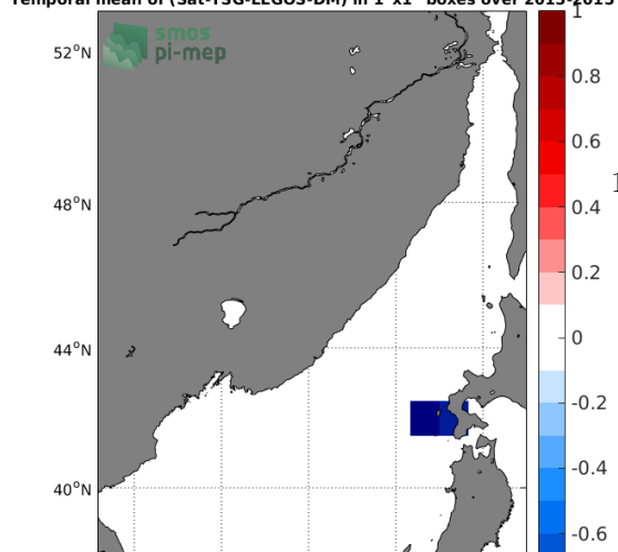
Temporal mean of (Sat-TSG-LEGOS-DM) in 1°x1° boxes over 2015-2015
