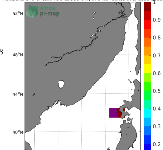
Temporal STD of (Sat-TSG-LEGOS-DM) in 1°x1° boxes over 2015-2015
