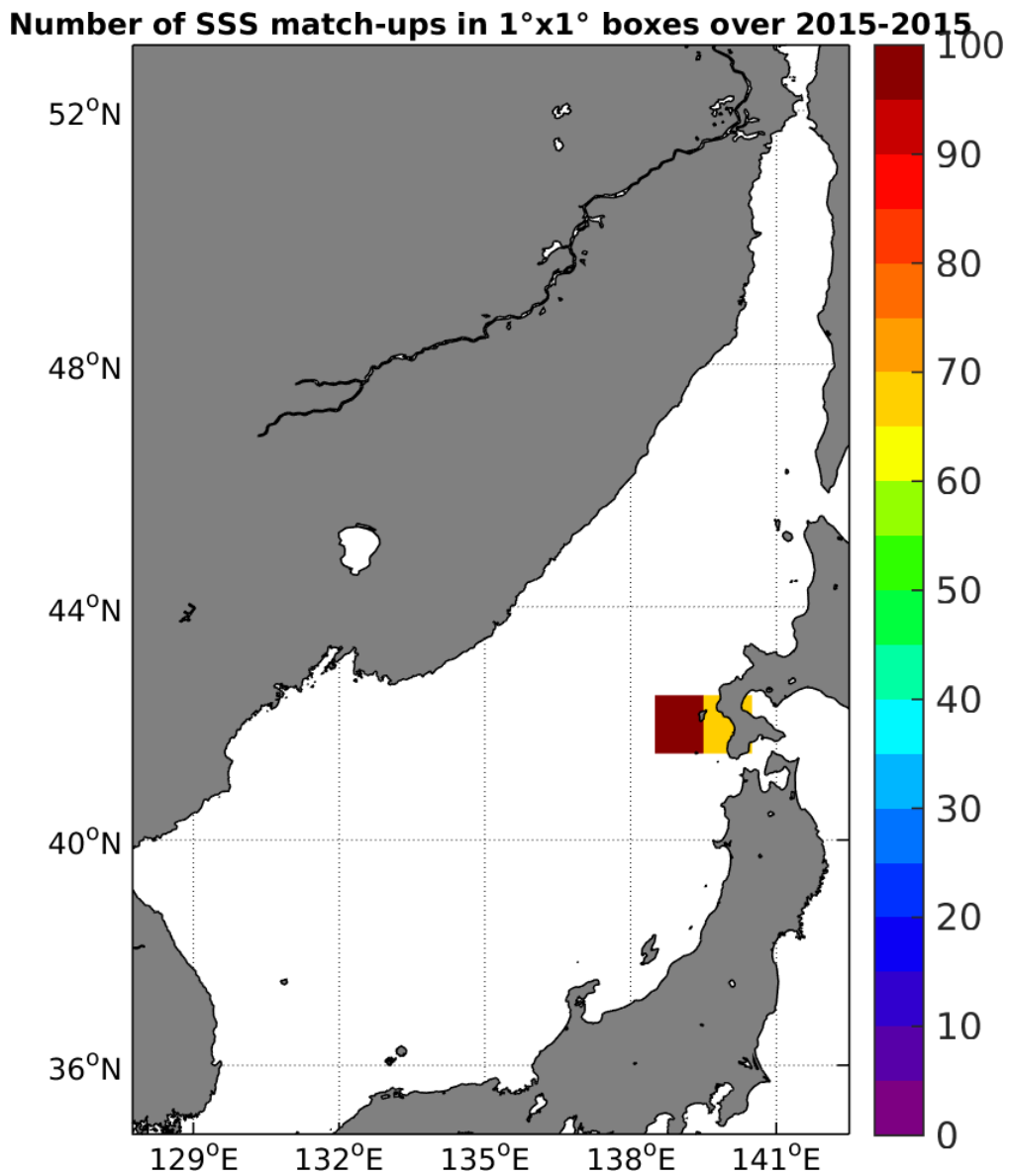
Figure 4: Number of SSS match-ups between TSG-LEGOS-DM SSS and the SMOS-L4-CATDS-CECOS-IFREMER-V2-WEEKLY-0.5DEG SSS product for the Sea of Japan Pi-MEP region over 1°x1° boxes and for the full satellite product period.
