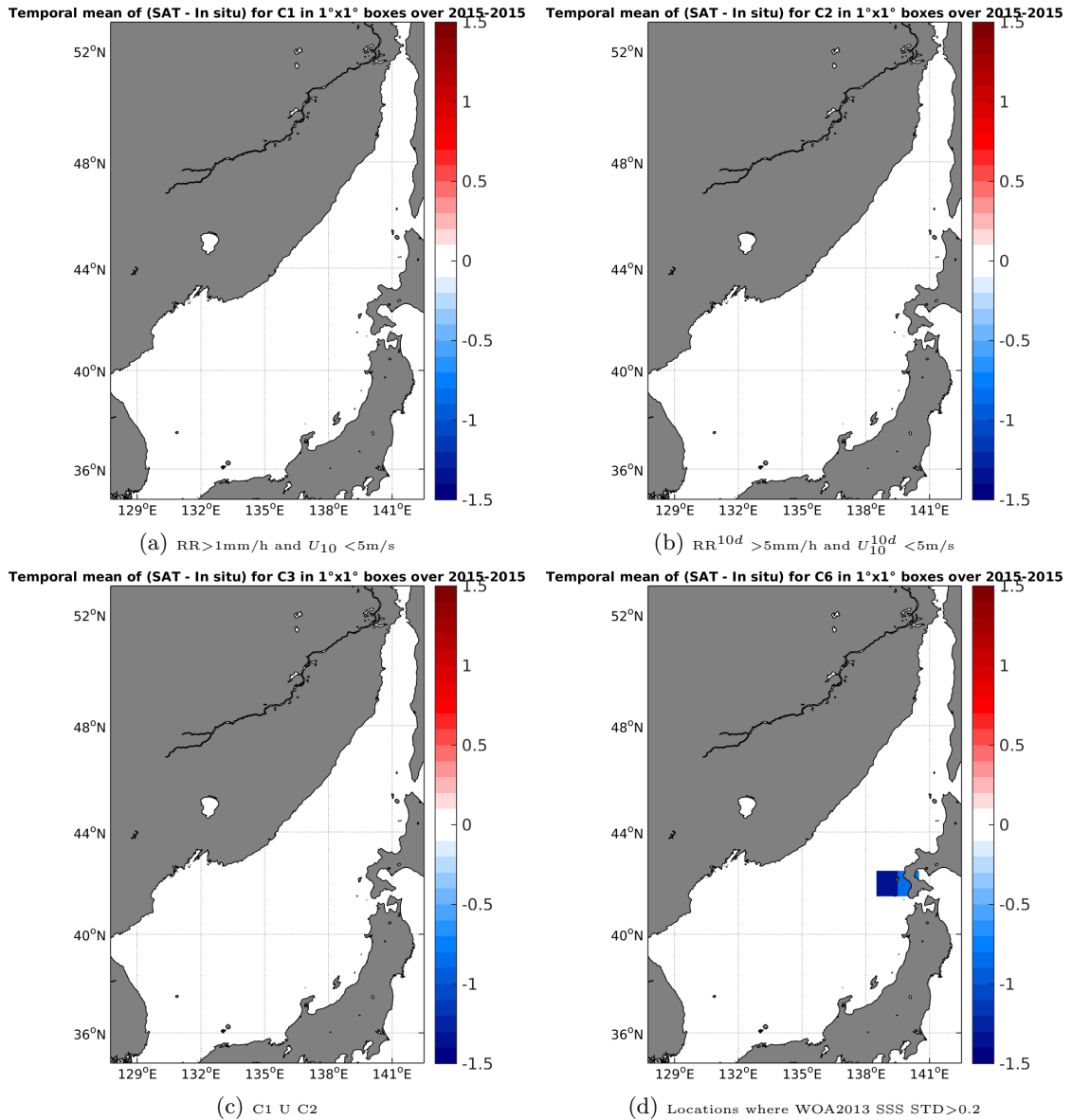
Figure 12: Temporal mean gridded over spatial boxes of size 1°x1° of \Delta SSS (SMOS-L4-CATDS-CECOS-IFREMER-V2-WEEKLY-0.5DEG - TSG-LEGOS-DM) for 4 different subdatasets corresponding to: RR > 1\text{mm/h} and U_{10} < 5\text{m/s} (a), RR^{10d} > 5\text{mm/h} and U_{10}^{10d} < 5\text{m/s} (b), C1 U C2 (c), Locations where WOA2013 SSS STD > 0.2 (d).
