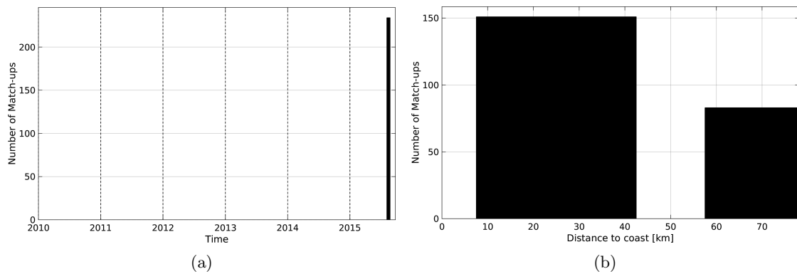
Figure 1: Number of match-ups between TSG-LEGOS-DM and SMOS-L4-CATDS-CECOS-IFREMER-V2-WEEKLY-0.5DEG SSS as a function of time (a) and as function of the distance to coast (b) over the Sea of Japan Pi-MEP region and for the full satellite product period.
