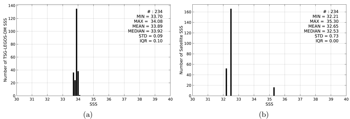
Figure 2: Histograms of SSS from TSG-LEGOS-DM (a) and SMOS-L4-CATDS-CECOS-IFREMER-V2-WEEKLY-0.5DEG (b) considering all match-up pairs per bins of 0.1 over the Sea of Japan Pi-MEP region and for the full satellite product period.
