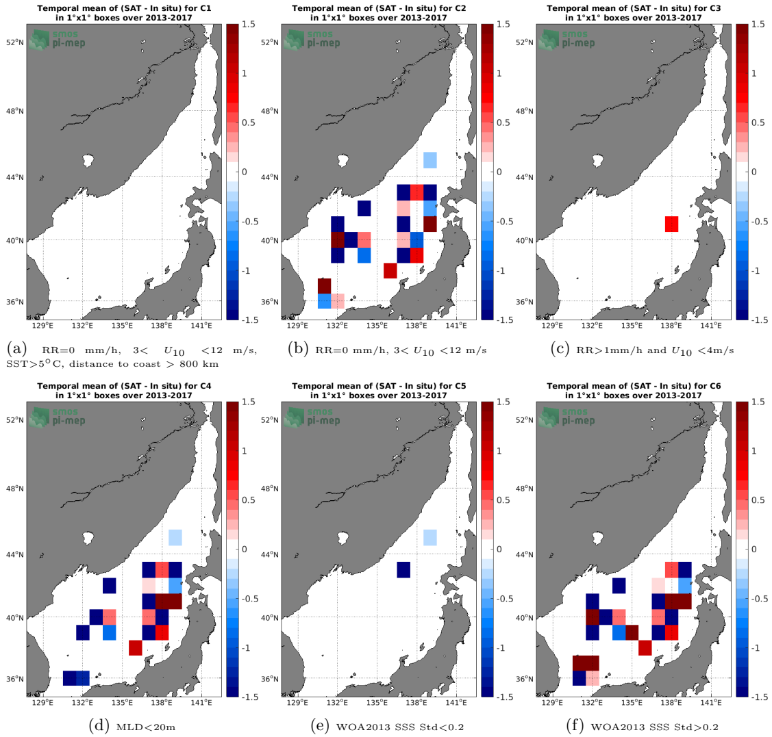
Figure 12: Temporal mean gridded over spatial boxes of size 1°x1° of \Delta SSS (SMOS L4 v2 Weekly (CATDS-CECOS-IFREMER) - Argo) for 6 different subdatasets corresponding to: RR=0 mm/h, 3 < U_{10} < 12 m/s, SST > 5°C, distance to coast > 800 km (a), RR=0 mm/h, 3 < U_{10} < 12 m/s (b), RR > 1mm/h and U_{10} < 4 m/s (c), MLD < 20m (d), WOA2013 SSS Std < 0.2 (e), WOA2013 SSS Std > 0.2 (f).
