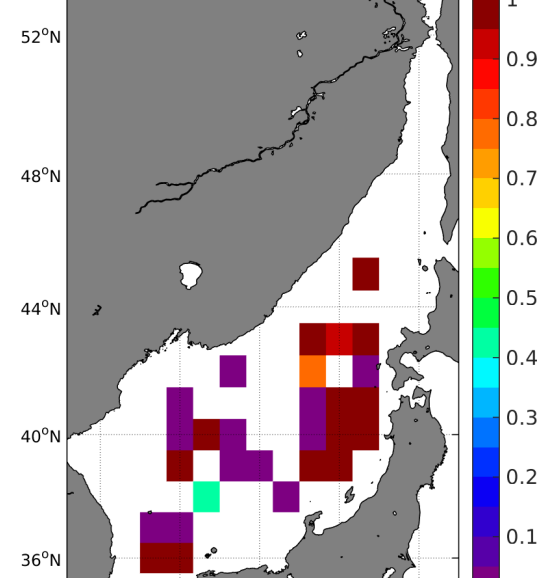
Temporal STD of (Sat-Argo) in 1°x1° boxes over 2013-2017
