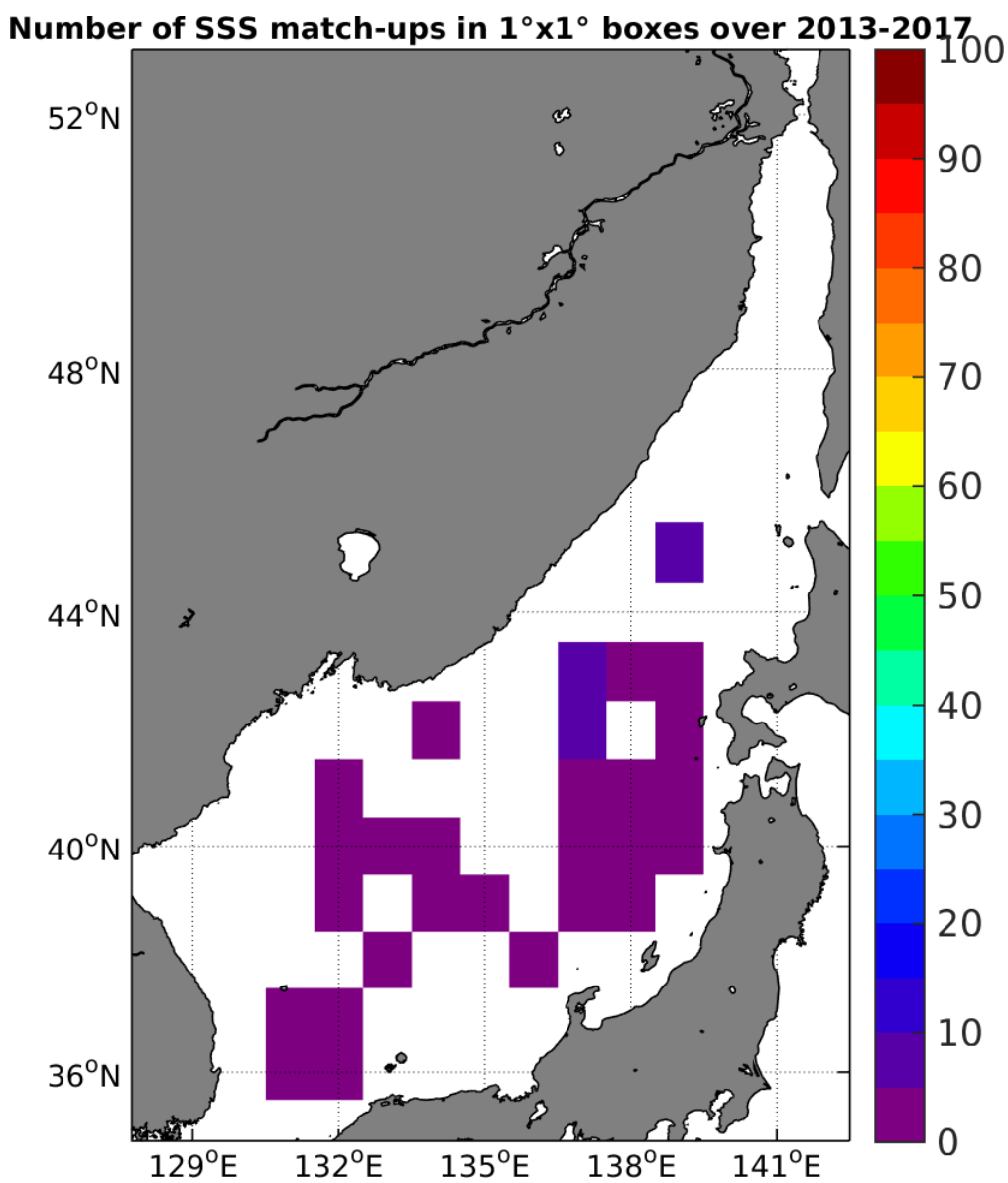
Figure 4: Number of SSS match-ups between Argo SSS and the SMOS-L4-CATDS-CECOS-IFREMER-V2-WEEKLY-0.5DEG SSS product for the Sea of Japan Pi-MEP region over 1°x1° boxes and for the full satellite product period.
