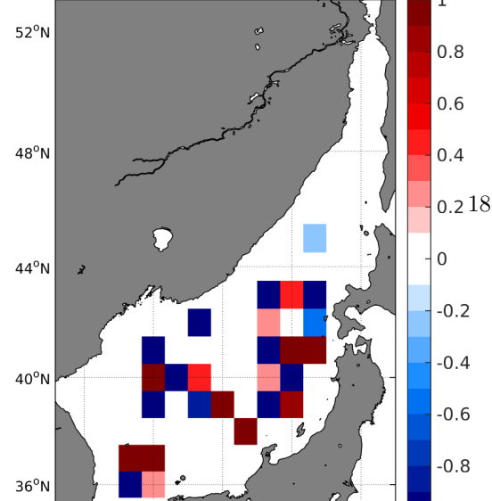
Temporal mean of (Sat-Argo) in 1°x1° boxes over 2013-2017
