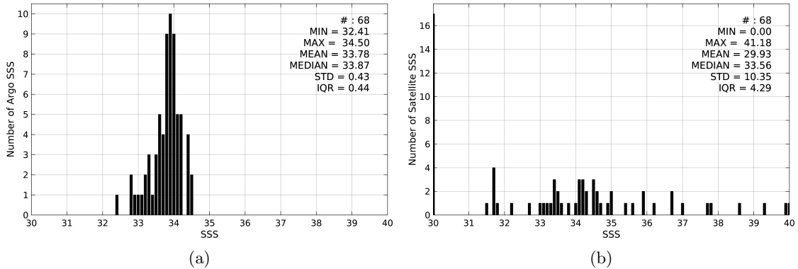
Figure 2: Histograms of SSS from Argo (a) and SMOS-L4-CATDS-CECOS-IFREMER-V2-WEEKLY-0.5DEG (b) considering all match-up pairs per bins of 0.1 over the Sea of Japan Pi-MEP region and for the full satellite product period.
