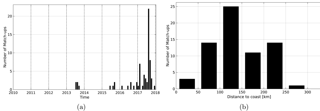
Figure 1: Number of match-ups between Argo and SMOS-L4-CATDS-CECOS-IFREMER-V2-WEEKLY-0.5DEG SSS as a function of time (a) and as function of the distance to coast (b) over the Sea of Japan Pi-MEP region and for the full satellite product period.
