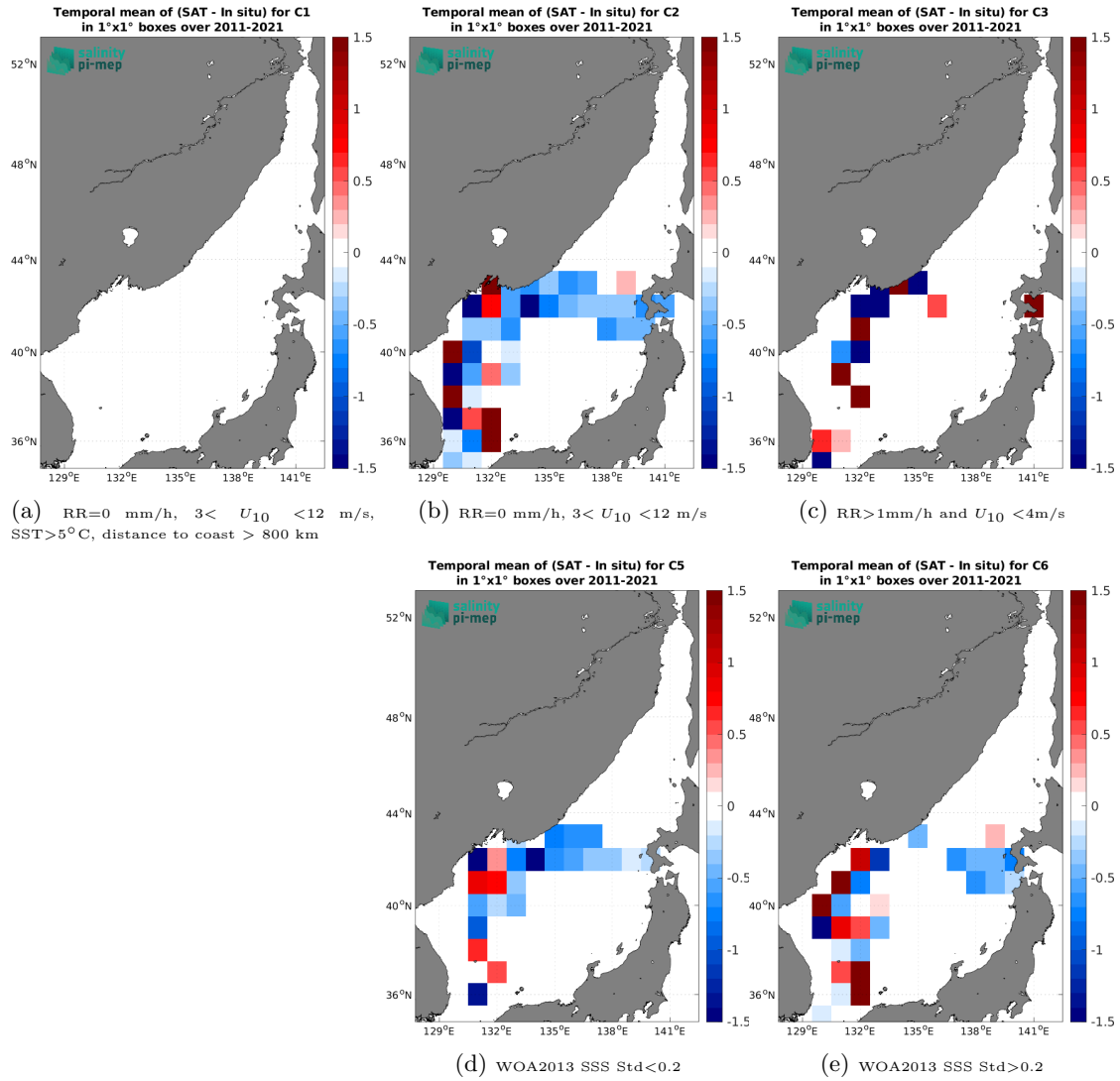
Figure 14: Temporal mean gridded over spatial boxes of size 1^\circ \times 1^\circ of \Delta\text{SSS} (SMOS SSS L4 v2 - Daily (BEC) - TSG (LEGOS-DM)) for 5 different subdatasets corresponding to: RR=0 mm/h, 3 < U_{10} < 12 m/s, SST > 5^\circ\text{C} , distance to coast > 800 km (a), RR=0 mm/h, 3 < U_{10} < 12 m/s (b), RR > 1 mm/h and U_{10} < 4 m/s (c), WOA2013 SSS Std < 0.2 (d), WOA2013 SSS Std > 0.2 (e).
