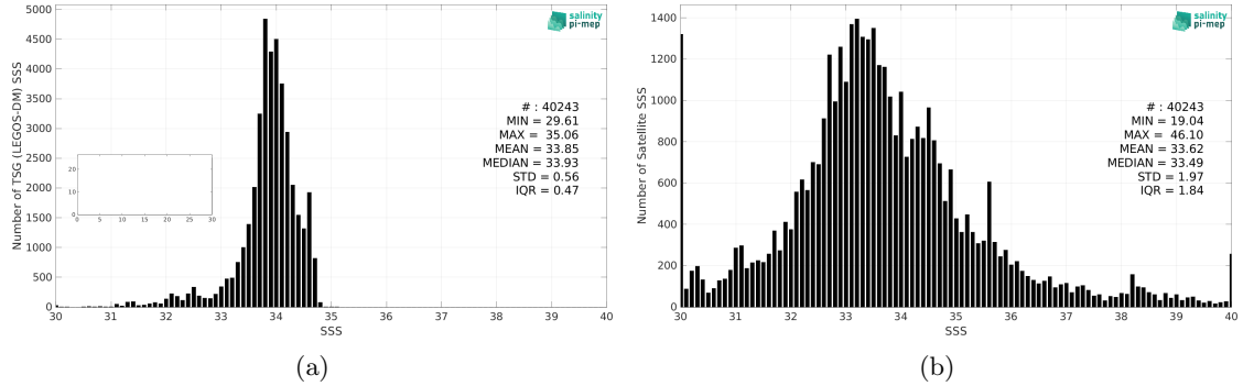
Figure 2: Histograms of SSS from TSG (LEGOS-DM) (a) and SMOS SSS L4 v2 - Daily (BEC) (b) considering all match-up pairs per bins of 0.1 over the Sea of Japan Pi-MEP region and for the full satellite product period.
