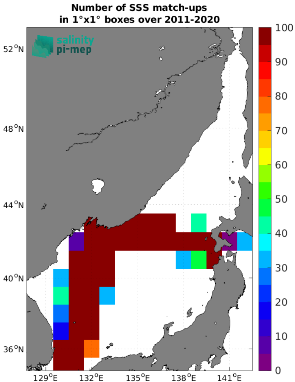
Figure 4: Number of SSS match-ups between TSG (LEGOS-DM) SSS and the SMOS SSS L4 v2 - Daily (BEC) SSS product for the Sea of Japan Pi-MEP region over 1°×1° boxes and for the full satellite product period.
