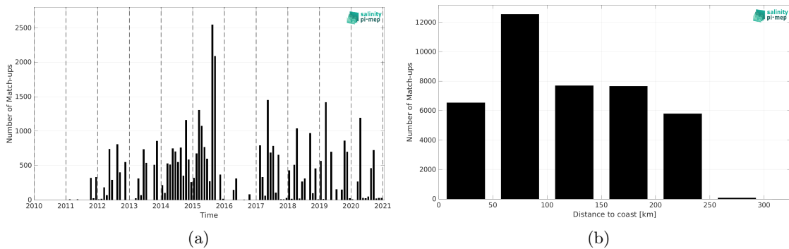
Figure 1: Number of match-ups between TSG (LEGOS-DM) and SMOS SSS L4 v2 - Daily (BEC) SSS as a function of time (a) and as function of the distance to coast (b) over the Sea of Japan Pi-MEP region and for the full satellite product period.
