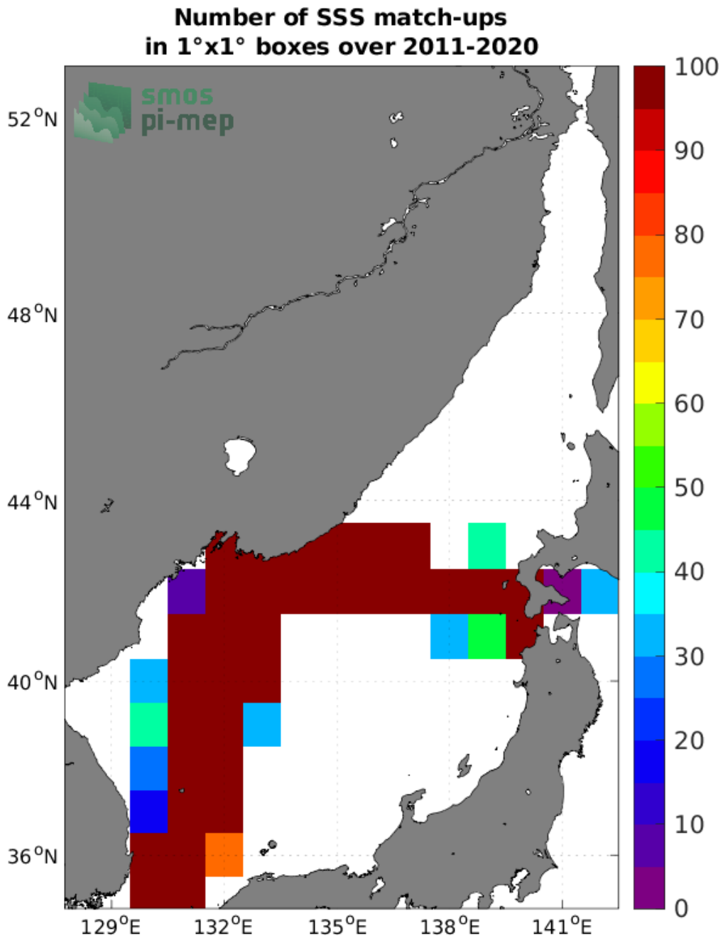
Figure 4: Number of SSS match-ups between TSG (LEGOS-DM) SSS and the SMOS SSS L4 v2 - Daily (BEC) SSS product for the Sea of Japan Pi-MEP region over 1^\circ \times 1^\circ boxes and for the full satellite product period.
