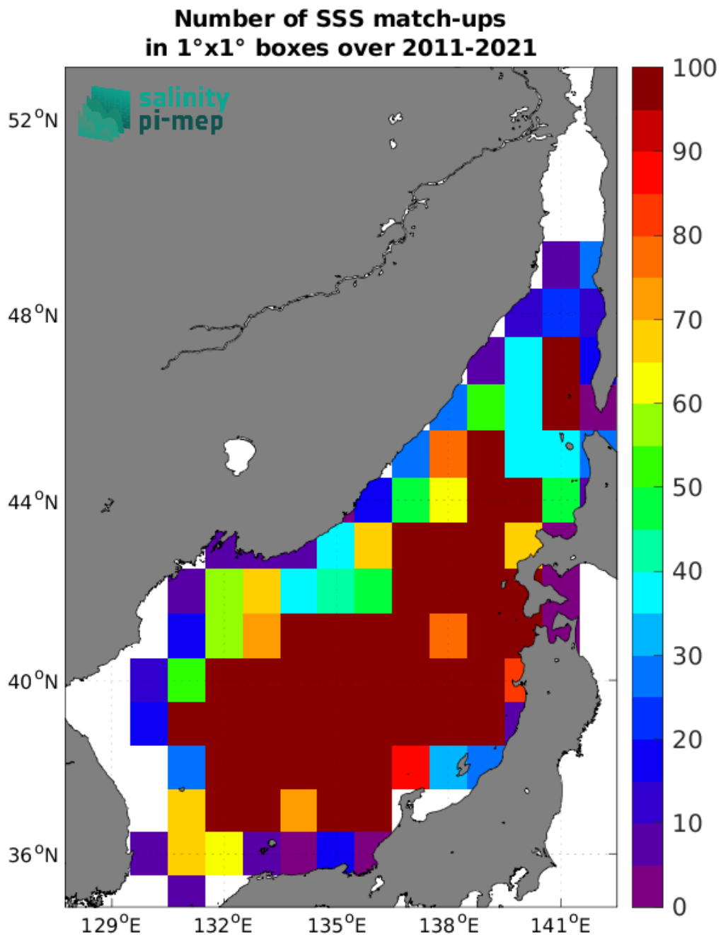
Figure 4: Number of SSS match-ups between Argo SSS and the SMOS SSS L4 v2 - Daily (BEC) SSS product for the Sea of Japan Pi-MEP region over 1°x1° boxes and for the full satellite product period.
