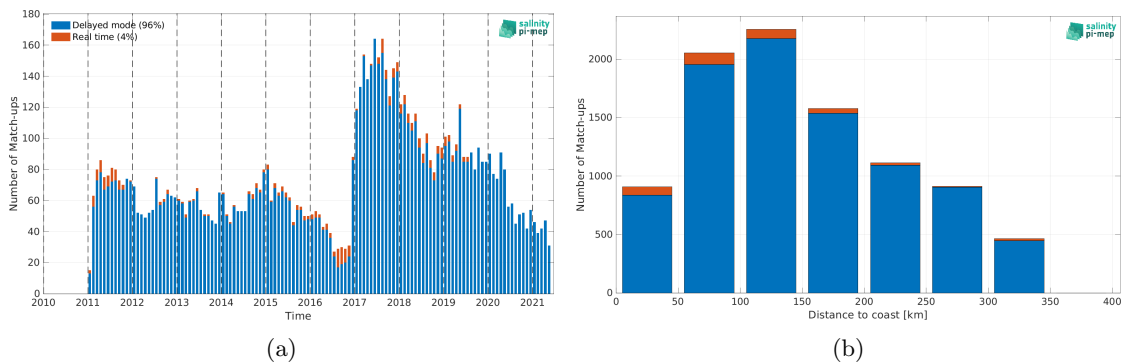
Figure 1: Number of match-ups between Argo and SMOS SSS L4 v2 - Daily (BEC) SSS as a function of time (a) and as function of the distance to coast (b) over the Sea of Japan Pi-MEP region and for the full satellite product period.
