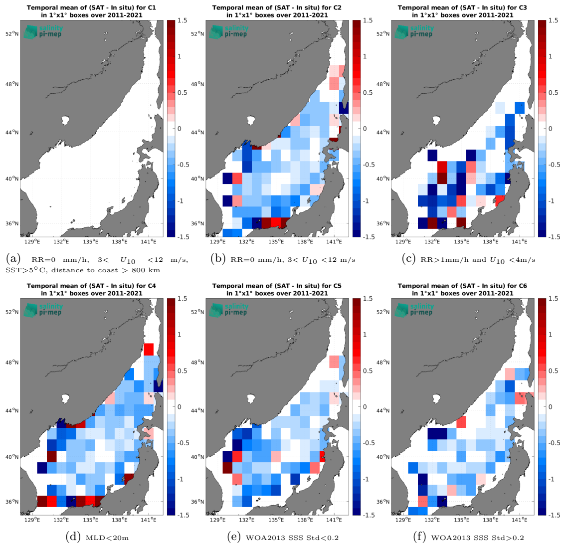
Figure 12: Temporal mean gridded over spatial boxes of size 1^\circ \times 1^\circ of \Delta SSS (SMOS SSS L4 v2 - Daily (BEC) - Argo) for 6 different subdatasets corresponding to: RR=0 mm/h, 3 < U_{10} < 12 m/s, SST > 5°C, distance to coast > 800 km (a), RR=0 mm/h, 3 < U_{10} < 12 m/s (b), RR > 1mm/h and U_{10} < 4 m/s (c), MLD < 20m (d), WOA2013 SSS Std < 0.2 (e), WOA2013 SSS Std > 0.2 (f).
