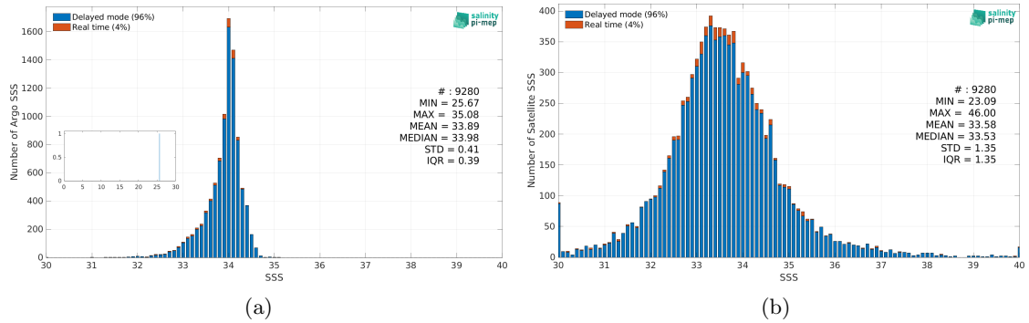
Figure 2: Histograms of SSS from Argo (a) and SMOS SSS L4 v2 - Daily (BEC) (b) considering all match-up pairs per bins of 0.1 over the Sea of Japan Pi-MEP region and for the full satellite product period.
