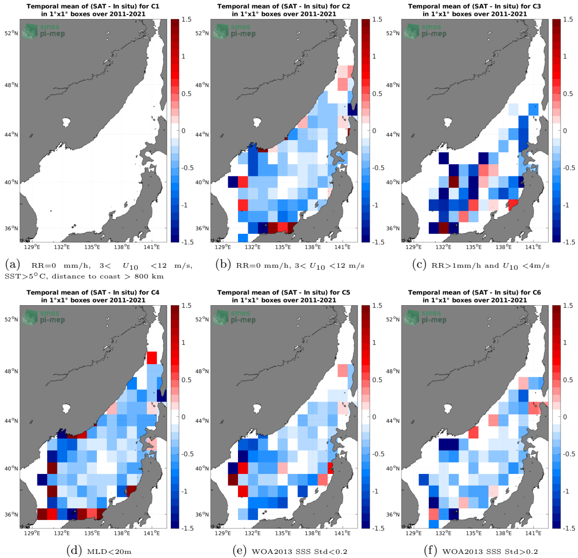
Figure 12: Temporal mean gridded over spatial boxes of size 1^\circ \times 1^\circ of \Delta\text{SSS} (SMOS SSS L4 v2 - Daily (BEC) - Argo) for 6 different subdatasets corresponding to: RR=0 mm/h, 3 < U_{10} < 12 m/s, SST > 5^\circ\text{C} , distance to coast > 800 km (a), RR=0 mm/h, 3 < U_{10} < 12 m/s (b), RR > 1 mm/h and U_{10} < 4 m/s (c), MLD < 20 m (d), WOA2013 SSS Std < 0.2 (e), WOA2013 SSS Std > 0.2 (f).
