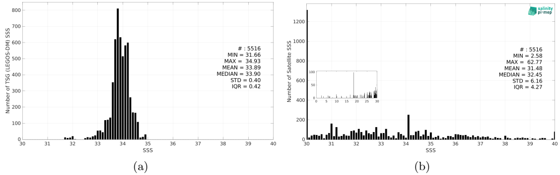
Figure 3: Histograms of SSS from TSG (LEGOS-DM) (a) and SMOS SSS L2Q v331 - With FLAG (CMEMS-CATDS-CPDC) (b) considering all match-up pairs per bins of 0.1 over the Sea of Japan Pi-MEP region and for the full satellite product period.
