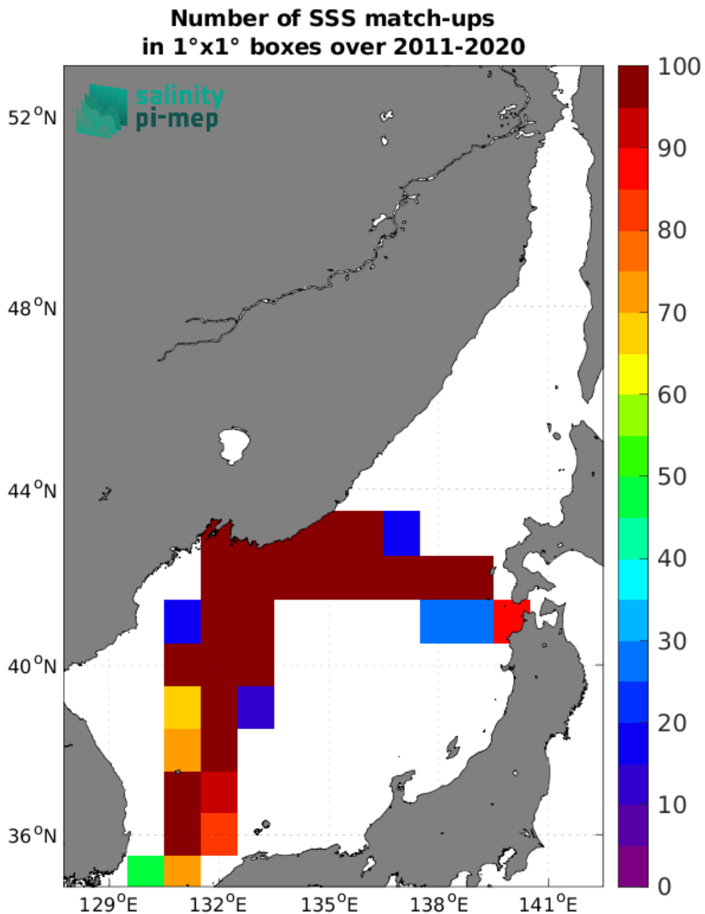
Figure 5: Number of SSS match-ups between TSG (LEGOS-DM) SSS and the SMOS SSS L2Q v331 - With FLAG (CMEMS-CATDS-CPDC) SSS product for the Sea of Japan Pi-MEP region over 1°x1° boxes and for the full satellite product period.
