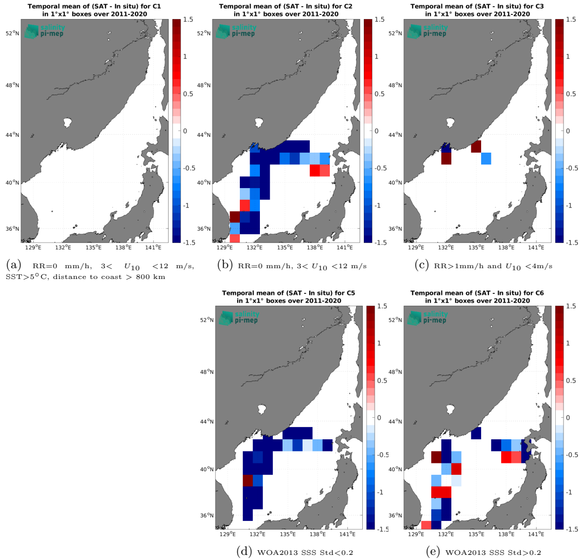
Figure 14: Temporal mean gridded over spatial boxes of size 1^\circ \times 1^\circ of \Delta\text{SSS} (SMOS SSS L2Q v331 - With FLAG (CMEMS-CATDS-CPDC) - TSG (LEGOS-DM)) for 5 different subdatasets corresponding to: RR=0 mm/h, 3 < U_{10} < 12 m/s, SST > 5^\circ\text{C} , distance to coast > 800 km (a), RR=0 mm/h, 3 < U_{10} < 12 m/s (b), RR > 1\text{mm/h} and U_{10} < 4\text{m/s} (c), WOA2013 SSS Std < 0.2 (d), WOA2013 SSS Std > 0.2 (e).
