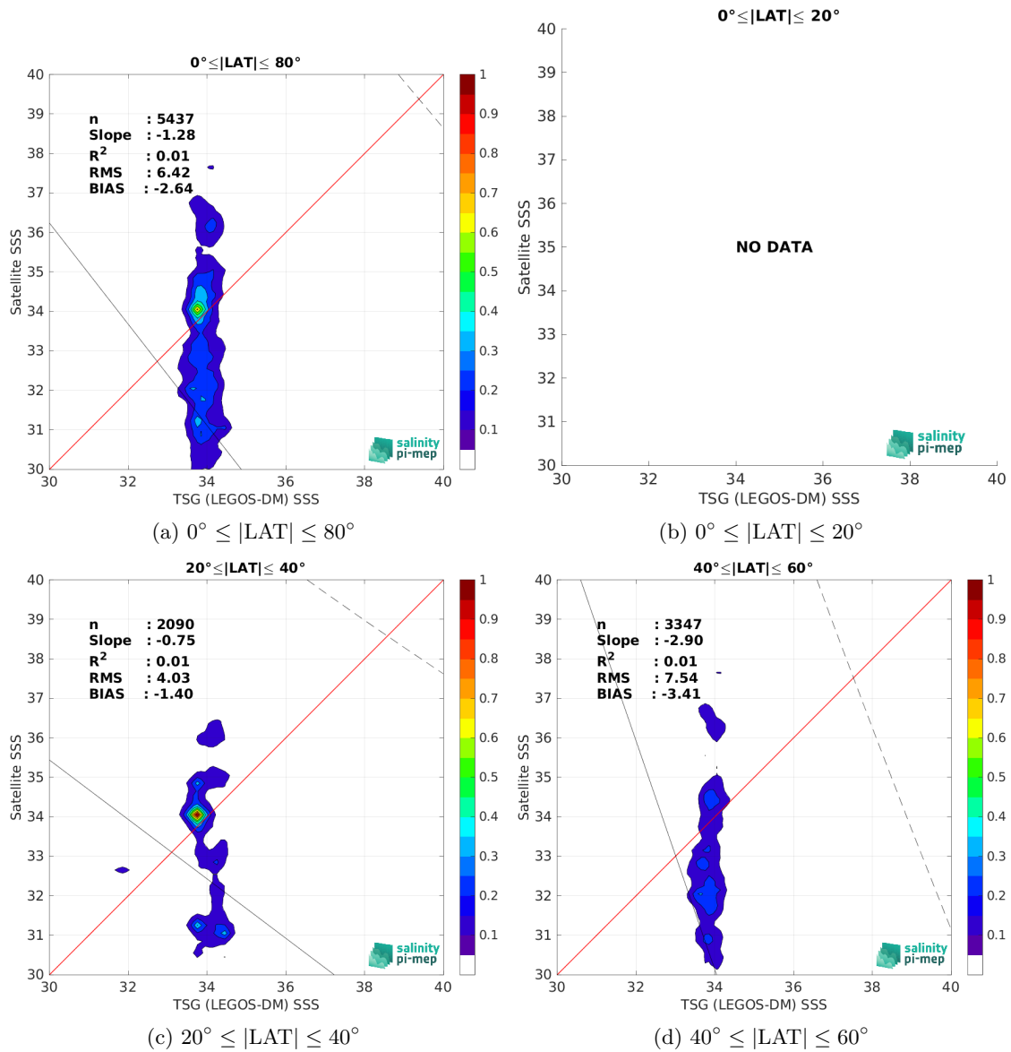
Figure 10: Contour maps of the concentration of SMOS SSS L2Q v331 - With FLAG (CMEMS-CATDS-CPDC) SSS (y-axis) versus TSG (LEGOS-DM) SSS (x-axis) at match-up pairs for different latitude bands. For each plot, the red line shows x=y . The black thin and dashed lines indicate a linear fit through the data cloud and the \pm 95\% confidence levels, respectively. The number match-up pairs n , the slope and R^2 coefficient of the linear fit, the root mean square (RMS) and the mean bias between satellite and in situ data are indicated for each latitude band in each plots.
