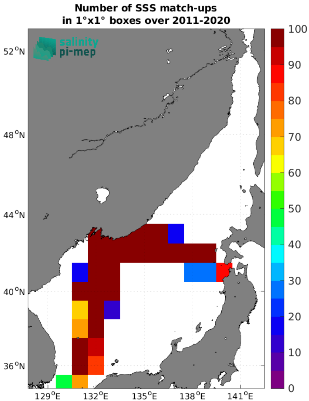
Figure 4: Number of SSS match-ups between TSG (LEGOS-DM) SSS and the SMOS SSS L2Q v331 - With FLAG (CMEMS-CATDS-CPDC) SSS product for the Sea of Japan Pi-MEP region over 1°x1° boxes and for the full satellite product period.
