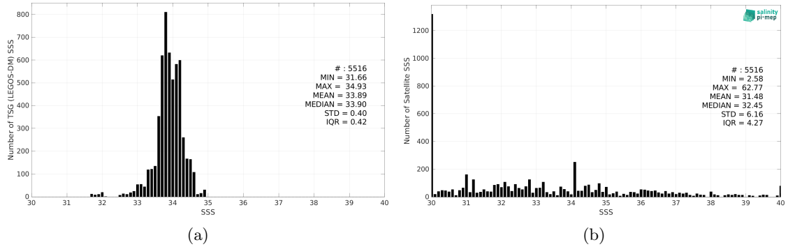
Figure 2: Histograms of SSS from TSG (LEGOS-DM) (a) and SMOS SSS L2Q v331 - With FLAG (CMEMS-CATDS-CPDC) (b) considering all match-up pairs per bins of 0.1 over the Sea of Japan Pi-MEP region and for the full satellite product period.
