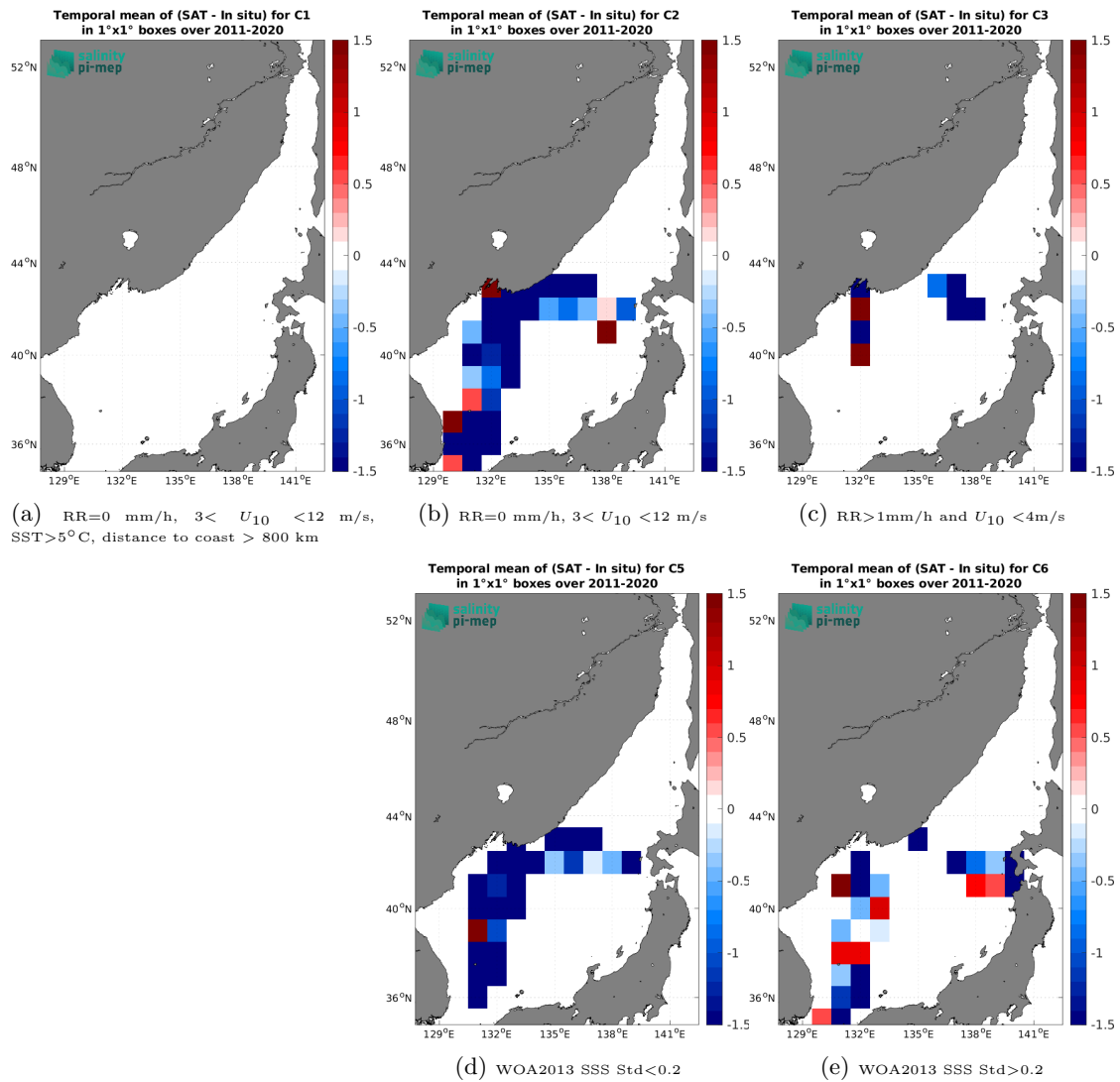
Figure 12: Temporal mean gridded over spatial boxes of size 1^\circ \times 1^\circ of \Delta\text{SSS} (SMOS SSS L2Q v331 - With FLAG (CMEMS-CATDS-CPDC) - TSG (LEGOS-DM)) for 5 different subdatasets corresponding to: RR=0 mm/h, 3 < U_{10} < 12 m/s, SST > 5^\circ\text{C} , distance to coast > 800 km (a), RR=0 mm/h, 3 < U_{10} < 12 m/s (b), RR > 1 mm/h and U_{10} < 4 m/s (c), WOA2013 SSS Std < 0.2 (d), WOA2013 SSS Std > 0.2 (e).
