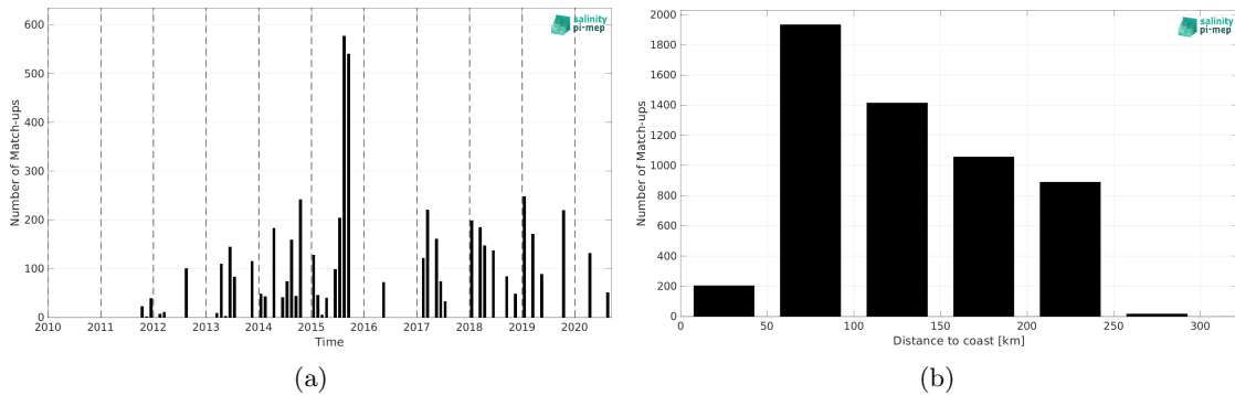
Figure 1: Number of match-ups between TSG (LEGOS-DM) and SMOS SSS L2Q v331 - With FLAG (CMEMS-CATDS-CPDC) SSS as a function of time (a) and as function of the distance to coast (b) over the Sea of Japan Pi-MEP region and for the full satellite product period.
