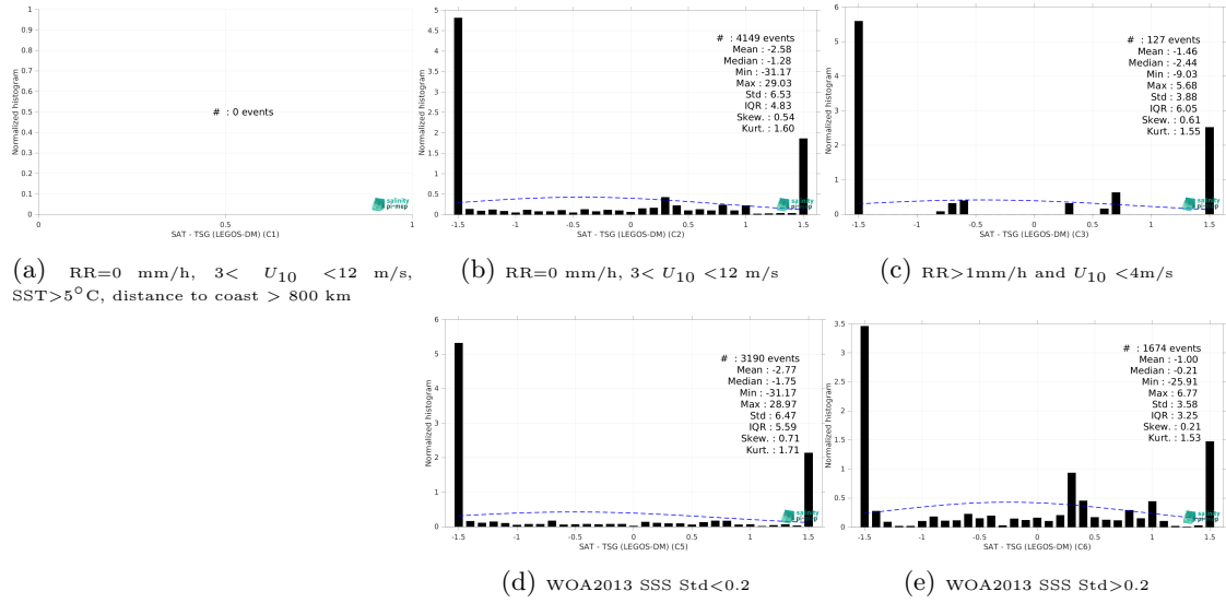
Figure 13: Normalized histogram of \Delta SSS (SMOS SSS L2Q v331 - With FLAG (CMEMS-CATDS-CPDC) - TSG (LEGOS-DM)) for 5 different subdatasets corresponding to: RR=0 mm/h, 3 < U_{10} < 12 m/s, SST > 5°C, distance to coast > 800 km (a), RR=0 mm/h, 3 < U_{10} < 12 m/s (b), RR > 1mm/h and U_{10} < 4 m/s (c), WOA2013 SSS Std < 0.2 (d), WOA2013 SSS Std > 0.2 (e).
