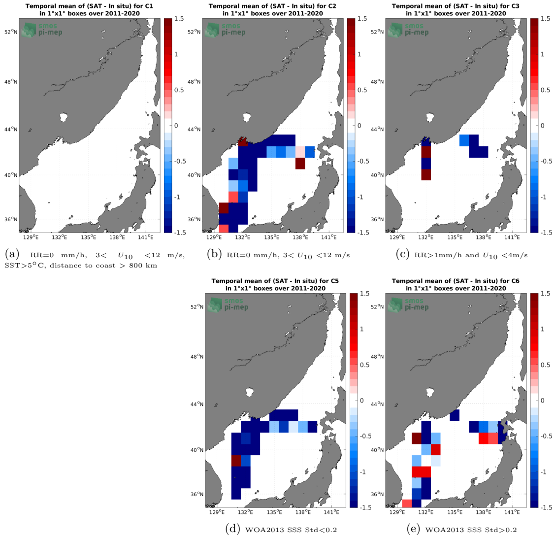
Figure 12: Temporal mean gridded over spatial boxes of size 1^\circ \times 1^\circ of \Delta SSS (SMOS SSS L2Q v331 - With FLAG (CMEMS-CATDS-CPDC) - TSG (LEGOS-DM)) for 5 different subdatasets corresponding to: RR=0 mm/h, 3 < U_{10} < 12 m/s, SST>5°C, distance to coast > 800 km (a), RR=0 mm/h, 3 < U_{10} < 12 m/s (b), RR>1mm/h and U_{10} < 4 m/s (c), WOA2013 SSS Std<0.2 (d), WOA2013 SSS Std>0.2 (e).
