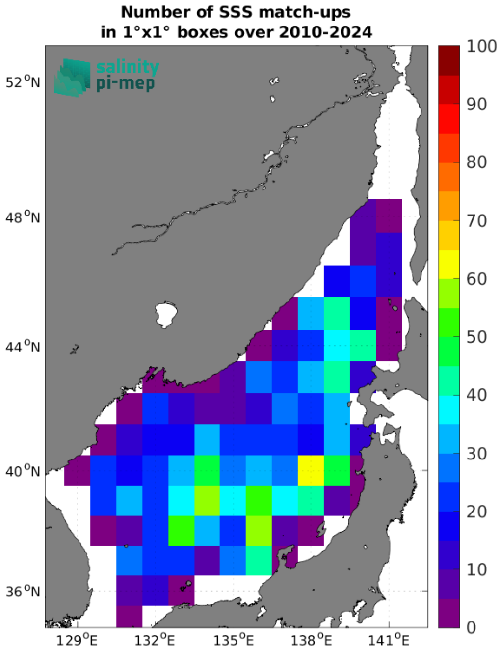
Figure 5: Number of SSS match-ups between Argo SSS and the SMOS SSS L2Q v331 - With FLAG (CMEMS-CATDS-CPDC) SSS product for the Sea of Japan Pi-MEP region over 1°x1° boxes and for the full satellite product period.
