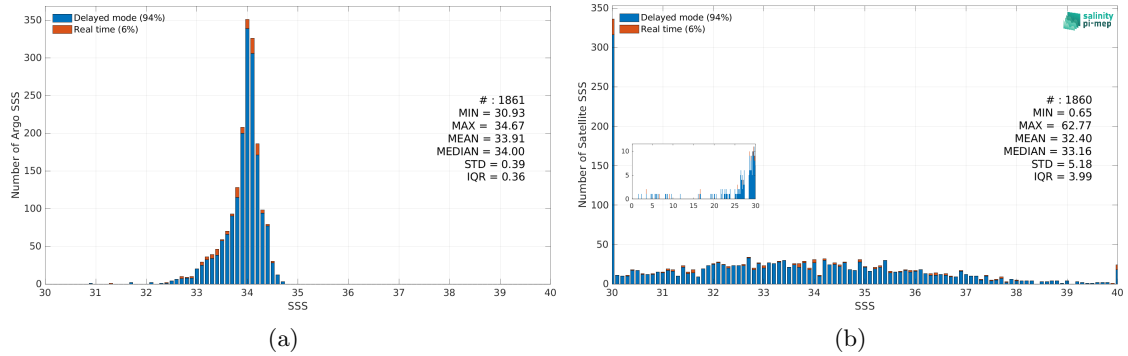
Figure 3: Histograms of SSS from Argo (a) and SMOS SSS L2Q v331 - With FLAG (CMEMS-CATDS-CPDC) (b) considering all match-up pairs per bins of 0.1 over the Sea of Japan Pi-MEP region and for the full satellite product period.
