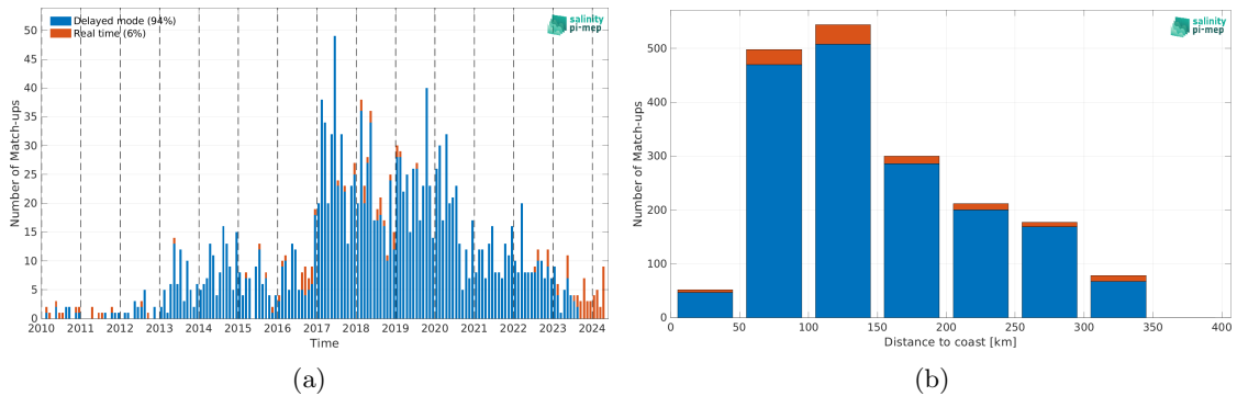
Figure 2: Number of match-ups between Argo and SMOS SSS L2Q v331 - With FLAG (CMEMS-CATDS-CPDC) SSS as a function of time (a) and as function of the distance to coast (b) over the Sea of Japan Pi-MEP region and for the full satellite product period.
