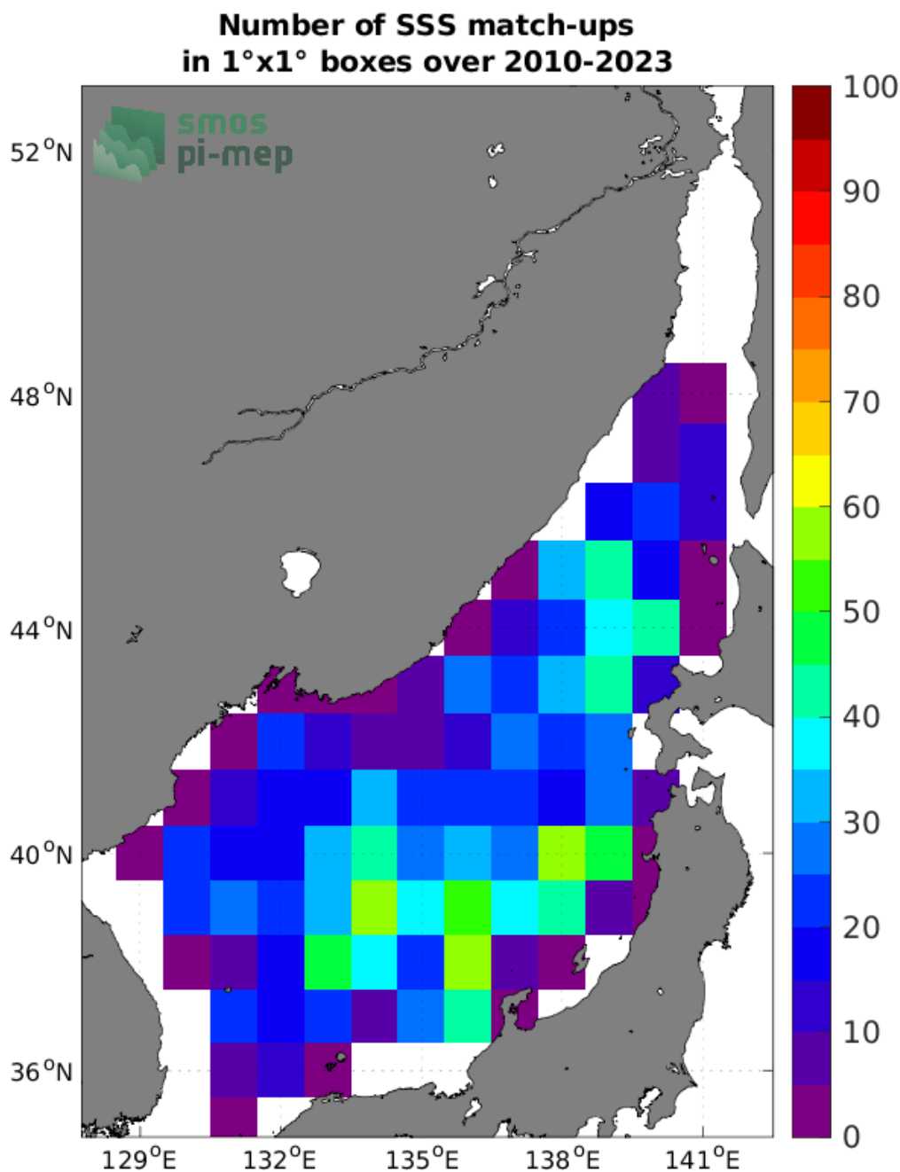
Figure 4: Number of SSS match-ups between Argo SSS and the SMOS SSS L2Q v331 - With FLAG (CMEMS-CATDS-CPDC) SSS product for the Sea of Japan Pi-MEP region over 1°x1° boxes and for the full satellite product period.
