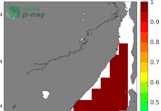
Temporal STD of (Sat - Argo) in 1°x1° boxes over 2010-2023
