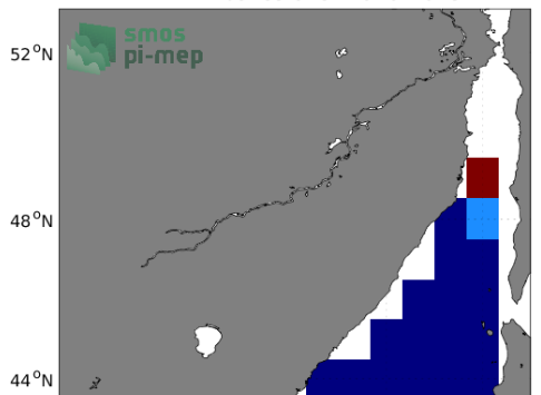
Temporal mean of (Sat - Argo) in 1°x1° boxes over 2010-2023
