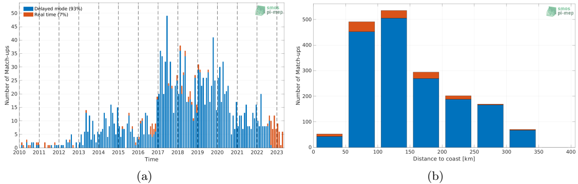
Figure 1: Number of match-ups between Argo and SMOS SSS L2Q v331 - With FLAG (CMEMS-CATDS-CPDC) SSS as a function of time (a) and as function of the distance to coast (b) over the Sea of Japan Pi-MEP region and for the full satellite product period.
