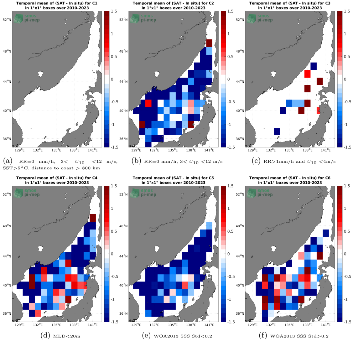
Figure 12: Temporal mean gridded over spatial boxes of size 1^\circ \times 1^\circ of \Delta\text{SSS} (SMOS SSS L2Q v331 - With FLAG (CMEMS-CATDS-CPDC) - Argo) for 6 different subdatasets corresponding to: RR=0 mm/h, 3 < U_{10} < 12 m/s, SST > 5^\circ\text{C} , distance to coast > 800 km (a), RR=0 mm/h, 3 < U_{10} < 12 m/s (b), RR > 1 mm/h and U_{10} < 4 m/s (c), MLD < 20 m (d), WOA2013 SSS Std < 0.2 (e), WOA2013 SSS Std > 0.2 (f).
