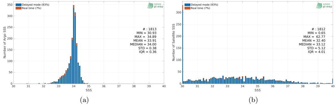
Figure 2: Histograms of SSS from Argo (a) and SMOS SSS L2Q v331 - With FLAG (CMEMS-CATDS-CPDC) (b) considering all match-up pairs per bins of 0.1 over the Sea of Japan Pi-MEP region and for the full satellite product period.
