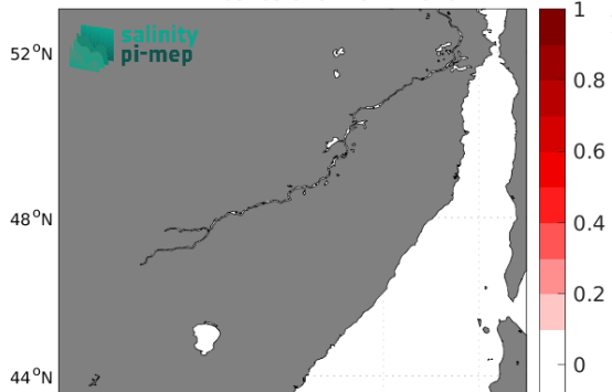
Temporal mean of (Sat - TSG (LEGOS-DM)) in 1°x1° boxes over 2011-2020
