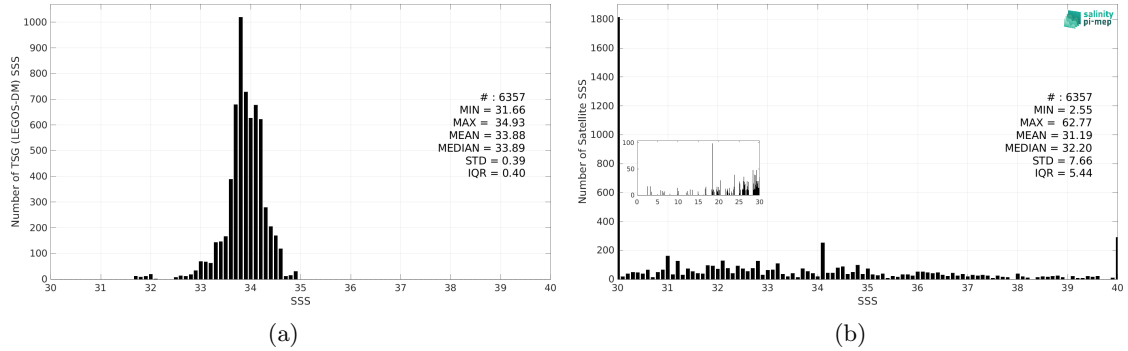
Figure 3: Histograms of SSS from TSG (LEGOS-DM) (a) and SMOS SSS L2Q v331 - No FLAG (CMEMS-CATDS-CPDC) (b) considering all match-up pairs per bins of 0.1 over the Sea of Japan Pi-MEP region and for the full satellite product period.
