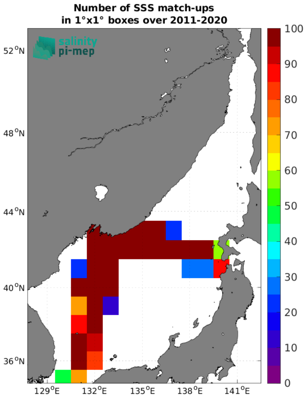
Figure 5: Number of SSS match-ups between TSG (LEGOS-DM) SSS and the SMOS SSS L2Q v331 - No FLAG (CMEMS-CATDS-CPDC) SSS product for the Sea of Japan Pi-MEP region over 1°×1° boxes and for the full satellite product period.
