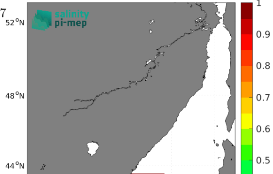
Temporal STD of (Sat - TSG (LEGOS-DM)) in 1°x1° boxes over 2011-2020
