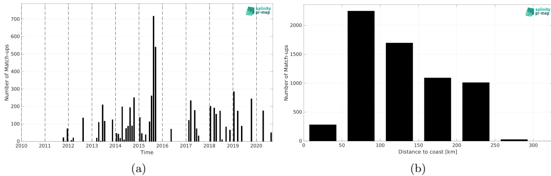
Figure 2: Number of match-ups between TSG (LEGOS-DM) and SMOS SSS L2Q v331 - No FLAG (CMEMS-CATDS-CPDC) SSS as a function of time (a) and as function of the distance to coast (b) over the Sea of Japan Pi-MEP region and for the full satellite product period.
