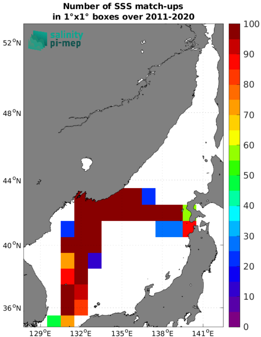
Figure 4: Number of SSS match-ups between TSG (LEGOS-DM) SSS and the SMOS SSS L2Q v331 - No FLAG (CMEMS-CATDS-CPDC) SSS product for the Sea of Japan Pi-MEP region over 1°x1° boxes and for the full satellite product period.
