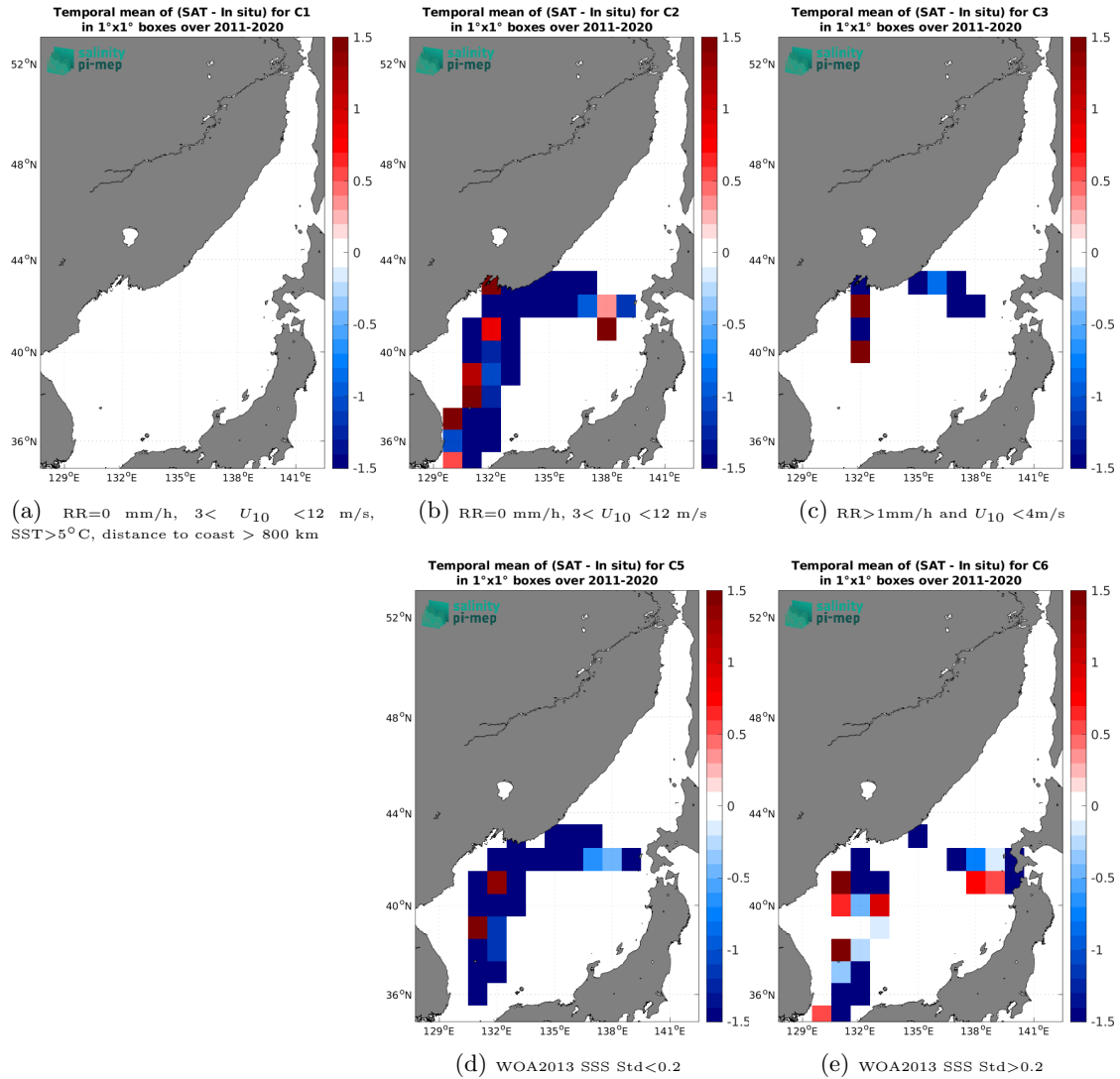
Figure 12: Temporal mean gridded over spatial boxes of size 1^\circ \times 1^\circ of \Delta\text{SSS} (SMOS SSS L2Q v331 - No FLAG (CMEMS-CATDS-CPDC) - TSG (LEGOS-DM)) for 5 different subdatasets corresponding to: RR=0 mm/h, 3 < U_{10} < 12 m/s, SST > 5^\circ\text{C} , distance to coast > 800 km (a), RR=0 mm/h, 3 < U_{10} < 12 m/s (b), RR > 1\text{mm/h} and U_{10} < 4\text{m/s} (c), WOA2013 SSS Std < 0.2 (d), WOA2013 SSS Std > 0.2 (e).
