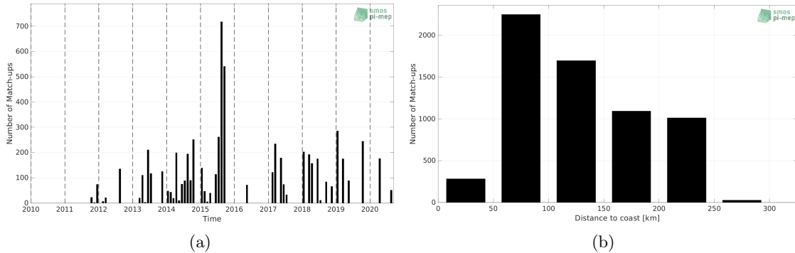
Figure 1: Number of match-ups between TSG (LEGOS-DM) and SMOS SSS L2Q v331 - No FLAG (CMEMS-CATDS-CPDC) SSS as a function of time (a) and as function of the distance to coast (b) over the Sea of Japan Pi-MEP region and for the full satellite product period.
