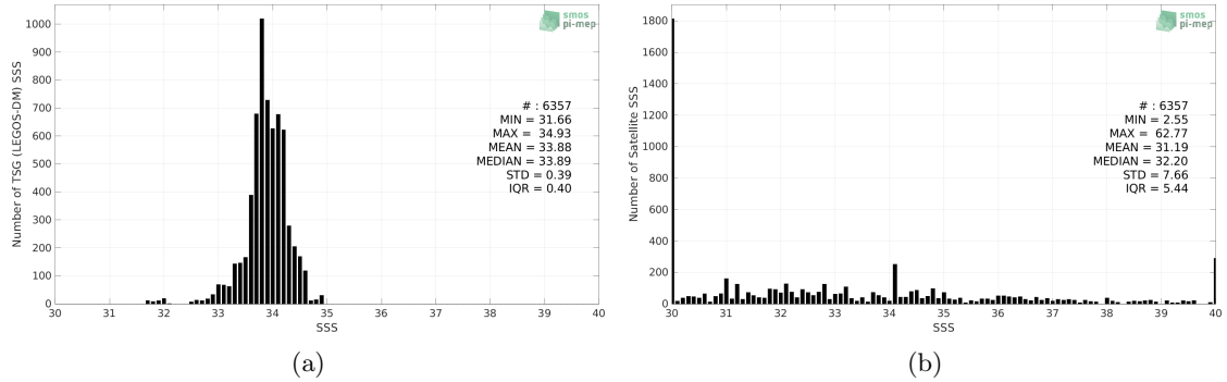
Figure 2: Histograms of SSS from TSG (LEGOS-DM) (a) and SMOS SSS L2Q v331 - No FLAG (CMEMS-CATDS-CPDC) (b) considering all match-up pairs per bins of 0.1 over the Sea of Japan Pi-MEP region and for the full satellite product period.
