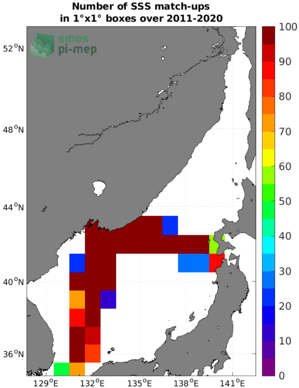
Figure 4: Number of SSS match-ups between TSG (LEGOS-DM) SSS and the SMOS SSS L2Q v331 - No FLAG (CMEMS-CATDS-CPDC) SSS product for the Sea of Japan Pi-MEP region over 1°×1° boxes and for the full satellite product period.
