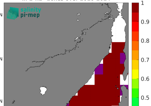
Temporal STD of (Sat - Argo) in 1°x1° boxes over 2010-2024
