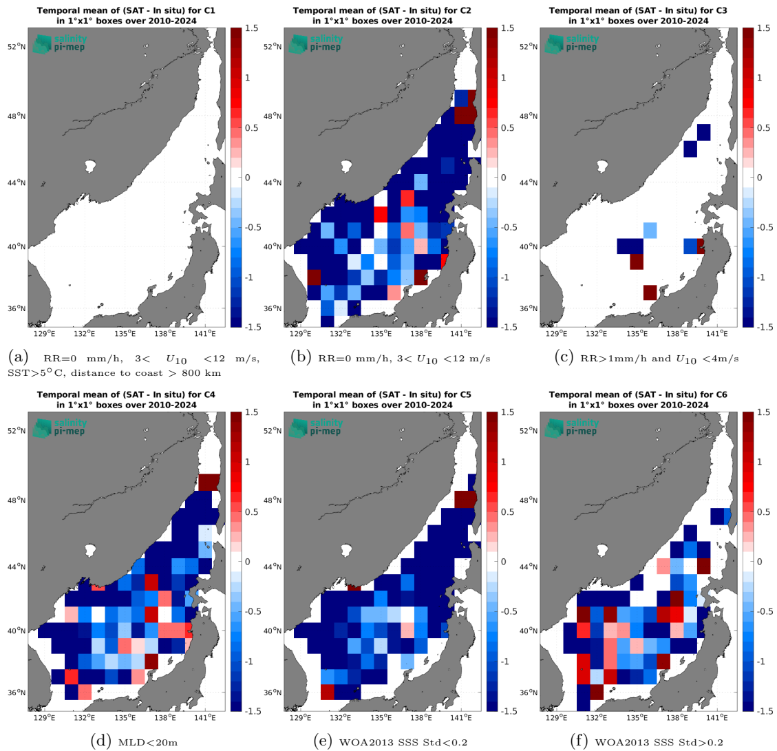
Figure 14: Temporal mean gridded over spatial boxes of size 1^\circ \times 1^\circ of \Delta SSS (SMOS SSS L2Q v331 - No FLAG (CMEMS-CATDS-CPDC) - Argo) for 6 different subdatasets corresponding to: RR=0 mm/h, 3 < U_{10} < 12 m/s, SST > 5°C, distance to coast > 800 km (a), RR=0 mm/h, 3 < U_{10} < 12 m/s (b), RR > 1mm/h and U_{10} < 4 m/s (c), MLD < 20m (d), WOA2013 SSS Std < 0.2 (e), WOA2013 SSS Std > 0.2 (f).
