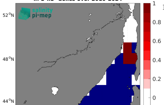
Temporal mean of (Sat - Argo) in 1°x1° boxes over 2010-2024
