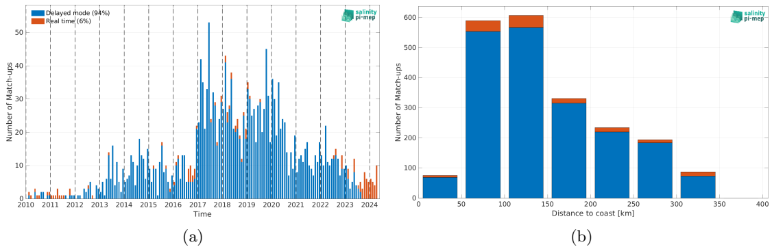
Figure 2: Number of match-ups between Argo and SMOS SSS L2Q v331 - No FLAG (CMEMS-CATDS-CPDC) SSS as a function of time (a) and as function of the distance to coast (b) over the Sea of Japan Pi-MEP region and for the full satellite product period.
