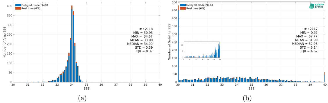
Figure 3: Histograms of SSS from Argo (a) and SMOS SSS L2Q v331 - No FLAG (CMEMS-CATDS-CPDC) (b) considering all match-up pairs per bins of 0.1 over the Sea of Japan Pi-MEP region and for the full satellite product period.
