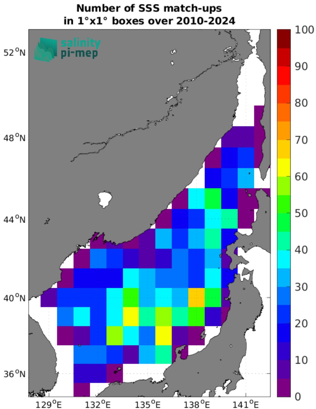
Figure 5: Number of SSS match-ups between Argo SSS and the SMOS SSS L2Q v331 - No FLAG (CMEMS-CATDS-CPDC) SSS product for the Sea of Japan Pi-MEP region over 1°x1° boxes and for the full satellite product period.
