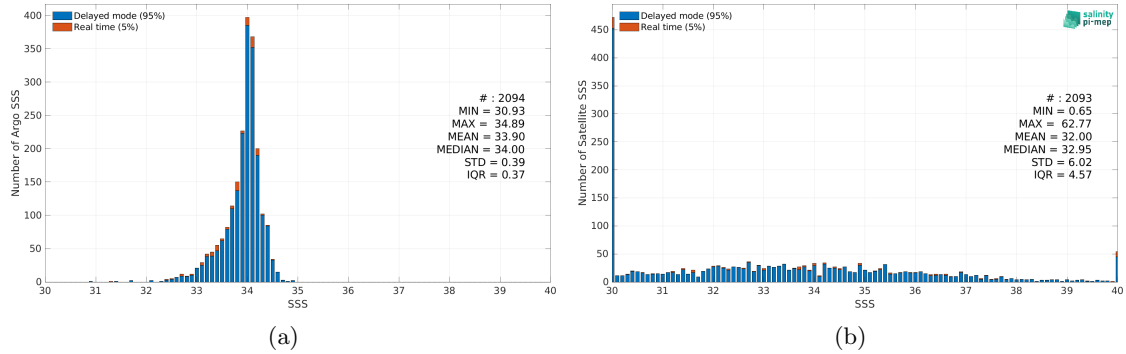
Figure 2: Histograms of SSS from Argo (a) and SMOS SSS L2Q v331 - No FLAG (CMEMS-CATDS-CPDC) (b) considering all match-up pairs per bins of 0.1 over the Sea of Japan Pi-MEP region and for the full satellite product period.
