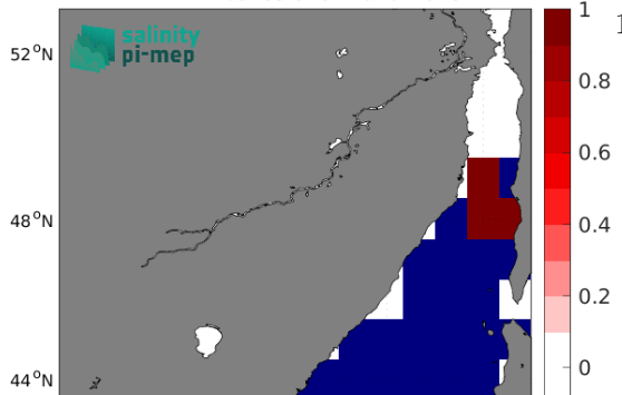
Temporal mean of (Sat - Argo) in 1°x1° boxes over 2010-2023
