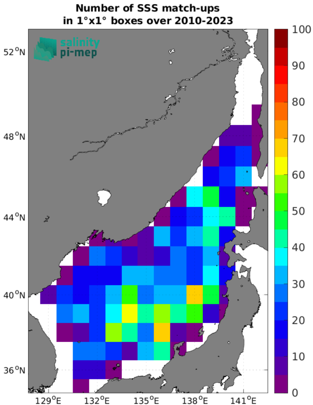
Figure 4: Number of SSS match-ups between Argo SSS and the SMOS SSS L2Q v331 - No FLAG (CMEMS-CATDS-CPDC) SSS product for the Sea of Japan Pi-MEP region over 1°x1° boxes and for the full satellite product period.
