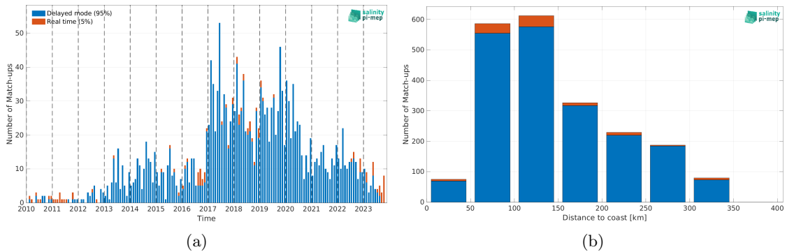
Figure 1: Number of match-ups between Argo and SMOS SSS L2Q v331 - No FLAG (CMEMS-CATDS-CPDC) SSS as a function of time (a) and as function of the distance to coast (b) over the Sea of Japan Pi-MEP region and for the full satellite product period.
