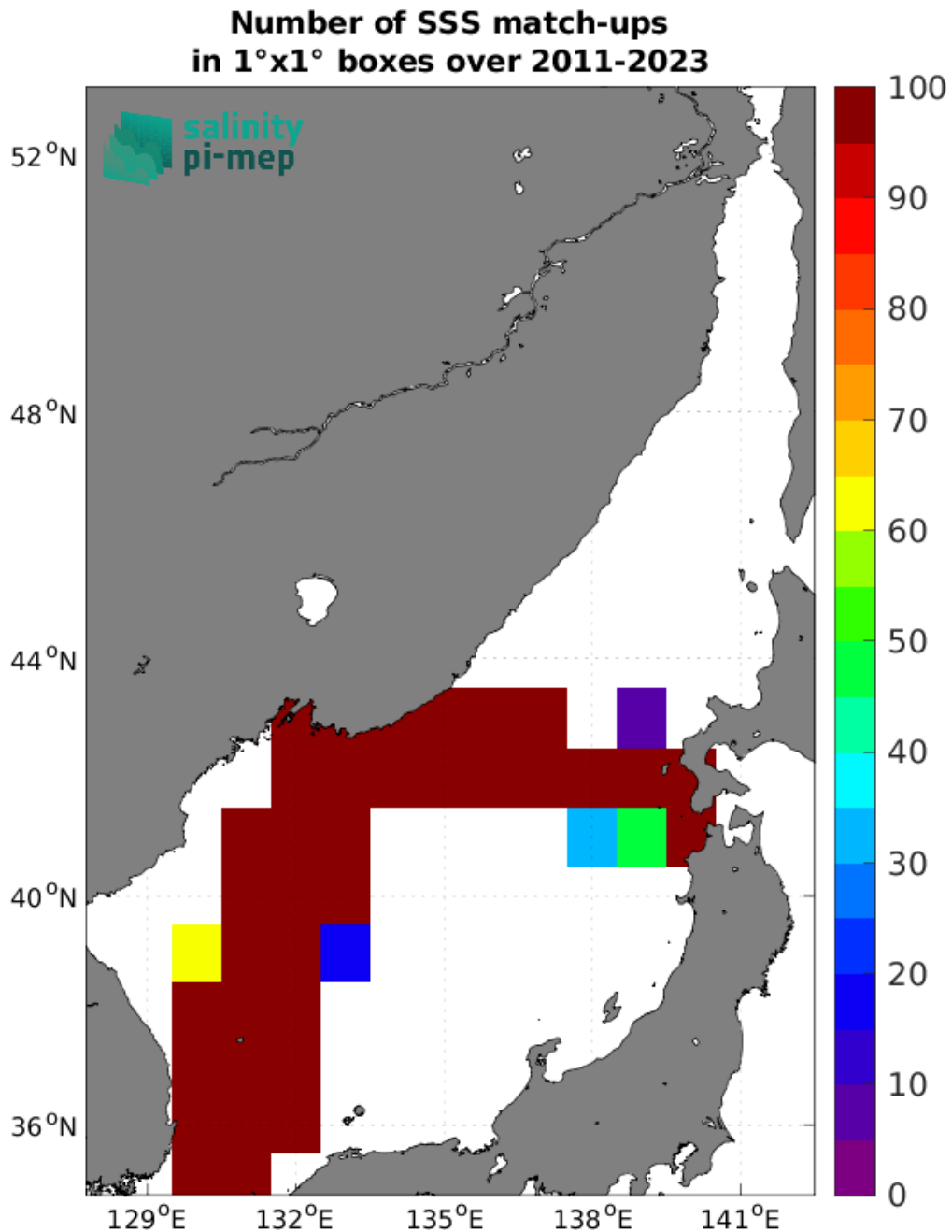
Figure 5: Number of SSS match-ups between TSG (LEGOS-DM) SSS and the SMOS SSS L3 v9 - 9 Days (CATDS-CEC-LOCEAN) SSS product for the Sea of Japan Pi-MEP region over 1°x1° boxes and for the full satellite product period.
