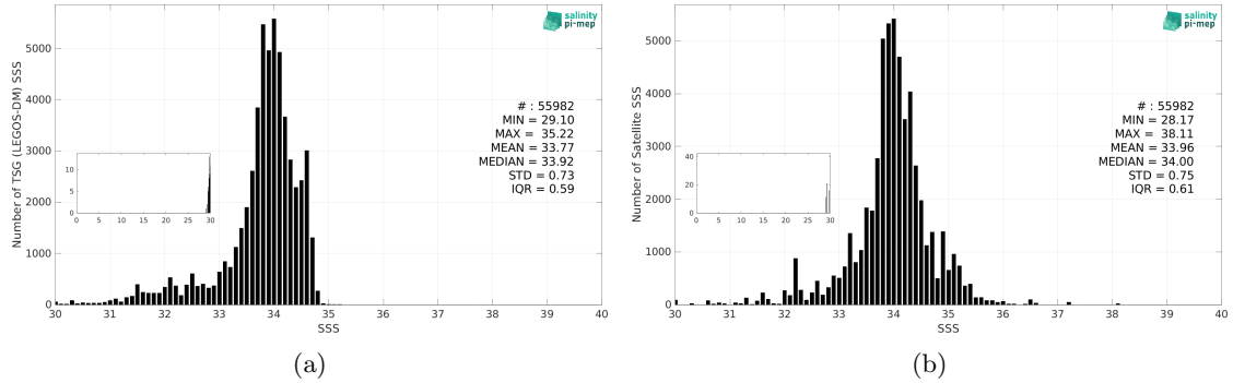
Figure 3: Histograms of SSS from TSG (LEGOS-DM) (a) and SMOS SSS L3 v9 - 9 Days (CATDS-CEC-LOCEAN) (b) considering all match-up pairs per bins of 0.1 over the Sea of Japan Pi-MEP region and for the full satellite product period.
