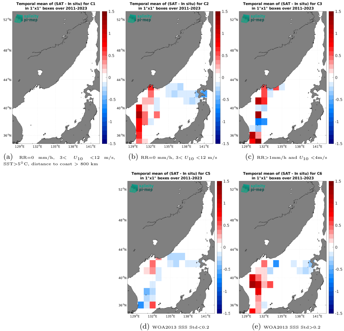
Figure 14: Temporal mean gridded over spatial boxes of size 1^\circ \times 1^\circ of \Delta\text{SSS} (SMOS SSS L3 v9 - 9 Days (CATDS-CEC-LOCEAN) - TSG (LEGOS-DM)) for 5 different subdatasets corresponding to: RR=0 mm/h, 3 < U_{10} < 12 m/s, SST > 5^\circ\text{C} , distance to coast > 800 km (a), RR=0 mm/h, 3 < U_{10} < 12 m/s (b), RR > 1 mm/h and U_{10} < 4 m/s (c), WOA2013 SSS Std < 0.2 (d), WOA2013 SSS Std > 0.2 (e).
