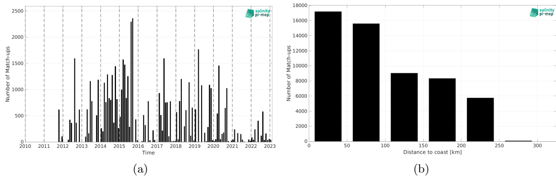
Figure 2: Number of match-ups between TSG (LEGOS-DM) and SMOS SSS L3 v9 - 9 Days (CATDS-CEC-LOCEAN) SSS as a function of time (a) and as function of the distance to coast (b) over the Sea of Japan Pi-MEP region and for the full satellite product period.
