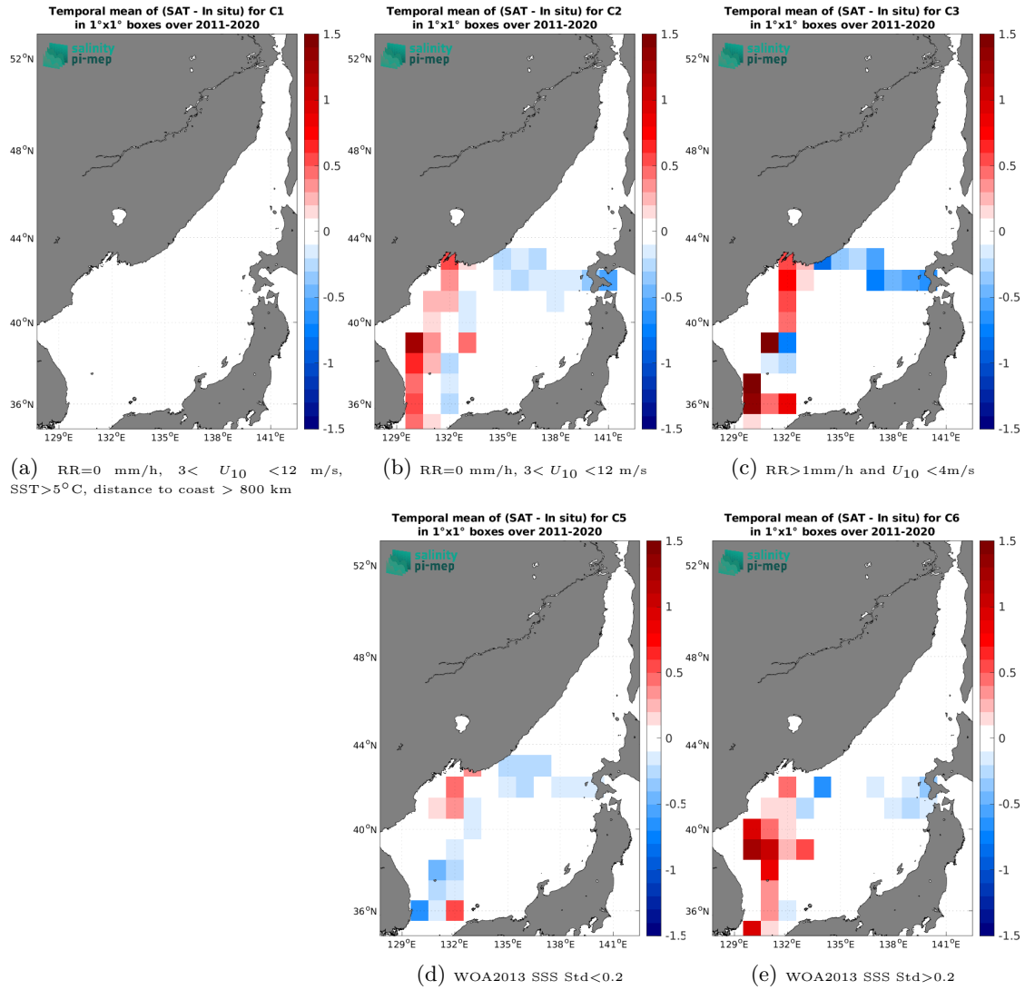
Figure 12: Temporal mean gridded over spatial boxes of size 1^\circ \times 1^\circ of \Delta SSS (SMOS SSS L3 v9 - 9 Days (CATDS-CEC-LOCEAN) - TSG (LEGOS-DM)) for 5 different subdatasets corresponding to:RR=0 mm/h, 3 < U_{10} < 12 m/s, SST>5°C, distance to coast > 800 km (a), RR=0 mm/h, 3 < U_{10} < 12 m/s (b), RR>1mm/h and U_{10} < 4 m/s (c), WOA2013 SSS Std<0.2 (d), WOA2013 SSS Std>0.2 (e).
