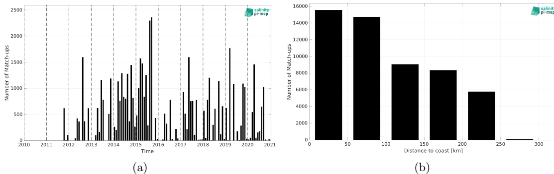
Figure 1: Number of match-ups between TSG (LEGOS-DM) and SMOS SSS L3 v9 - 9 Days (CATDS-CEC-LOCEAN) SSS as a function of time (a) and as function of the distance to coast (b) over the Sea of Japan Pi-MEP region and for the full satellite product period.
