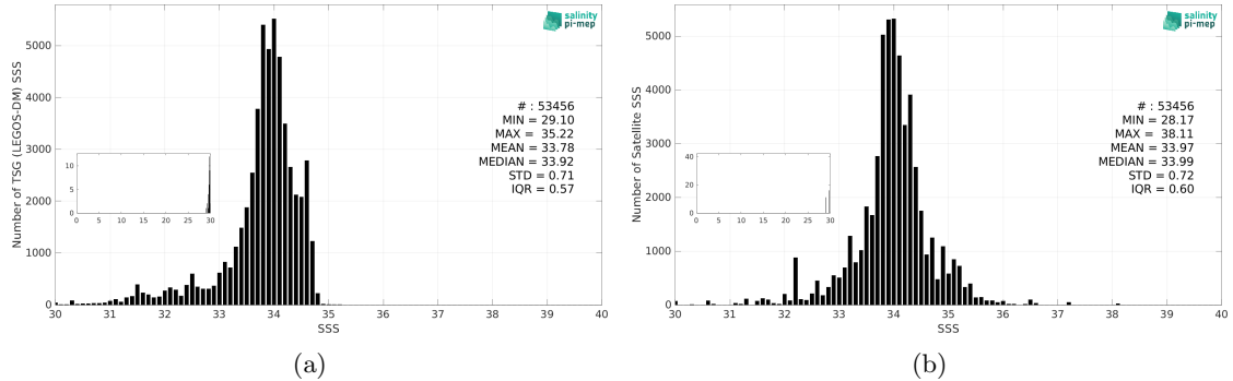
Figure 2: Histograms of SSS from TSG (LEGOS-DM) (a) and SMOS SSS L3 v9 - 9 Days (CATDS-CEC-LOCEAN) (b) considering all match-up pairs per bins of 0.1 over the Sea of Japan Pi-MEP region and for the full satellite product period.
