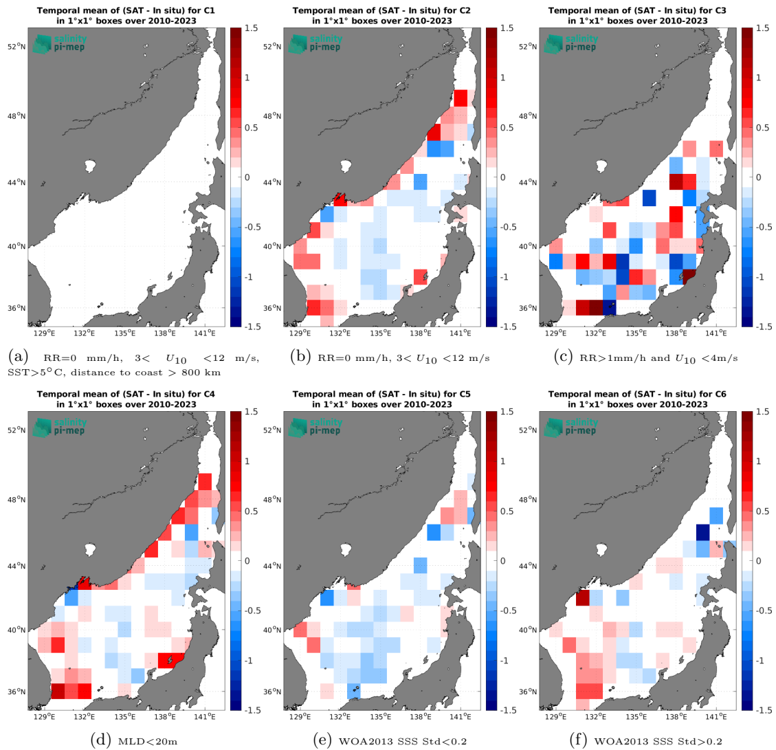
Figure 12: Temporal mean gridded over spatial boxes of size 1^\circ \times 1^\circ of \Delta SSS (SMOS SSS L3 v9 - 9 Days (CATDS-CEC-LOCEAN) - Argo) for 6 different subdatasets corresponding to: RR=0 mm/h, 3 < U_{10} < 12 m/s, SST > 5^\circ\text{C} , distance to coast > 800 km (a), RR=0 mm/h, 3 < U_{10} < 12 m/s (b), RR > 1 mm/h and U_{10} < 4 m/s (c), MLD < 20 m (d), WOA2013 SSS Std < 0.2 (e), WOA2013 SSS Std > 0.2 (f).
