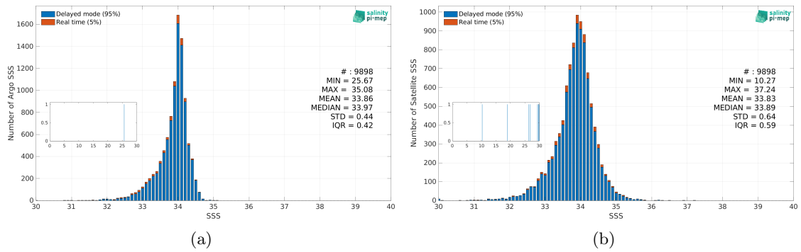
Figure 2: Histograms of SSS from Argo (a) and SMOS SSS L3 v9 - 9 Days (CATDS-CEC-LOCEAN) (b) considering all match-up pairs per bins of 0.1 over the Sea of Japan Pi-MEP region and for the full satellite product period.
