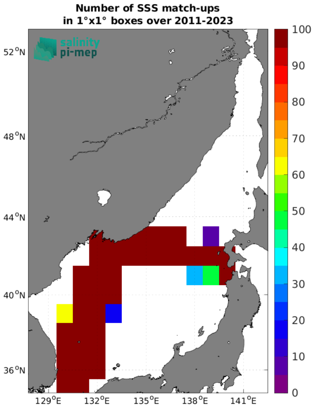
Figure 5: Number of SSS match-ups between TSG (LEGOS-DM) SSS and the SMOS SSS L3 v9 - 18 Days (CATDS-CEC-LOCEAN) SSS product for the Sea of Japan Pi-MEP region over 1°x1° boxes and for the full satellite product period.
