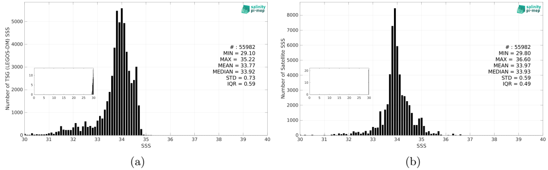
Figure 3: Histograms of SSS from TSG (LEGOS-DM) (a) and SMOS SSS L3 v9 - 18 Days (CATDS-CEC-LOCEAN) (b) considering all match-up pairs per bins of 0.1 over the Sea of Japan Pi-MEP region and for the full satellite product period.
