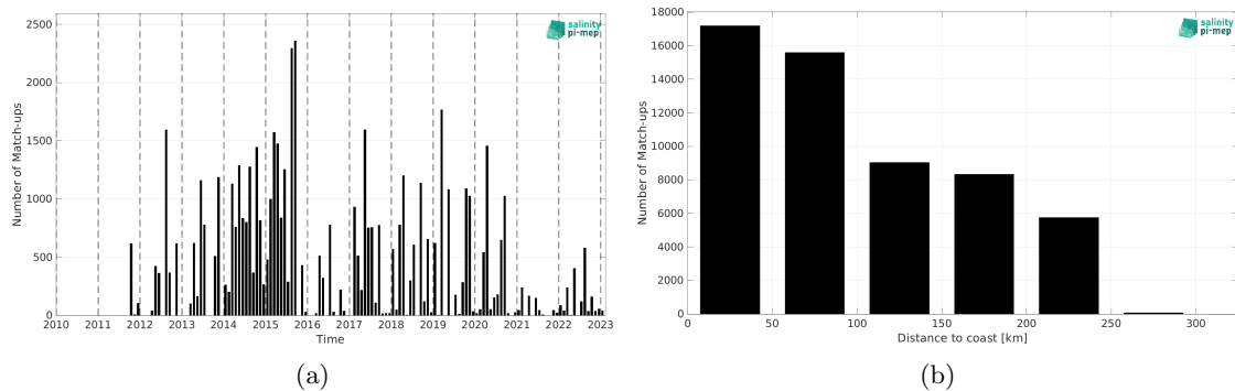
Figure 2: Number of match-ups between TSG (LEGOS-DM) and SMOS SSS L3 v9 - 18 Days (CATDS-CEC-LOCEAN) SSS as a function of time (a) and as function of the distance to coast (b) over the Sea of Japan Pi-MEP region and for the full satellite product period.
