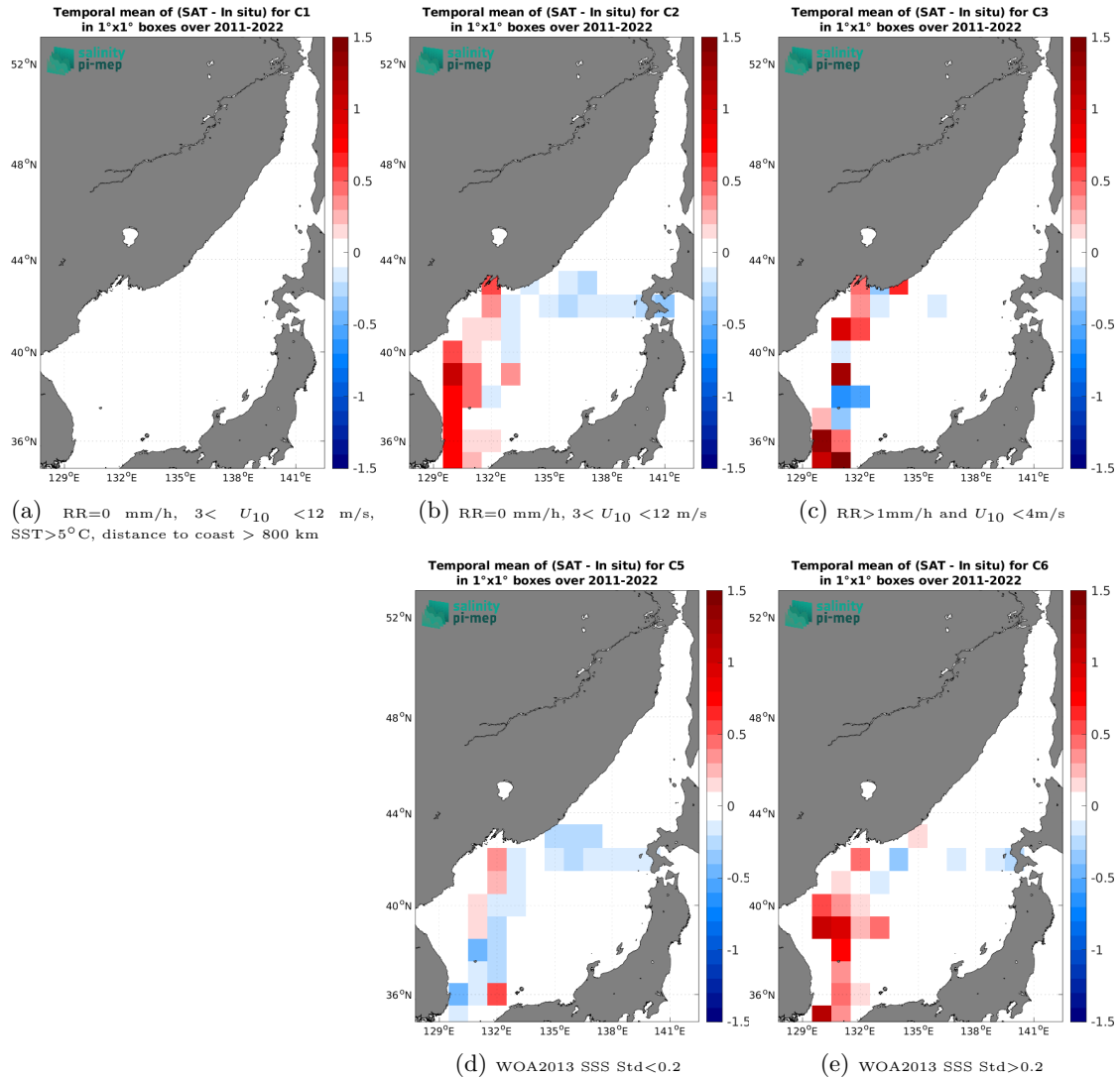
Figure 14: Temporal mean gridded over spatial boxes of size 1^\circ \times 1^\circ of \Delta\text{SSS} (SMOS SSS L3 v9 - 18 Days (CATDS-CEC-LOCEAN) - TSG (LEGOS-DM)) for 5 different subdatasets corresponding to: RR=0 mm/h, 3 < U_{10} < 12 m/s, SST > 5^\circ\text{C} , distance to coast > 800 km (a), RR=0 mm/h, 3 < U_{10} < 12 m/s (b), RR > 1 mm/h and U_{10} < 4 m/s (c), WOA2013 SSS Std < 0.2 (d), WOA2013 SSS Std > 0.2 (e).
