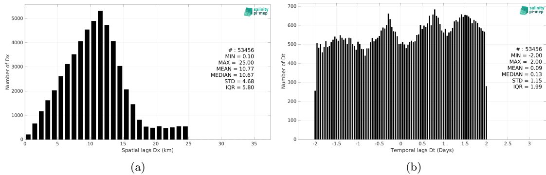
Figure 5: Histograms of the spatial (a) and temporal (b) lags between the location/time of the TSG (LEGOS-DM) measurement and the date of the corresponding SMOS SSS L3 v9 - 18 Days (CATDS-CEC-LOCEAN) SSS pixel.
