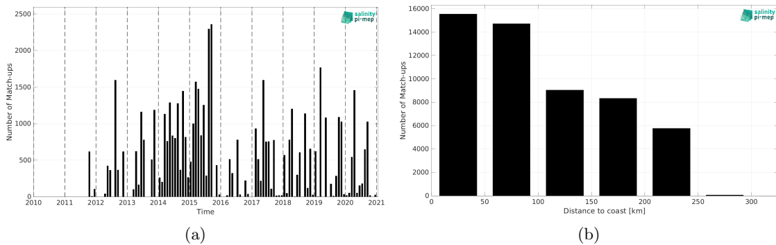
Figure 1: Number of match-ups between TSG (LEGOS-DM) and SMOS SSS L3 v9 - 18 Days (CATDS-CEC-LOCEAN) SSS as a function of time (a) and as function of the distance to coast (b) over the Sea of Japan Pi-MEP region and for the full satellite product period.
