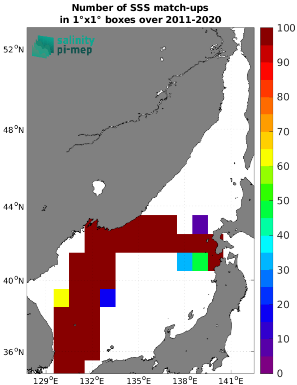
Figure 4: Number of SSS match-ups between TSG (LEGOS-DM) SSS and the SMOS SSS L3 v9 - 18 Days (CATDS-CEC-LOCEAN) SSS product for the Sea of Japan Pi-MEP region over 1°x1° boxes and for the full satellite product period.
