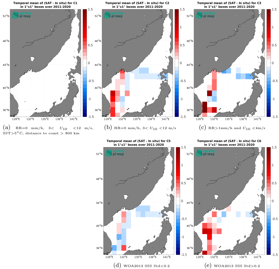
Figure 12: Temporal mean gridded over spatial boxes of size 1^\circ \times 1^\circ of \Delta SSS (SMOS SSS L3 v9 - 18 Days (CATDS-CEC-LOCEAN) - TSG (LEGOS-DM)) for 5 different subdatasets corresponding to:RR=0 mm/h, 3 < U_{10} < 12 m/s, SST>5°C, distance to coast > 800 km (a), RR=0 mm/h, 3 < U_{10} < 12 m/s (b), RR>1mm/h and U_{10} < 4 m/s (c), WOA2013 SSS Std<0.2 (d), WOA2013 SSS Std>0.2 (e).
