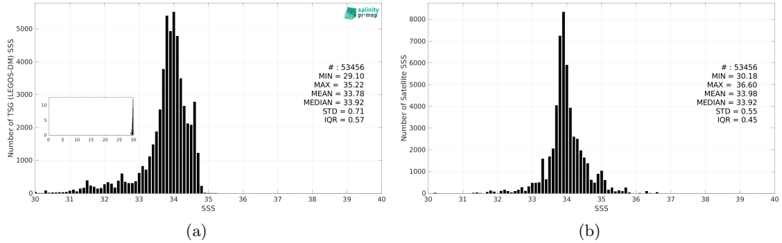
Figure 2: Histograms of SSS from TSG (LEGOS-DM) (a) and SMOS SSS L3 v9 - 18 Days (CATDS-CEC-LOCEAN) (b) considering all match-up pairs per bins of 0.1 over the Sea of Japan Pi-MEP region and for the full satellite product period.
