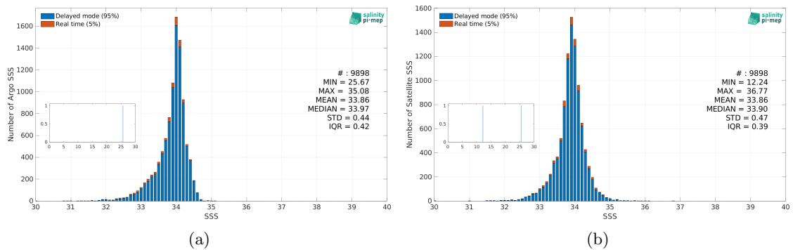
Figure 2: Histograms of SSS from Argo (a) and SMOS SSS L3 v9 - 18 Days (CATDS-CEC-LOCEAN) (b) considering all match-up pairs per bins of 0.1 over the Sea of Japan Pi-MEP region and for the full satellite product period.
