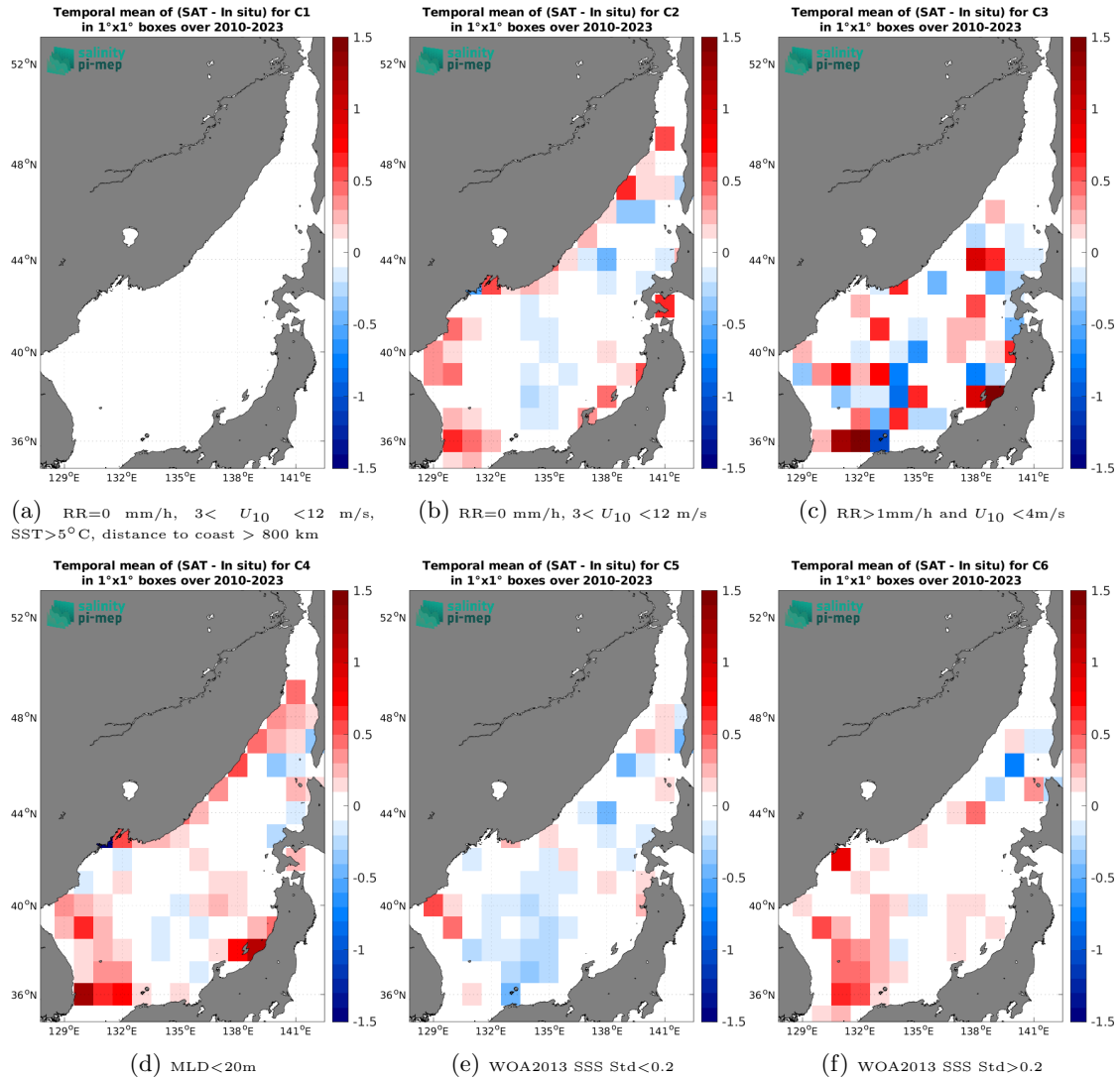
Figure 12: Temporal mean gridded over spatial boxes of size 1^\circ \times 1^\circ of \Delta SSS (SMOS SSS L3 v9 - 18 Days (CATDS-CEC-LOCEAN) - Argo) for 6 different subdatasets corresponding to: RR=0 mm/h, 3 < U_{10} < 12 m/s, SST > 5°C, distance to coast > 800 km (a), RR=0 mm/h, 3 < U_{10} < 12 m/s (b), RR > 1mm/h and U_{10} < 4 m/s (c), MLD < 20m (d), WOA2013 SSS Std < 0.2 (e), WOA2013 SSS Std > 0.2 (f).
