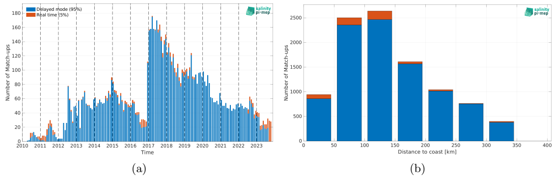
Figure 1: Number of match-ups between Argo and SMOS SSS L3 v9 - 18 Days (CATDS-CEC-LOCEAN) SSS as a function of time (a) and as function of the distance to coast (b) over the Sea of Japan Pi-MEP region and for the full satellite product period.
