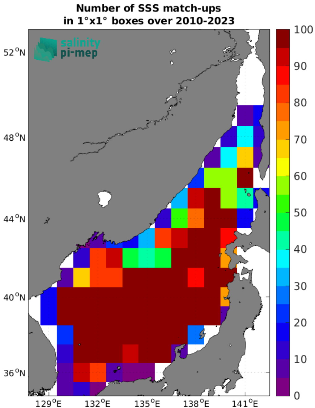
Figure 4: Number of SSS match-ups between Argo SSS and the SMOS SSS L3 v9 - 18 Days (CATDS-CEC-LOCEAN) SSS product for the Sea of Japan Pi-MEP region over 1°x1° boxes and for the full satellite product period.
