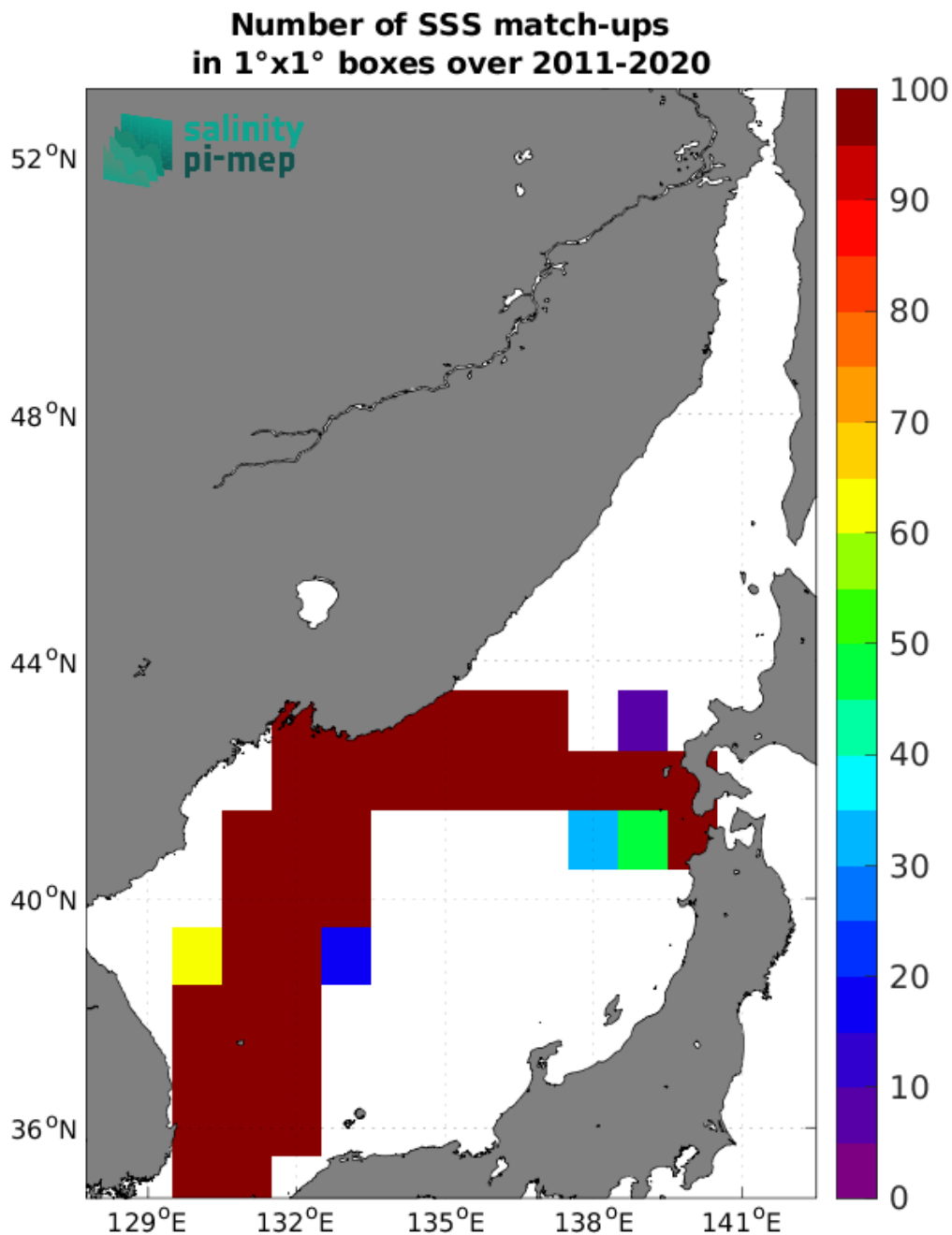
Figure 4: Number of SSS match-ups between TSG (LEGOS-DM) SSS and the SMOS SSS L3 v8 - 9 Days (CATDS-CEC-LOCEAN) SSS product for the Sea of Japan Pi-MEP region over 1°x1° boxes and for the full satellite product period.
