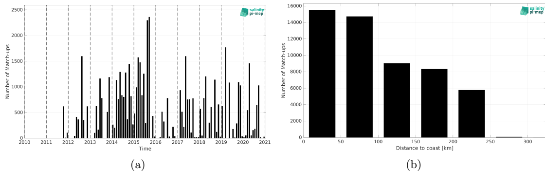
Figure 1: Number of match-ups between TSG (LEGOS-DM) and SMOS SSS L3 v8 - 9 Days (CATDS-CEC-LOCEAN) SSS as a function of time (a) and as function of the distance to coast (b) over the Sea of Japan Pi-MEP region and for the full satellite product period.
