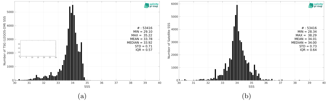
Figure 2: Histograms of SSS from TSG (LEGOS-DM) (a) and SMOS SSS L3 v8 - 9 Days (CATDS-CEC-LOCEAN) (b) considering all match-up pairs per bins of 0.1 over the Sea of Japan Pi-MEP region and for the full satellite product period.
