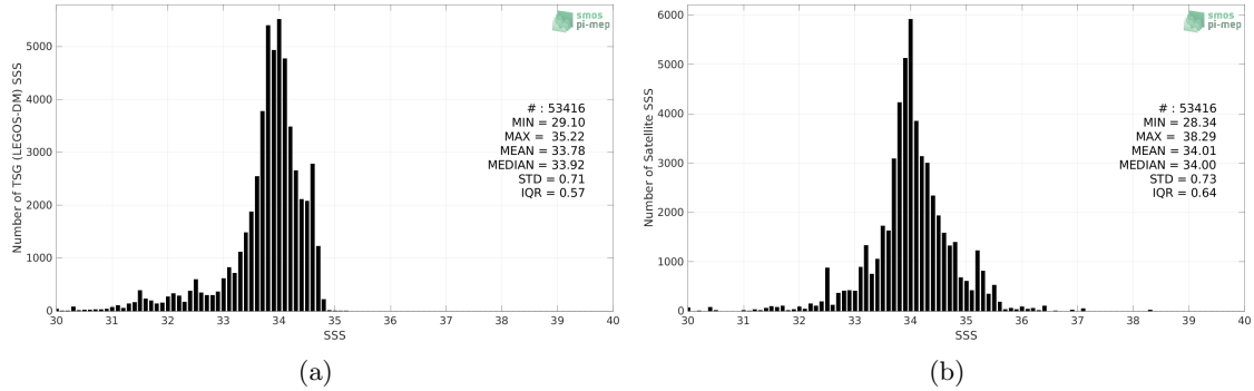
Figure 2: Histograms of SSS from TSG (LEGOS-DM) (a) and SMOS SSS L3 v8 - 9 Days (CATDS-CECOS-LOCEAN) (b) considering all match-up pairs per bins of 0.1 over the Sea of Japan Pi-MEP region and for the full satellite product period.
