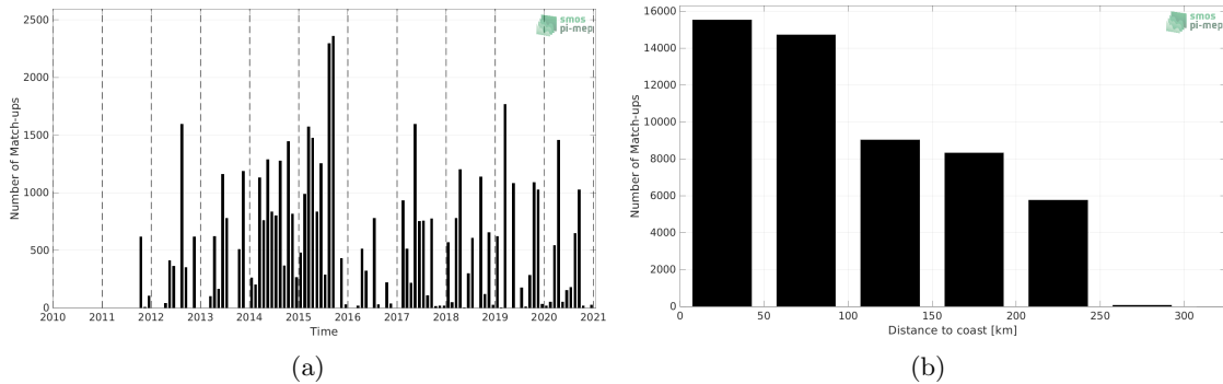
Figure 1: Number of match-ups between TSG (LEGOS-DM) and SMOS SSS L3 v8 - 9 Days (CATDS-CECOS-LOCEAN) SSS as a function of time (a) and as function of the distance to coast (b) over the Sea of Japan Pi-MEP region and for the full satellite product period.
