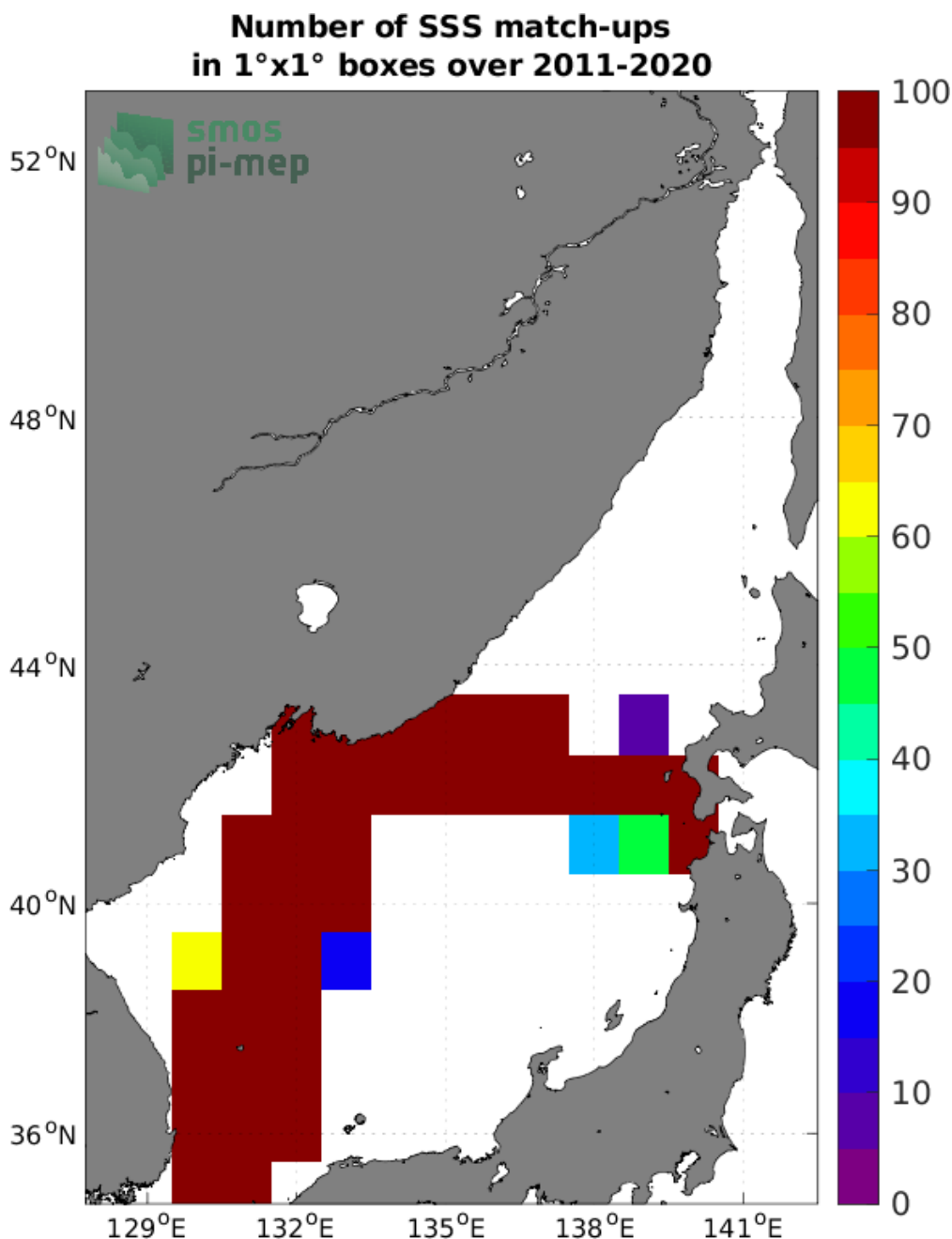
Figure 4: Number of SSS match-ups between TSG (LEGOS-DM) SSS and the SMOS SSS L3 v8 - 9 Days (CATDS-CECOS-LOCEAN) SSS product for the Sea of Japan Pi-MEP region over 1°x1° boxes and for the full satellite product period.
