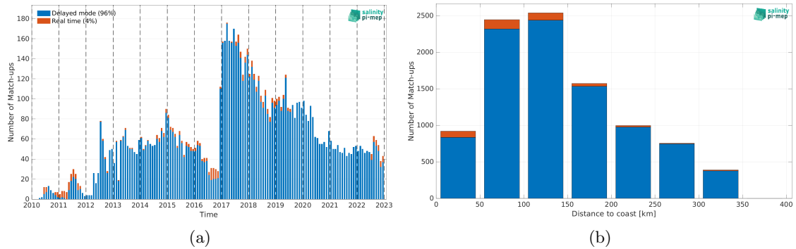
Figure 1: Number of match-ups between Argo and SMOS SSS L3 v8 - 9 Days (CATDS-CEC-LOCEAN) SSS as a function of time (a) and as function of the distance to coast (b) over the Sea of Japan Pi-MEP region and for the full satellite product period.
