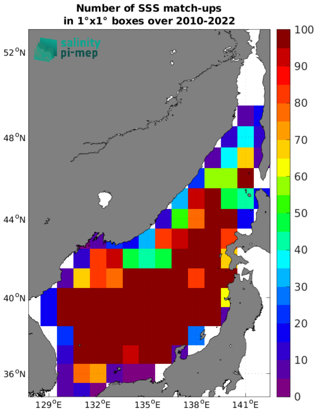
Figure 4: Number of SSS match-ups between Argo SSS and the SMOS SSS L3 v8 - 9 Days (CATDS-CEC-LOCEAN) SSS product for the Sea of Japan Pi-MEP region over 1°x1° boxes and for the full satellite product period.
