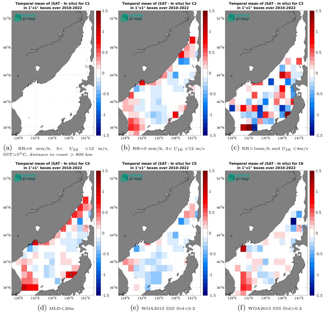
Figure 12: Temporal mean gridded over spatial boxes of size 1^\circ \times 1^\circ of \Delta\text{SSS} (SMOS SSS L3 v8 - 9 Days (CATDS-CEC-LOCEAN) - Argo) for 6 different subdatasets corresponding to: RR=0 mm/h, 3 < U_{10} < 12 m/s, SST > 5^\circ\text{C} , distance to coast > 800 km (a), RR=0 mm/h, 3 < U_{10} < 12 m/s (b), RR > 1\text{mm/h} and U_{10} < 4\text{m/s} (c), MLD < 20\text{m} (d), WOA2013 SSS Std < 0.2 (e), WOA2013 SSS Std > 0.2 (f).
